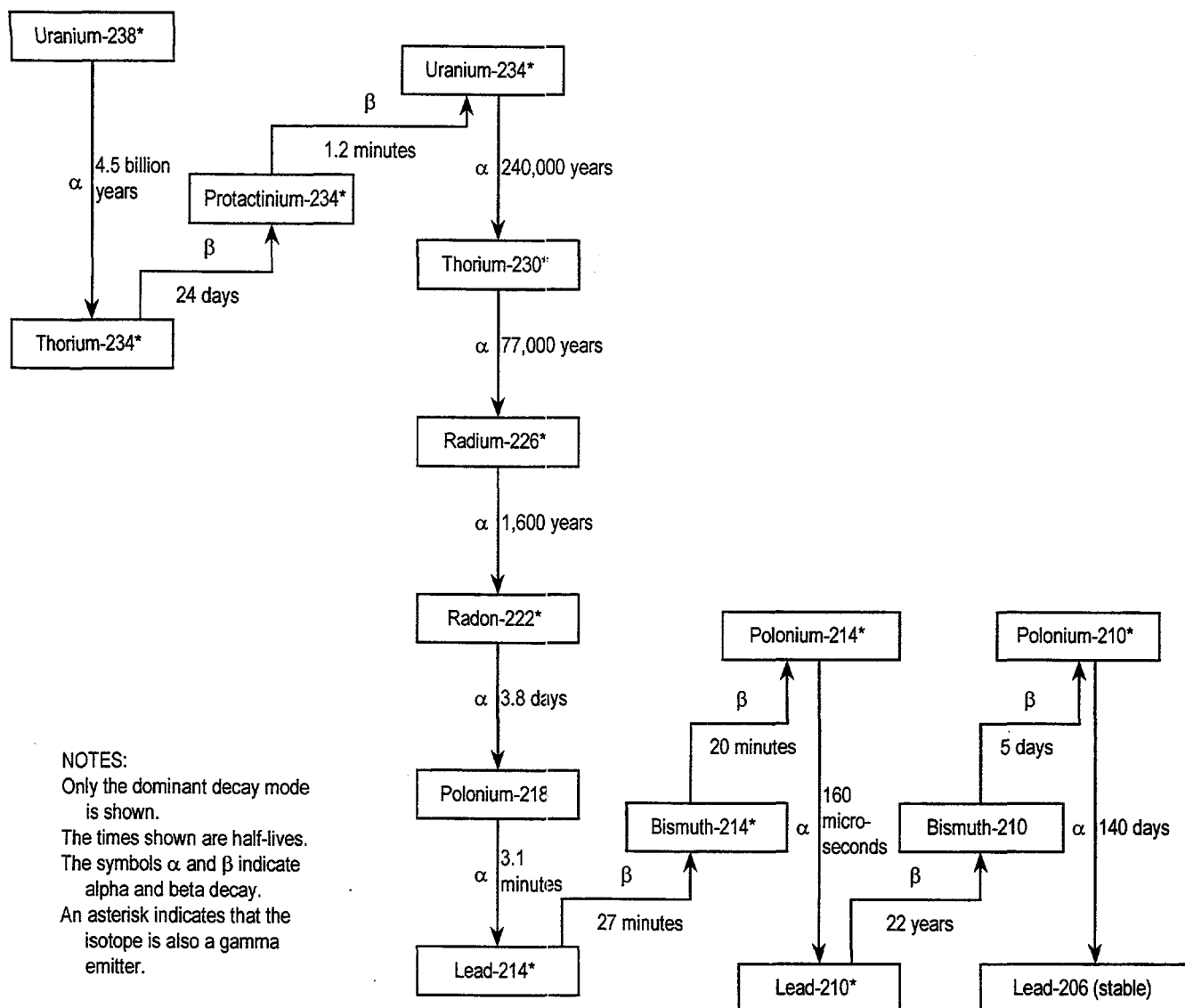
FIGURE 1 Uranium-238 Decay Series
