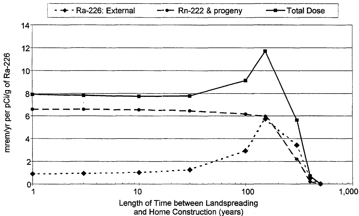
FIGURE 3 Potential Doses to a Resident of a Home with a Crawl Space Located over the Contaminated Zone
