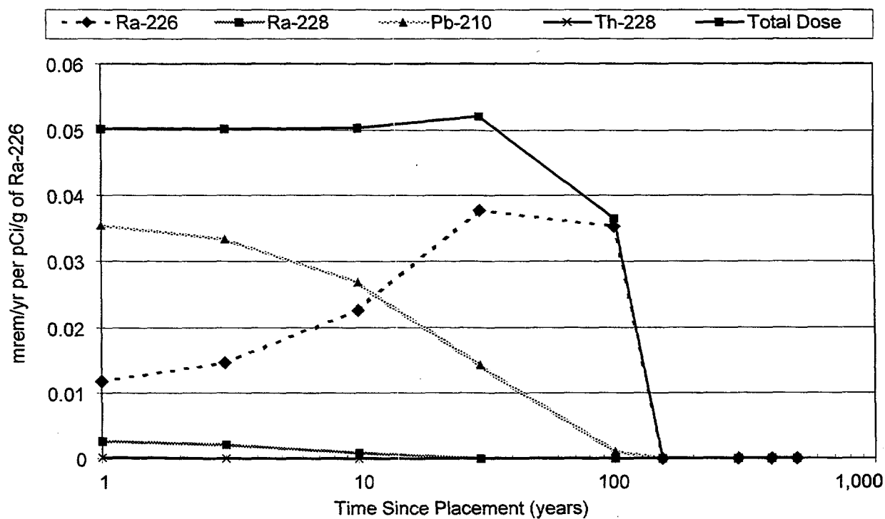
FIGURE 8 Potential Doses to an Individual from Ingestion of Contaminated Meat
