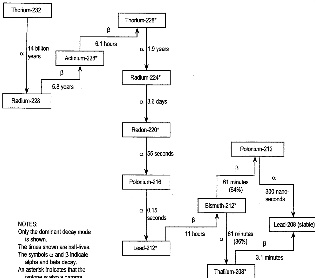
FIGURE 2 Thorium-232 Decay Series
