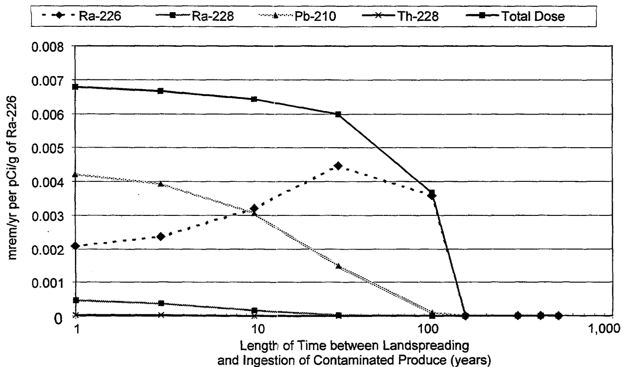
FIGURE 7 Potential Doses to an Individual from Ingestion of Contaminated Produce
