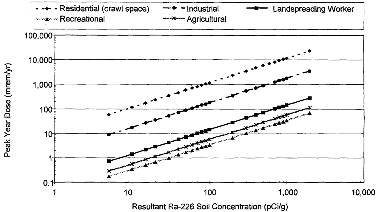
FIGURE 9 Correlation of Peak Year Dose to NORM Concentration
