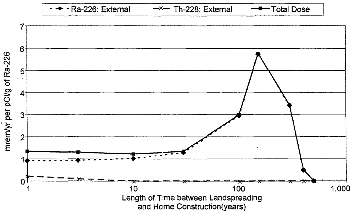
FIGURE 4 Potential Doses to a Resident of a Home with a Basement Excavated below the Contaminated Zone
