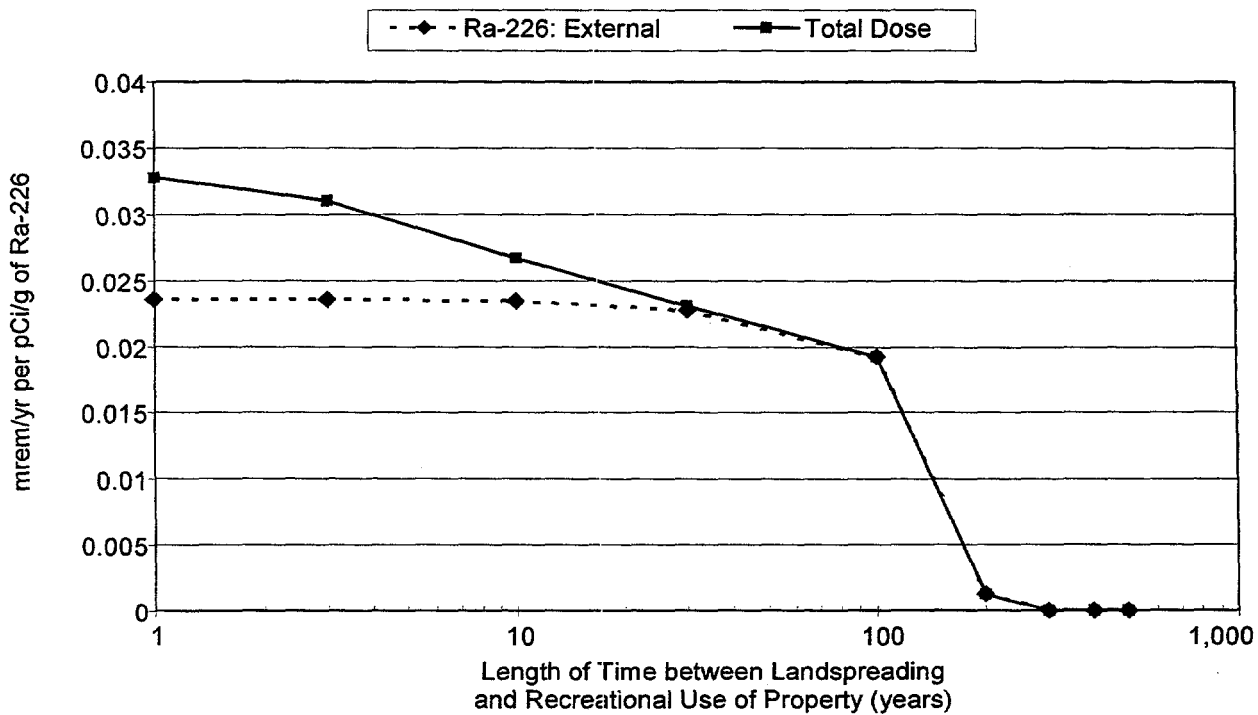
FIGURE 6 Potential Doses to a Member of the General Public Resulting from Occasional Recreational Use of the Property
