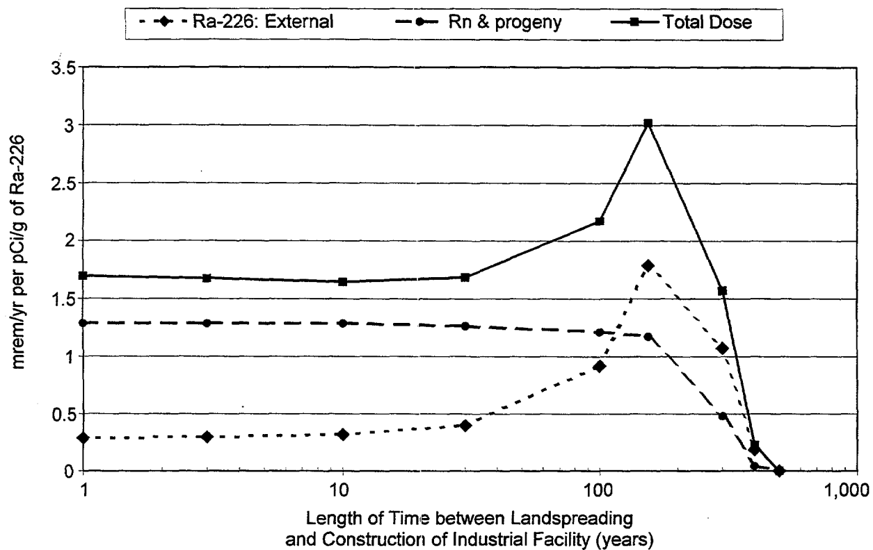
FIGURE 5 Potential Doses to an Industrial Worker
