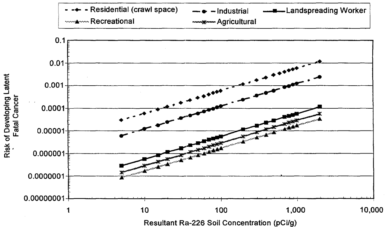
FIGURE 10 Correlation of Individual Risk of Developing Latent Fatal Cancer to NORM Concentration
