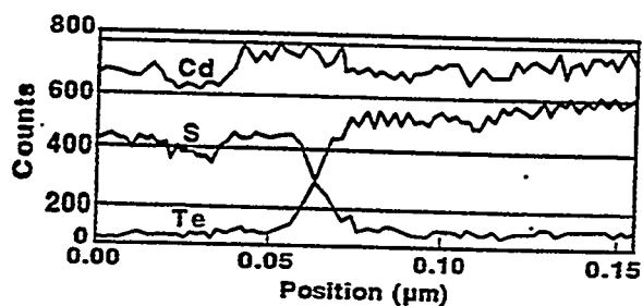
Figure 4: High resolution EDS elemental line-scans across the interface of a 425°C sample.
