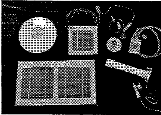
Fig. 1: Solar irradiance sensors, clockwise from upper left: Eppler PSP pyranometer, ESTI Sensor, LI-COR LI-200SA silicon-photodiode pyranometer, silicon reference cell, LI-COR LI-200SA with collimator, and AstroPower mini-module.
