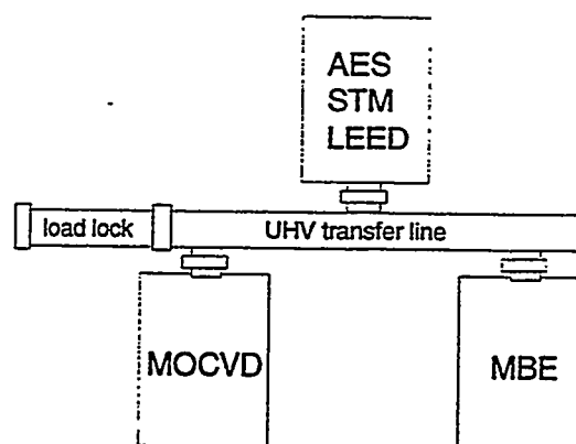
Figure 1. Schematic of MOCVD/MBE/Surface Analysis Cluster Tool.
