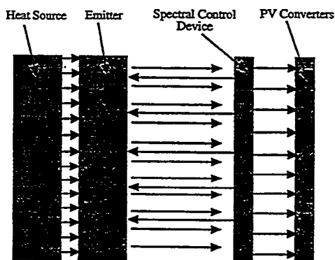
Figure 1: Block diagram illustrating key components of a TPV system.
