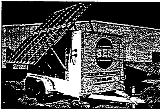
Figure 2: Solar Electric Specialties 1 kW Photogenaset, shown in the trailer-mounted configuration.
