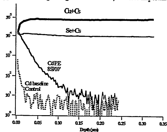
Fig. 5: SIMS profiles of Cd, Cu and Se in as-grown and Cd PE treated CuInSe 2 single crystals.
