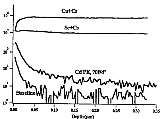
Fig. 4: SIMS profile of Cd, Cu and Se in CuInSe 2 thin films. Baseline refers to the as-grown film. The Cd PE treatment was done at 70°C for 4 min.
