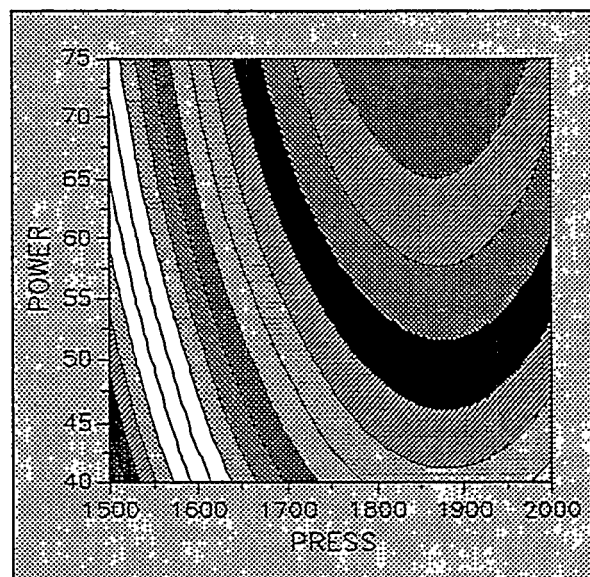
Figure 2. Contour plot showing response of J_{sc} to the power (W) and pressure (mT) during \text{NH}_3 -treatment with a protective-nitride thickness of 10 nm. J_{sc} ranges from 216 in the lower left corner to a minimum of 161 fA/cm 2 near the upper right corner. The duration of the \text{NH}_3 hydrogenation was 20 minutes.
