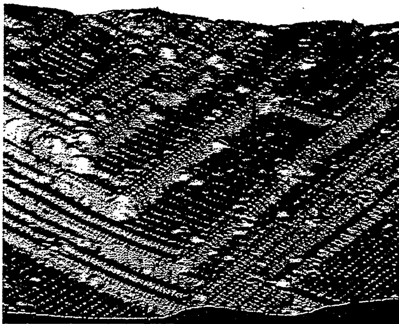
Figure 7. STM image of Ge(100)6'(110) annealed in AsH 3 at 640°C and an arsine partial pressure of 0.12 torr. Both 2x1 and 1x2 terraces are present. Individual terrace dimers and individual facet atoms are clearly visible. Microfacets show clear evidence of reconstruction.
