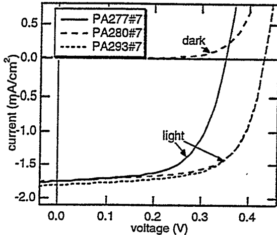
Figure 3. Measured IV curves at \sim 1 sun AM1.5 Direct illumination for several of the prototype devices of Fig. 2. The devices were covered by a GaAs filter and the currents were calibrated as described in the text. The corresponding dark IV curve for PA280#7 is shown also.
