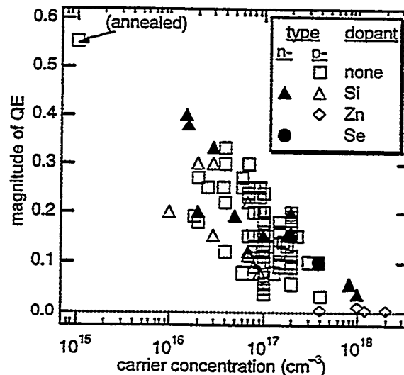
Figure 5. The QE of a variety of GaInNAs epilayers at 200-meV above the band edge, as a function of carrier concentration. All data shown are from layers with band gaps E_g < 1.15 eV.
