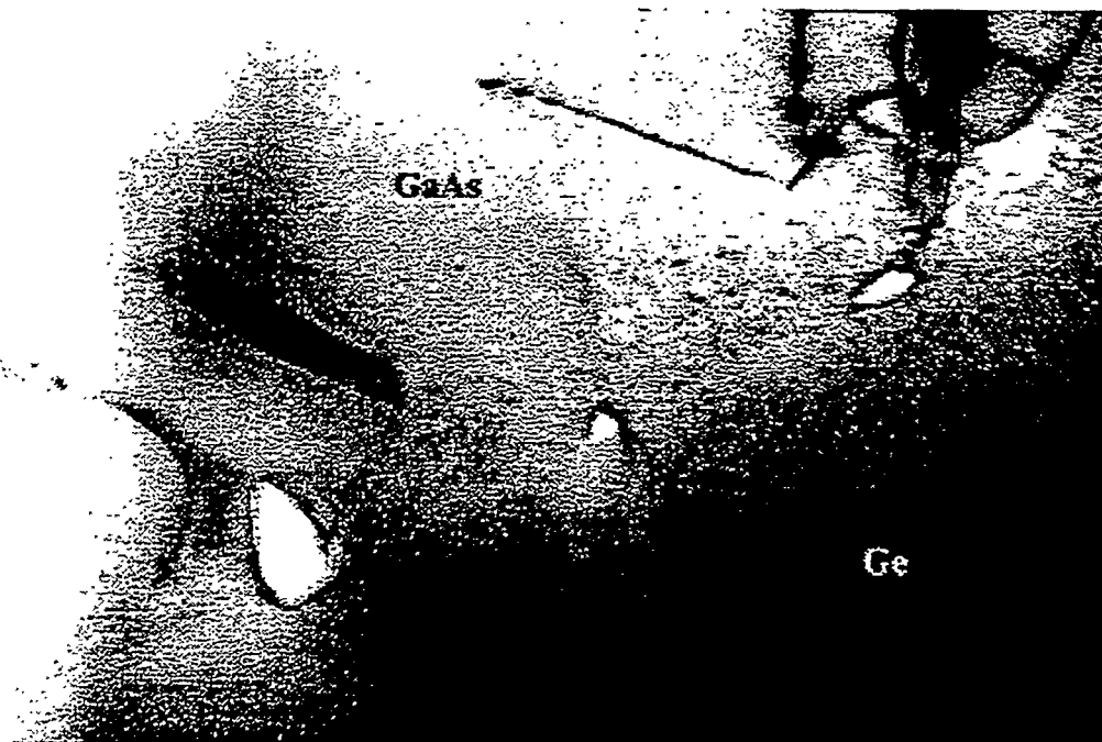
Figure 8. TEM micrograph showing antiphase domains (small truncated triangles) at the GaAs/Ge interface. The Ge(100)6'(111) substrate was annealed in AsH 3 under conditions similar to those used in Fig. 5.
