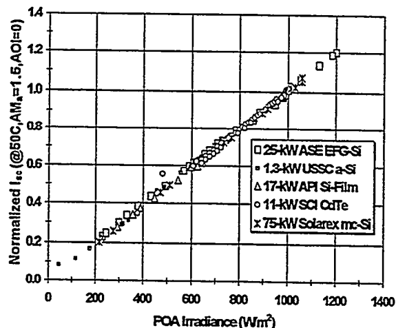
Fig. 3: Normalized I_{sc} versus solar irradiance for five PV arrays of different technologies, new performance model.
