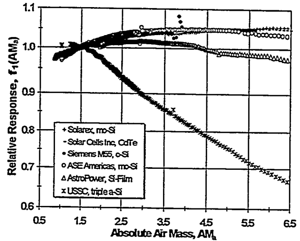
Fig. 1: Measured effect of solar spectral variation ( AM_a ) on the relative response (short-circuit current) of different commercial modules, for clear sky conditions.
