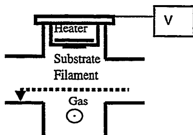
Figure 1a: The HWCVD cross reactor
