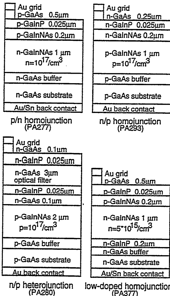
Figure 2. Schematics of the structures of the 1-eV cells (not to scale). The growth run identification numbers are shown in parentheses at the bottom of the figure. For each growth run, several devices were fabricated on the wafer, and are designated, for example, as PA280#7 in the tables and figures below.
