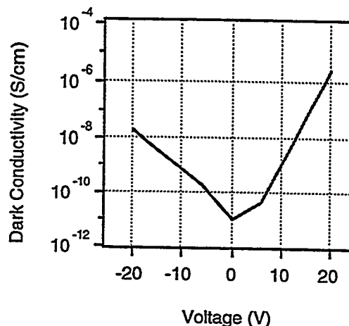
Figure 4: The effect of bias on the a-Si:H film quality. The represents the value of many sample data.
