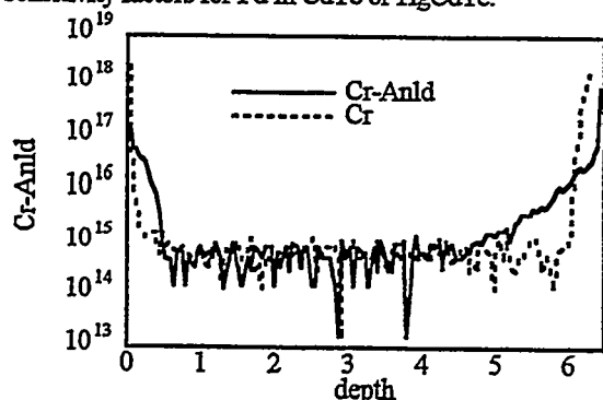
Figure 4: SIMS profile of Cr concentration in sample before and after annealing.
