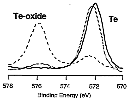
Figure 6: XPS spectra of Te, showing the presence of Te oxide(s) at the surface (dashed line), and its diminution deeper in the material: at 4 nm (dotted line) and at 13 nm (solid line).
