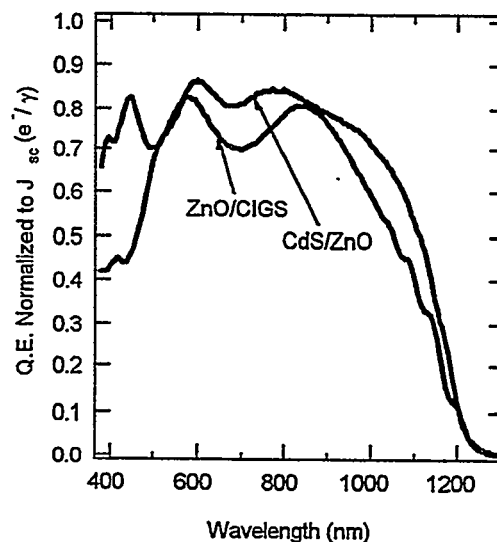
Fig. 7: Spectral response curves for CIGS devices with and without CdS.
