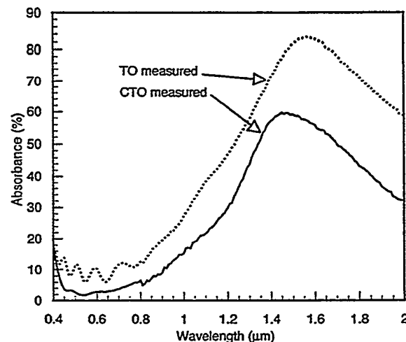
Figure 4: Measured free-carrier absorbance of films of tin oxide and CTO.
