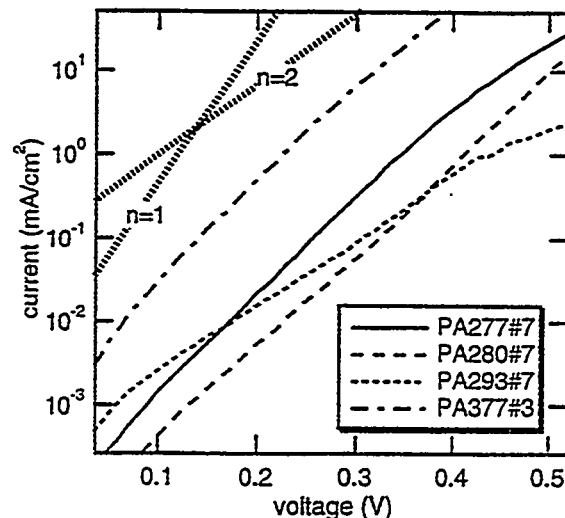
Figure 7. Dark IV curves for the various devices of Fig. 2. The slopes corresponding to ideality factors n=1 and 2 are indicated by the thick dotted lines labeled " n=1 " and " n=2 ".
