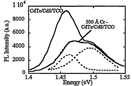
Figure 2: Junction PL spectra for non-metallized and 500 Å Cr sample illustrating the nature of the changes induced in the spectra by metallization.
