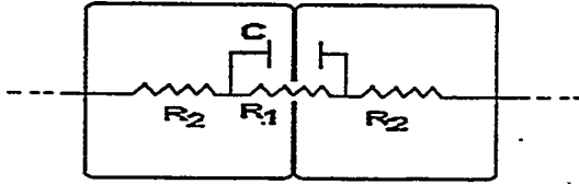
Figure 1: Grain-Boundary Electrical Model with intragrain resistance, R_2 , in series with a grain-boundary impedance, R_1 in parallel with C. Typically, R_1 \gg R_2 .
