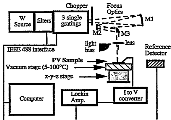
Figure 2: NREL grating monochrometer QE system
