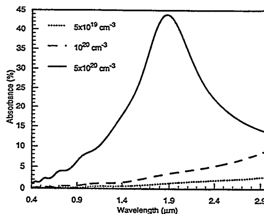
Figure 1: Modeled variation of the free-carrier absorbance of TCO films, the carrier concentration being treated parametrically.
