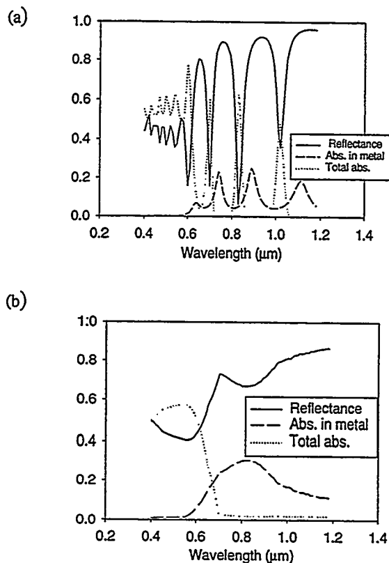
Figure 5: Calculated characteristics of a a-Si solar cell (see text for the cell structure) using PV Optics in (a) coherent mode and (b) noncoherent mode.
