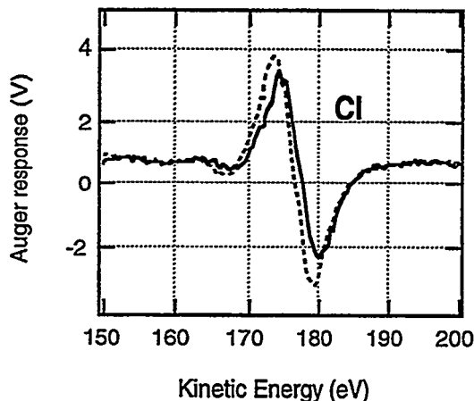
Figure 2: AES spectra of chlorine before (dashed line) and after (solid line) a 45-min anneal at 10^{-8} torr.
