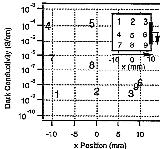
Figure 2: The mapping of dark conductivity of a-Si:H on glass substrate at 220°C substrate temperature. Inserted figure is the glass substrate and the numbers indicate the positions on the film that conductivity be measured. The dark strip on the side is grounded metal clips to hold substrate.
