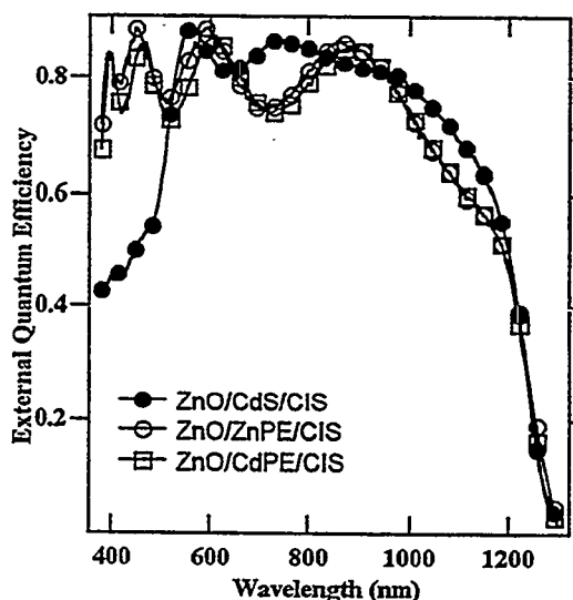
Fig. 2: Spectral response of the \text{CuInSe}_2 devices shown in Fig. 1. Measured before AR coating.
