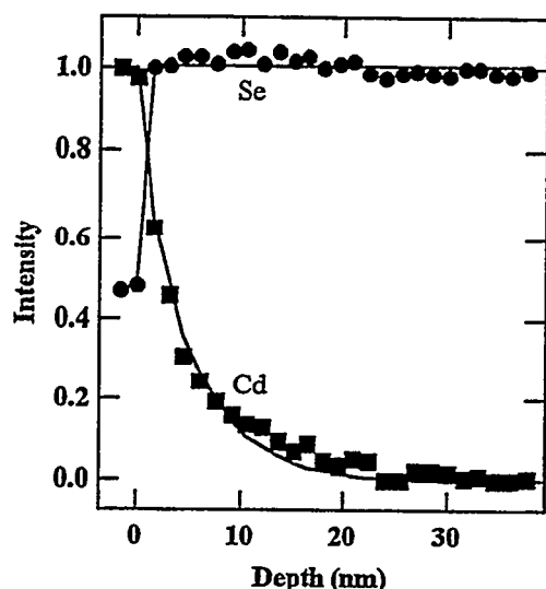
Fig. 3: XPS profile of Cd after Cd PE treatment. The absorber is CuInGaSe 2 thin film.
