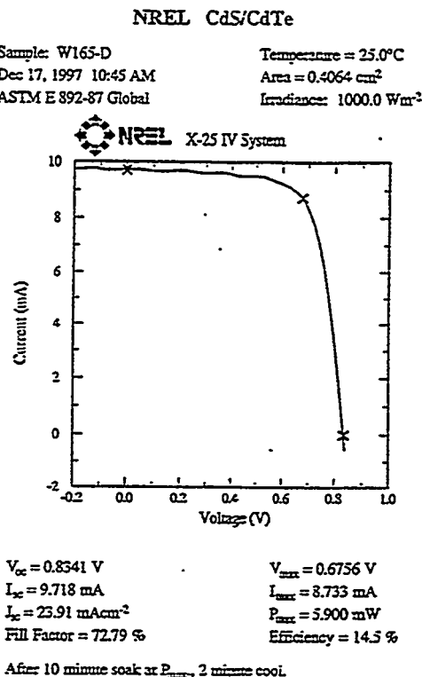
Figure 6: Current/voltage characteristic of a CdS/CdTe device using a CTO top contact. CdS/CdTe solar cell with a CTO back-contact.
