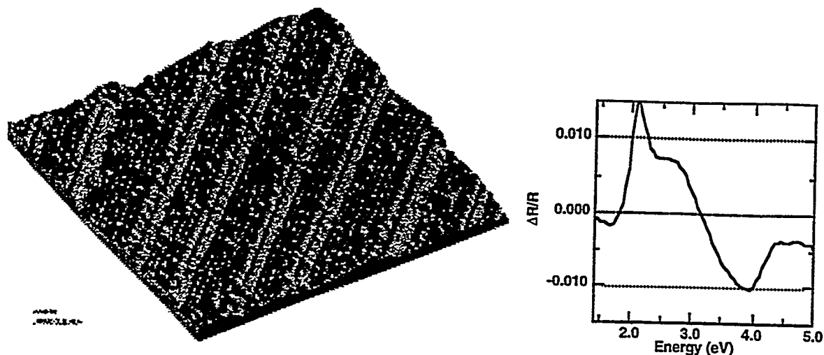
Figure 4. (a) STM image of As:Ge(100)6'(111). Dimer rows run parallel to step edges. (b) RD spectrum at room temperature for this surface.
