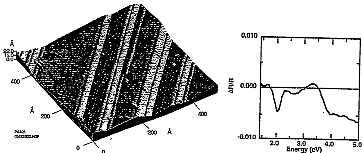
Figure 5. (a) STM image of a Ge(100)6'(111) surface annealed in AsH 3 at 640°C for 15 min. Surface is two-domain with dimer rows both parallel and perpendicular to the step edges. Steps are bunching to form facets. Step bunching process is facilitated by a slow AsH 3 etching of the Ge.
