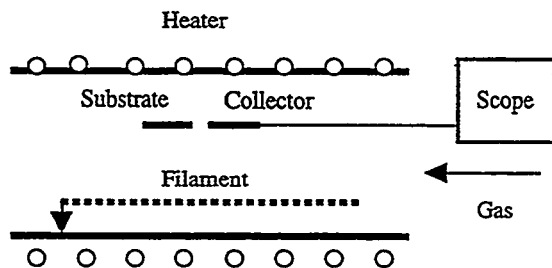
Figure 1b: The HWCVD tube reactor. Tube is side the vacuum chamber which is not shown.
