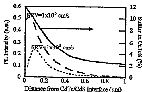
Figure 5: Spatial distribution of recombination vs. sulfur alloy composition in CdTe layer. Dashed lines show recombination for two different values of SRV.
