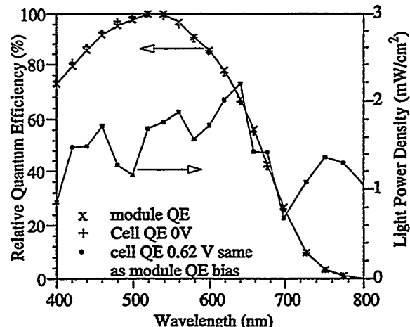
Figure 3: Module vs. cell QE measured with the filter system on a Solarex SA5 module.
