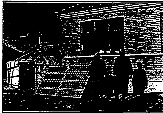
Figure 2. 500-Watt PV/wind hybrid household system in Inner Mongolia. Courtesy of Wang Sicheng, JiKe Company.
