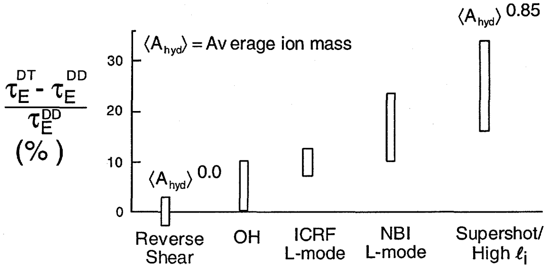
Fig.3. Comparison of the percentage increase in confinement time in comparable D and D-T plasmas, for the confinement time in reverse shear, ICRF, OH L-mode, supershots and high l_i regimes. The results are shown for an average mass of the hydrogenic ion of 2.5.
