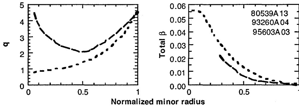
Fig. 2. Experiments in 1995-96 have explored three high-confinement regimes. The solid curves are for supershots with \beta_{nmax} \leq 2 which resulted in 10.7MW of fusion power. The short dashed curves are for high l_i discharges with \beta_{nmax} \geq 2.3 and P_{DT} = 8.7 MW and the long dashed curves are for an enhanced reversed shear discharge with \beta_{nmax} < 2.0 .
