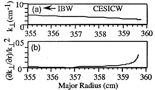
Fig. 2. CESICW \Rightarrow IBW launching case. f = 51 MHz, B_{TF} = 4.5 T (at R=275\text{cm} ) (a) k_{\perp} ( \text{cm}^{-1} ), and (b) WKB parameters.
