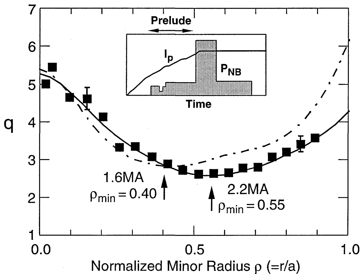
Fig. 1 q -profiles calculated for 2.2 MA (solid) and 1.6 MA (dashed) reversed shear plasmas at the end of the neutral beam prelude. The solid points are the motional Stark-effect (MSE) data for the 2.2 MA plasmas. Conditions: R_p = 2.60 m, a = 0.95 m, B_T = 4.6 T. Schematic waveforms of the plasma current and neutral beam power are shown in the inset.
