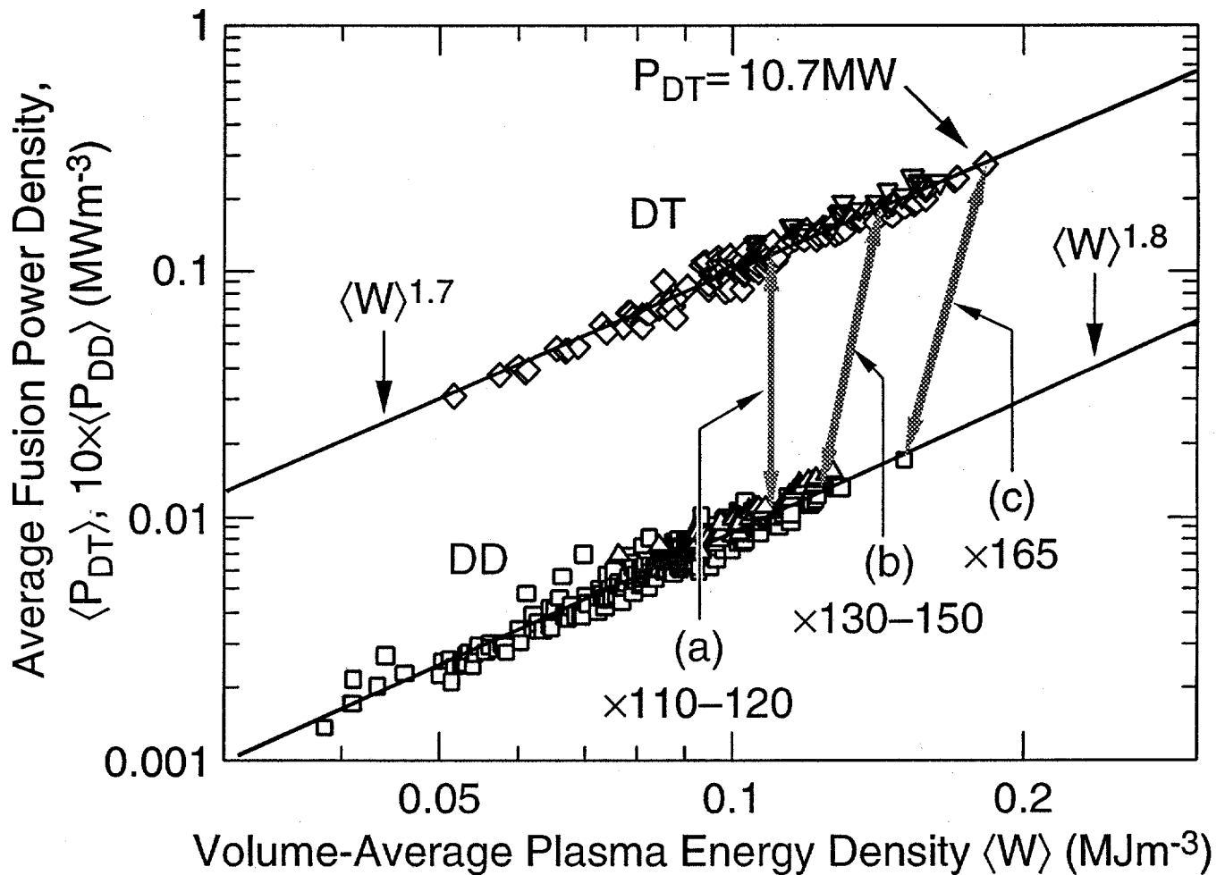
Fig. 7 In NBI-heated supershots and high- I_p plasmas, there is a close relationship between the volume-average plasma energy density ( \langle W \rangle \propto \beta B^2 ) and the volume-average fusion power density for both DD ( \propto \langle W \rangle^{1.8} ) and DT ( \propto \langle W \rangle^{1.7} ) reactions. The data above is for plasmas with I_p \geq 2\text{MA} and volumes 31 - 46\text{ m}^3 . The DT plasmas are restricted to those with nearly optimal D-T mixture. The arrowed lines indicate the reactivity ratio achievable under various constraints: (a) for constant \beta ; (b) for constant NBI power, taking advantage of the isotope effect on global confinement; (c) at maximum supershot performance, taking advantage of the higher NBI power available with tritium NBI.
