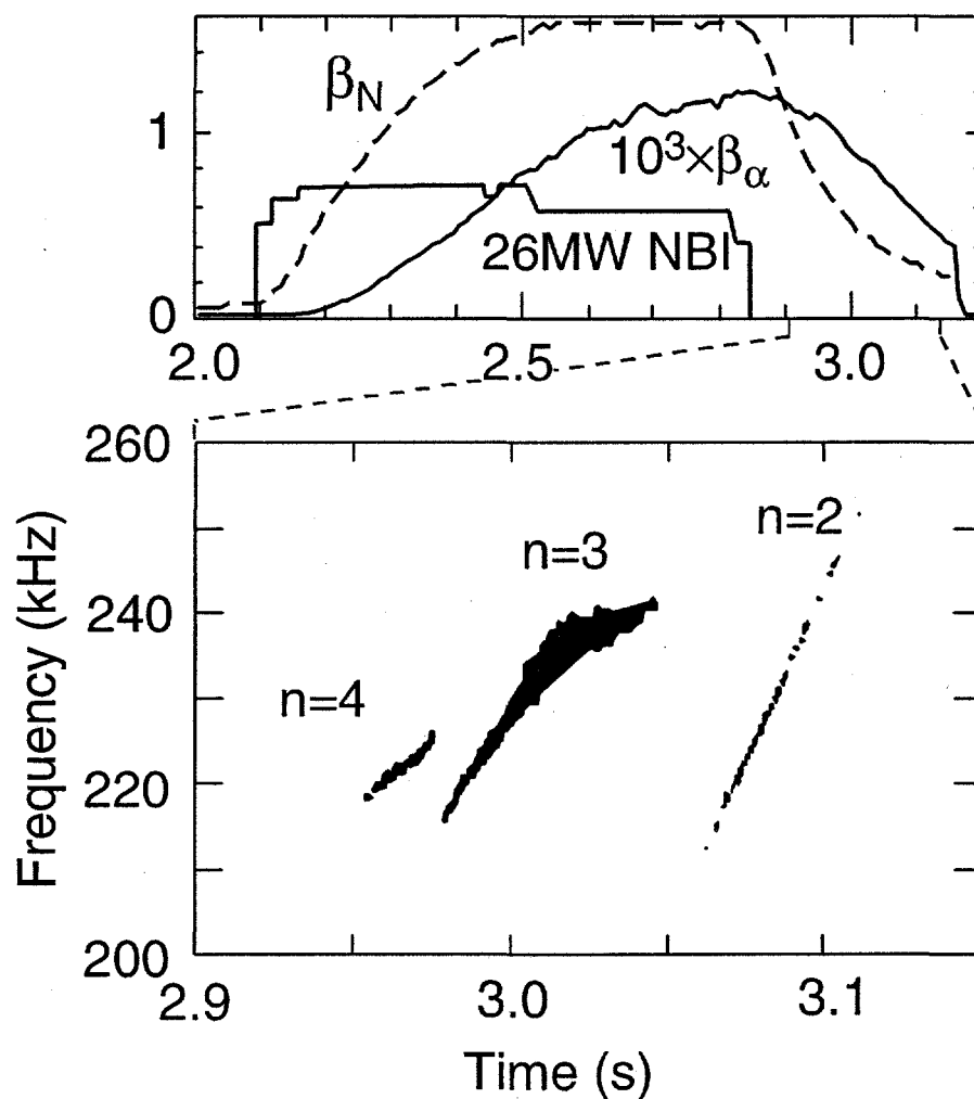
Fig. 8 Observation of a core-localized TAE driven by fusion alpha-particles in a plasma with weak magnetic shear and q_0 > 1 . a) NBI heating power, normalized \beta and \beta_\alpha . b) Frequency spectrum of Mirnov fluctuations in the TAE range of frequencies. Three modes are successively excited in the period following NBI. The n=3 mode was also observed on a core channel of the microwave reflectometer.
