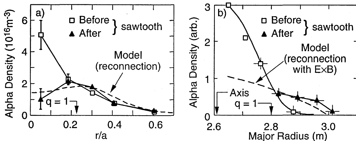
Fig. 9 Radial profiles of confined alphas near the center of TFTR as measured by a) the Alpha-CHERS system measuring predominantly passing alphas in the energy range 0.15 – 0.6 MeV and b) the pellet charge-exchange (PCX) diagnostic measuring deeply trapped alphas at an energy of 1.2 MeV. The sawtooth crash causes a significant redistribution of the alphas from inside to outside the q = 1 radius. The dashed lines indicate calculations of the profiles after the crash based on models of the reconnection. Plasma conditions: I_p = 2.0 \text{MA} , B_T = 5.1 \text{T} , R_p = 2.52 \text{m} , a = 0.87 \text{m}
