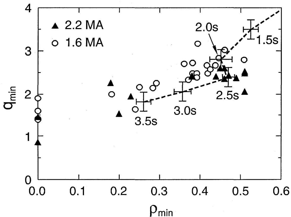
Fig. 2 Values of \rho_{\min} and q_{\min} at the start of the high-power NBI phase for 1.6MA (open circles) and 2.2MA (solid triangles) plasmas with varying startup conditions. Plasmas with \rho_{\min} > 0 have reversed shear. Also shown is the trajectory in time followed by one 2.2MA plasma. The radial error bars indicate the variability of \rho_{\min} within a 0.1s window about each time point.
