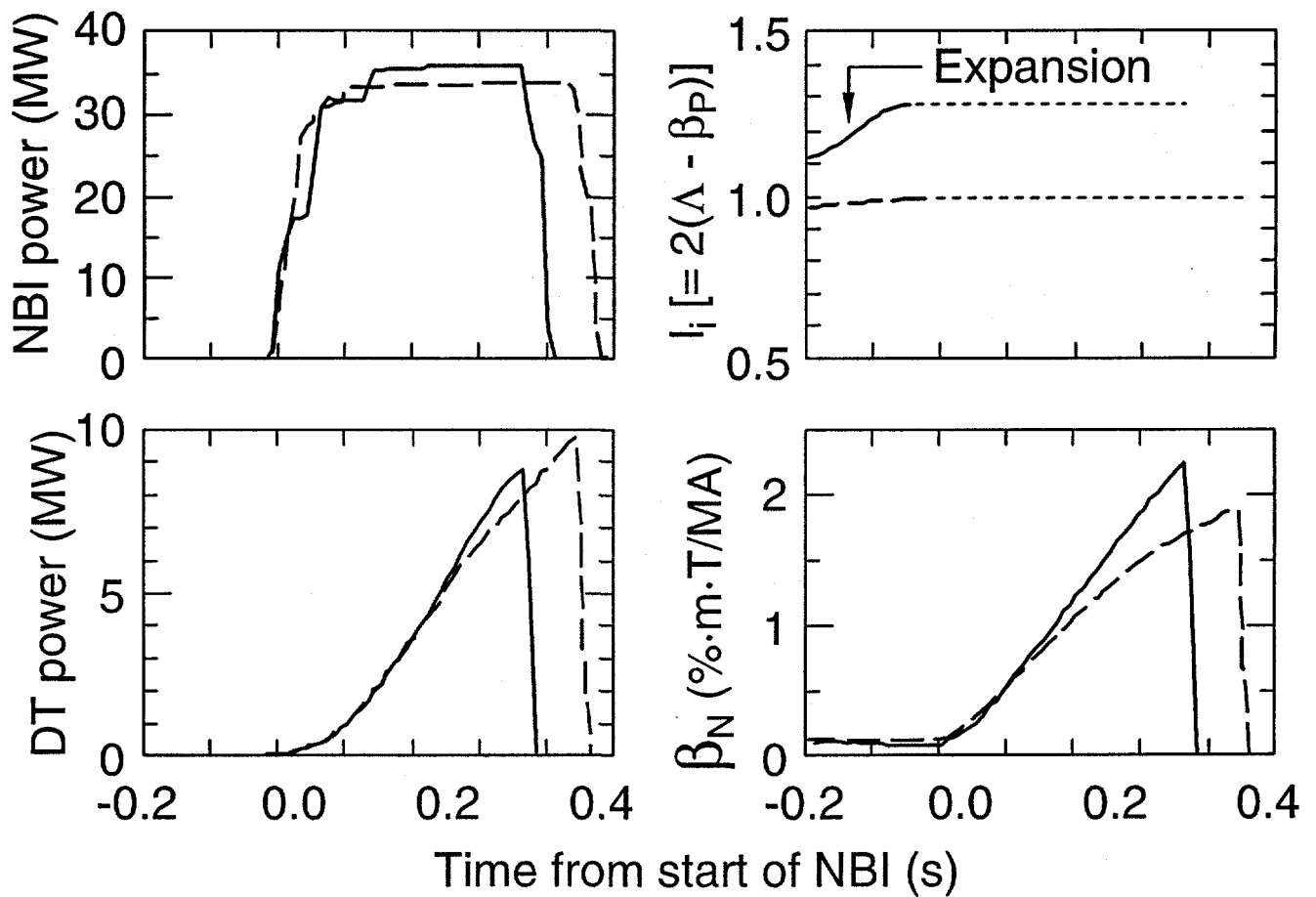
Fig. 6 Comparison of the evolution of high- I_i (2.0 MA, 4.75 T, shown solid) and supershot (2.5 MA, 5.1 T, dashed) D-T plasmas producing similar fusion power. Both plasmas have R_p = 2.52 m, a = 0.87 m during NBI. The internal inductance calculated from magnetic diagnostic data is extrapolated through the NBI pulse when the plasma pressure becomes anisotropic. The increase in the normalized \beta -limit is proportional to the increase in I_i .
