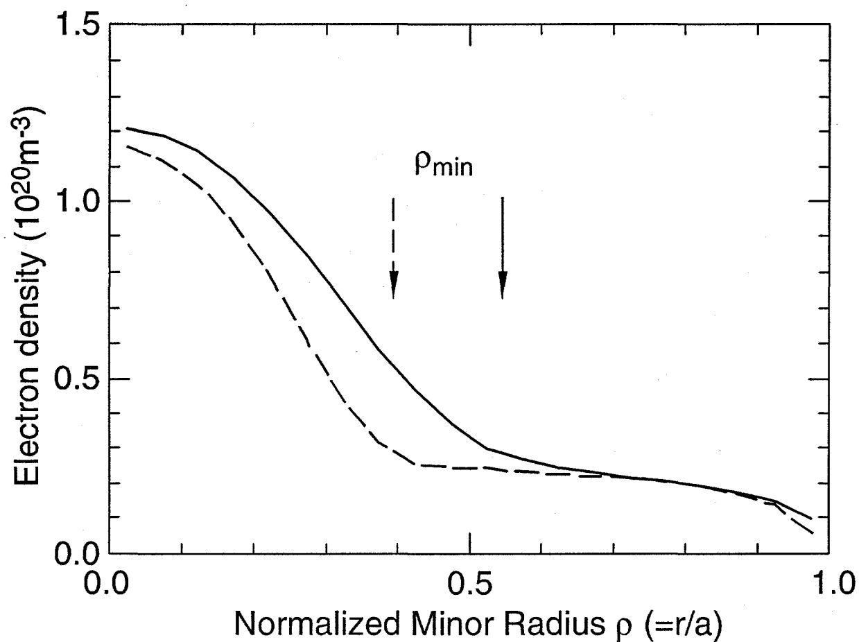
Fig. 3 Profiles of the electron density for 2.2 MA (solid) and 1.6 MA (dashed) ERS plasmas at the time of maximum plasma energy. The radii of minimum q at the start of the high-power NBI phase are indicated. The ERS transport barrier, indicated by the abrupt change in the density gradient, moves out with \rho_{\min} .
