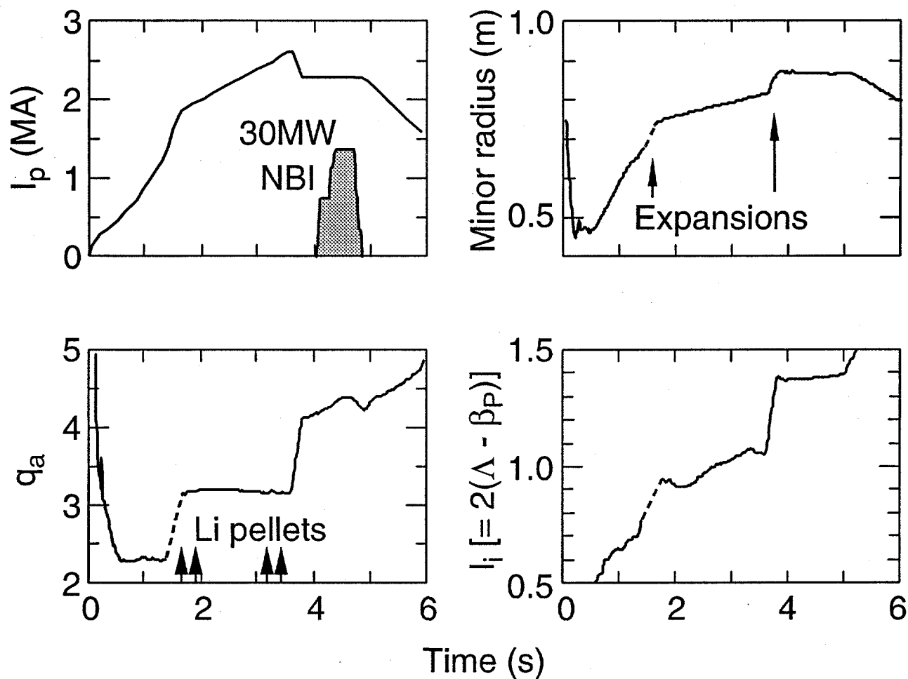
Fig. 5 Technique for producing high- I_i by cross-section expansion. This plasma is initiated on the outer limiter. The edge q is rapidly reduced to 2.4 and maintained there until 1.4s when the plasma is moved onto the inner limiter, raising q_a to 3.2 to allow the injection of 4 lithium pellets for limiter conditioning. At 3.7s, the boundary is expanded again before NBI starts at 4.0 s. The plasma current is slightly reduced during the final expansion to conserve poloidal flux.
