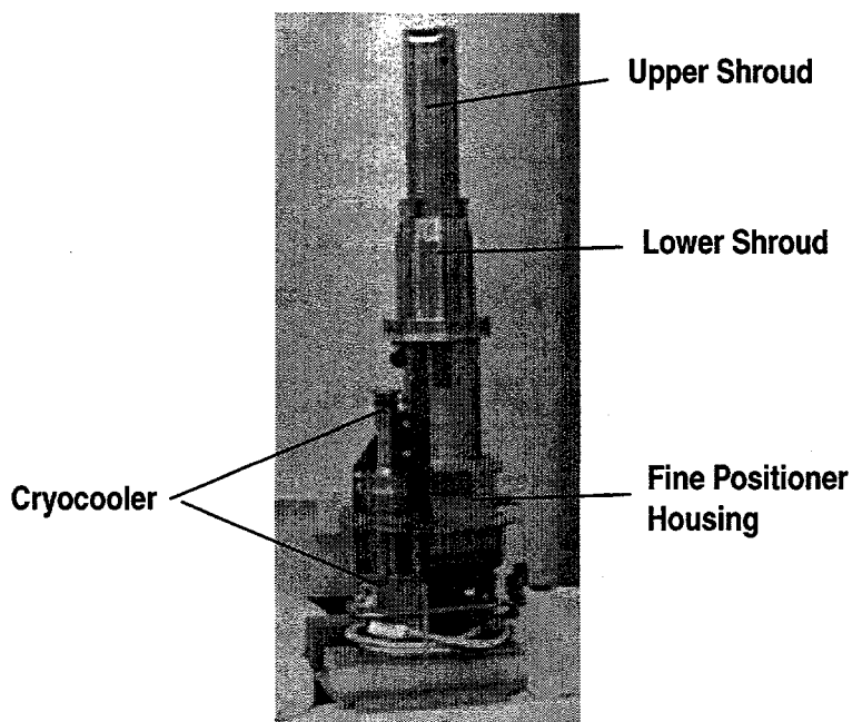
Fig. 6-5. Moving cryostat.
