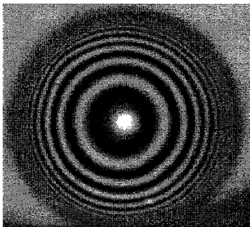
Fig. 2-5. A TiO 2 shell resulting from the pyrolysis of Ti-GDP. The interferometric fringe pattern demonstrates the transparency and wall uniformity of the shell.
