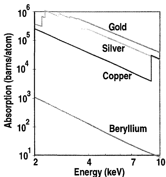
Fig. 2-16. X-ray absorption versus energy for the bonding metals (copper, silver, and gold) compared to pure beryllium.
