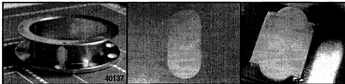
Fig. 3-5. A new application for low density foams is shown here. The photograph on the left is an overview of a current return can with two hole closure foams. The inner diameter of the can is approximately 51 mm. Close-up views of the foams are shown on the right side. The inside view confirms that there is no foam protruding into the can where it could interfere with other target components. The outside view documents the method of securing the foam. The 11 by 4 mm oval is cast with thin side extensions that can be tacked in place with four drops of epoxy — one at each corner. The epoxy is far from the hole so that it is not seen by any diagnostic.
