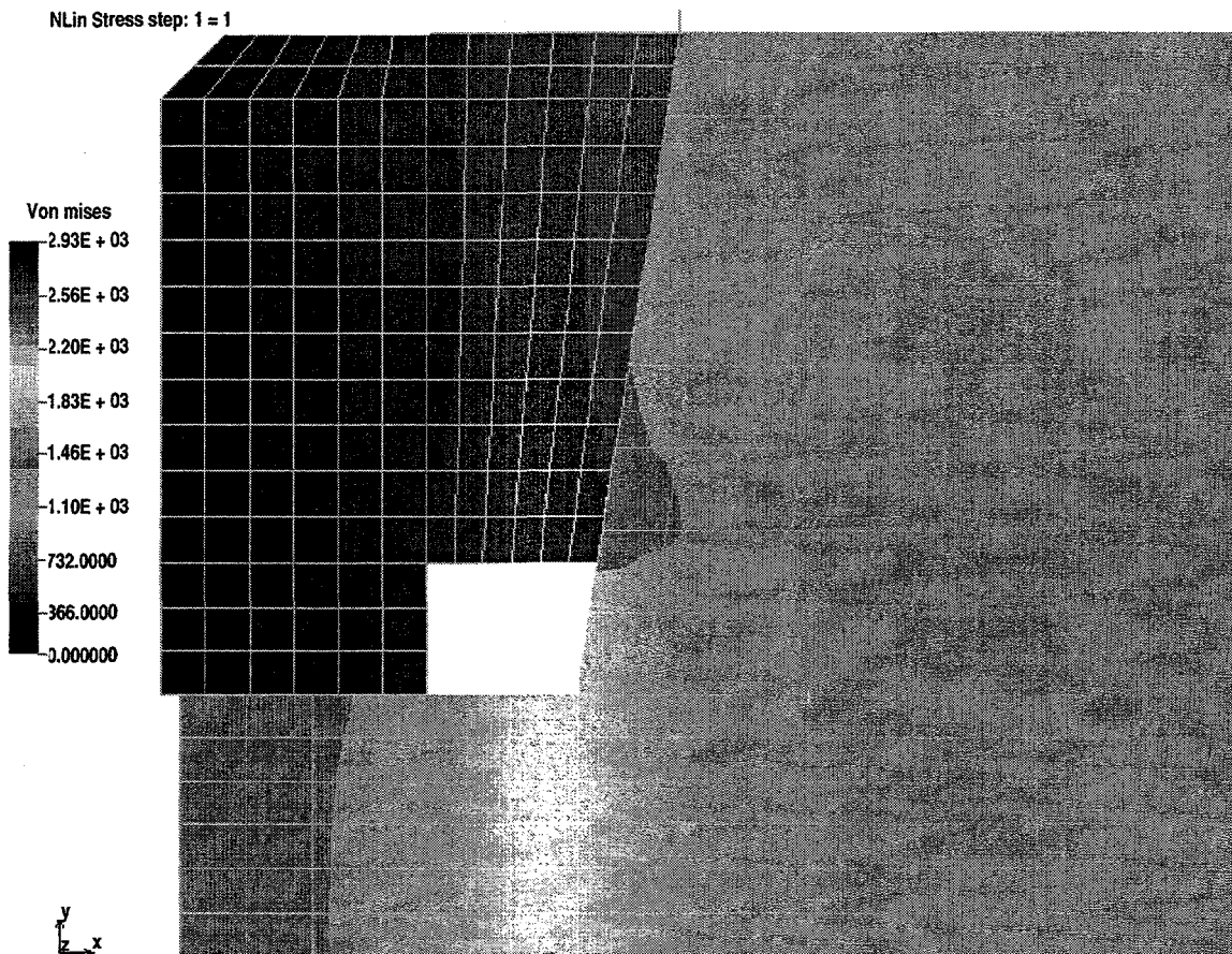
Fig. 5-23. The Von Mises stress is plotted in units of \text{kg/cm}^2 on the deformed plot of the inner and outer seal rings. Notice that the inner ring is now bottomed out on the outer ring. The inner ring is highly stressed, but this stress is below the ultimate yield strength of about 4000 \text{ kg/cm}^2 for annealed C10100 copper at 18 K.
