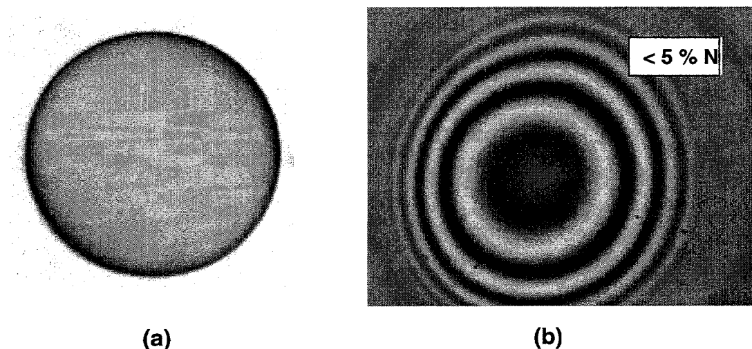
Fig. 2-4. Images of enlarged glass shells. (a) Transmission microscope image of a 1740 \mu\text{m} glass shell expanded from a 1200 \mu\text{m} starting mandrel. Note the absence of any wrinkles or dents. (b) Interferometric image of a 2002 \mu\text{m} glass shell made from a ~1300 \mu\text{m} starting mandrel. The smooth fringe pattern indicates absence of wrinkling or major wall thickness variations in the shell. The wall thickness nonconcentricity is less than 5%.
