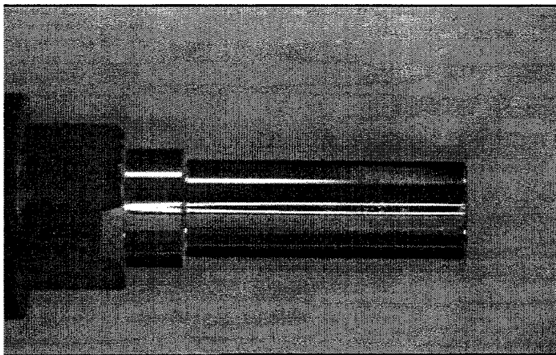
Fig. 1-2. A typical central can mandrel with a copper coating.
