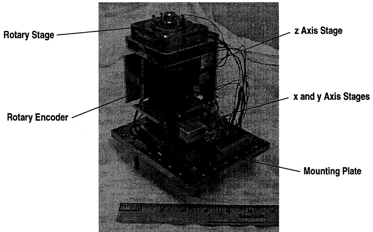
Fig. 6-6 Fine positioner.
