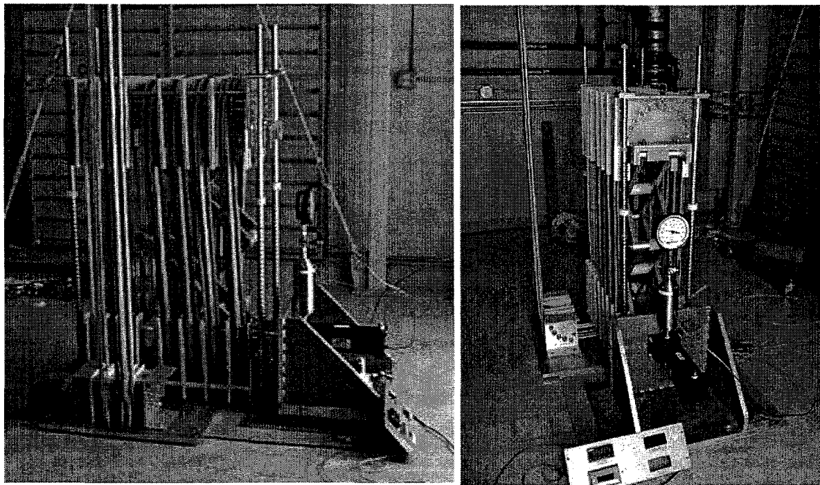
Fig. 6-8. Two views of the spooler.
