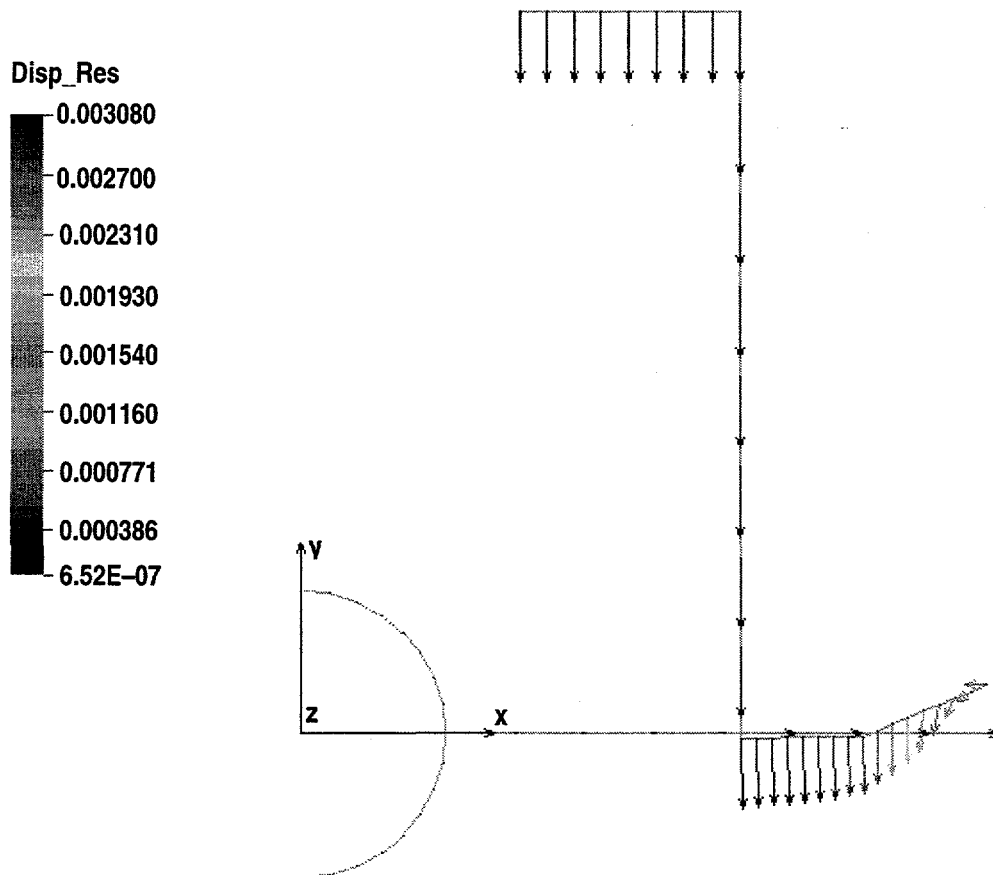
Fig. 5-25. The displacement of the hohlraum due to assembly process is 31\text{ }\mu\text{m} along the inner walls of the hohlraum. This means that the initial gap of the brim above the capsule's mounting film must be increased from 3 to 28\text{ }\mu\text{m} to avoid contacting the film and the other hohlraum half that would be coming up from below. The scale is in centimeters. The inner walls of the hohlraum experience very little radial displacement, most of the radial displacement is in the brim that connects that hohlraum proper to the inner seal ring.
