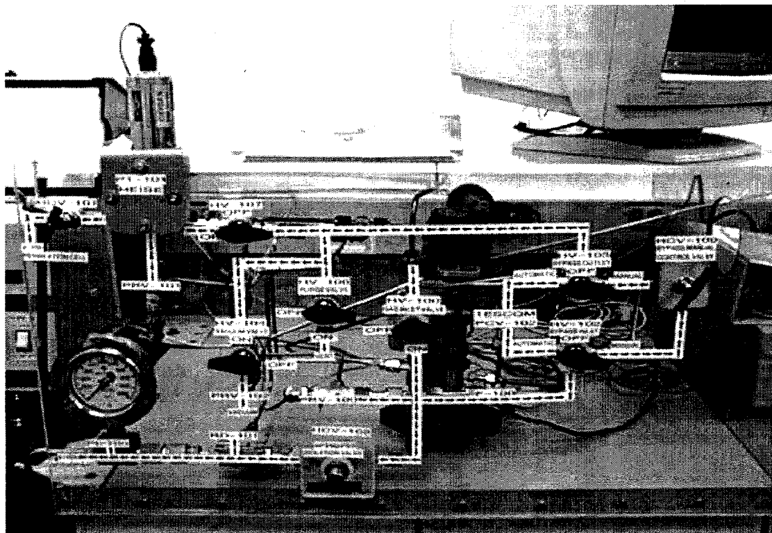
Fig. 2-8. The central portion of the new fill station with computer-controlled pressure regulator.
