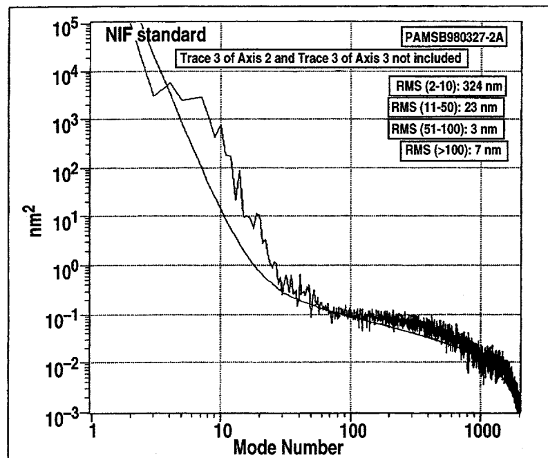
Fig. 2-2. Power spectrum of ~2 mm PAMS bead.
