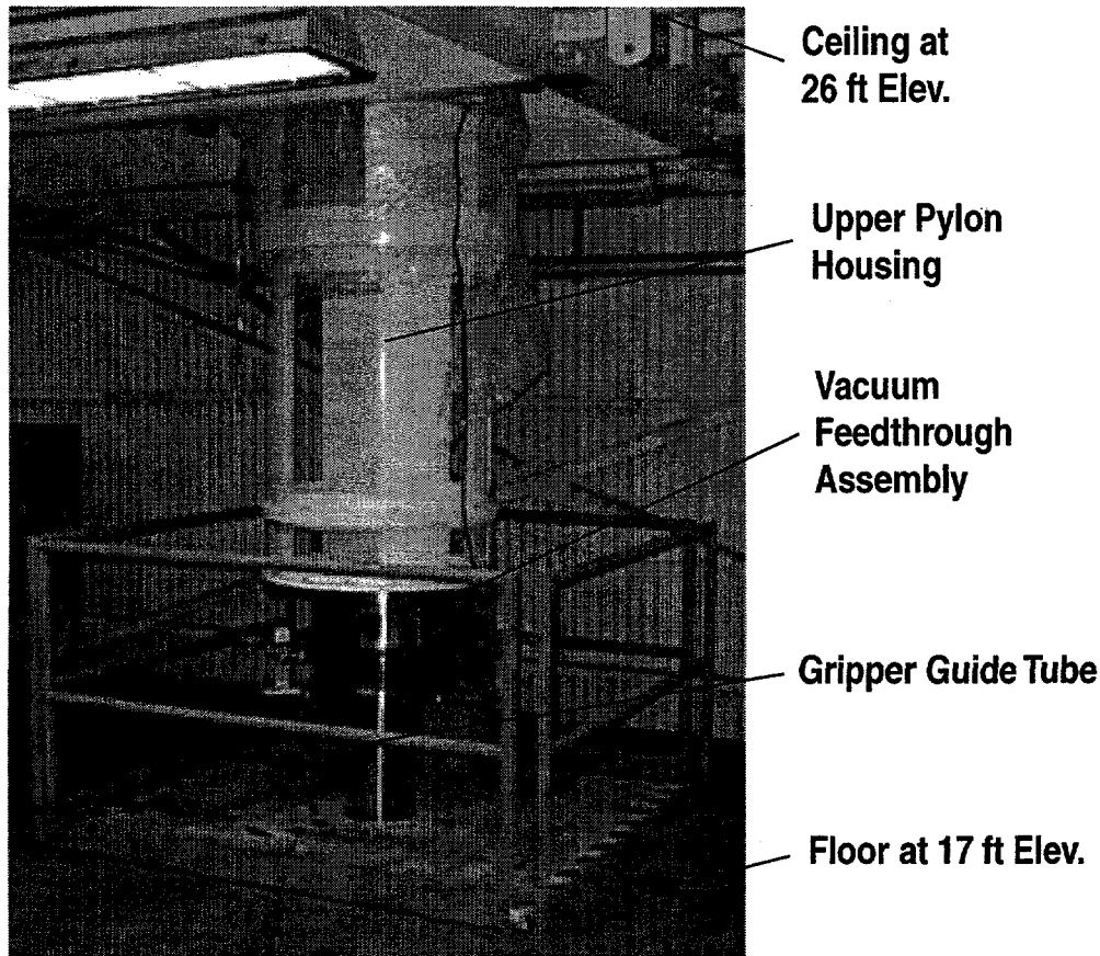
Fig. 6-9. UP segment installed at GA Bldg. 35.
