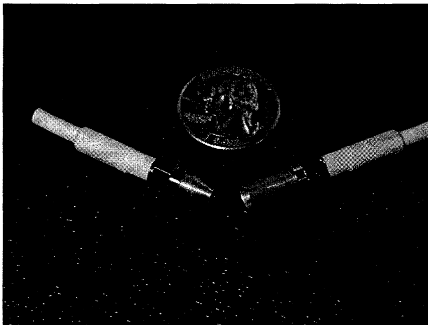
Fig. 5-9. Picture of the conical fittings attached to SMA connectors.
