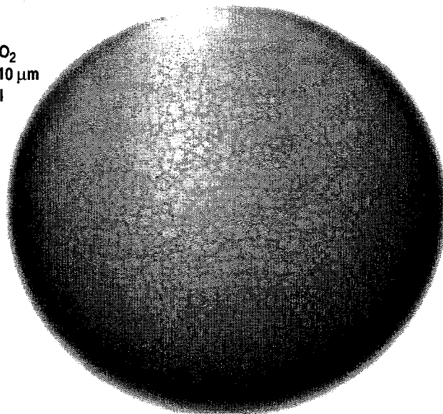
Fig. 2-9. Optical picture of a 0.2\text{ }\mu\text{m} glass coating on a \sim 900 diameter \times 10\text{ }\mu\text{m} GDP shell. The coating had developed numerous microcracks when examined after coating. This did not happen for coatings of 0.4\text{ }\mu\text{m} or thicker.
