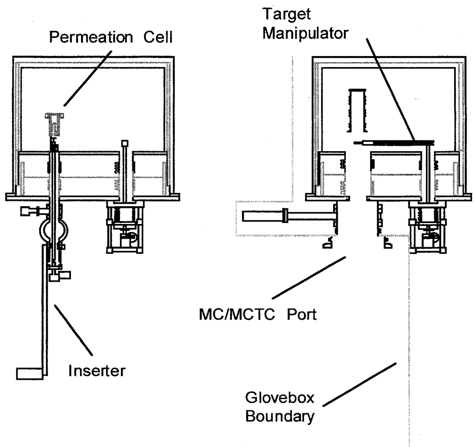
Fig. 6-1. FTS section views.
