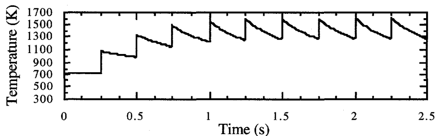
FIGURE 6. A calculation that shows the temperature of a SiC fiber placed in the APT 1.7-GeV beam. The beam is pulsed at 4-Hz with a 0.15-ms long pulse and a current density of 1.6 \text{ A/cm}^2 .
