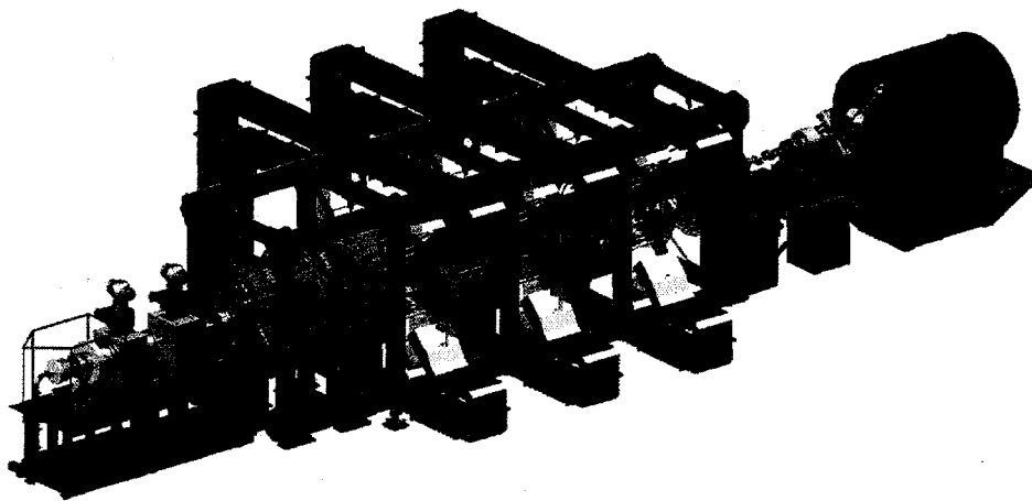
FIGURE 2. The first LEDA experiment configuration that includes the 75-keV injector, the 6.7-MeV RFQ, a short HEBT, and a 670-kW beamstop, is shown.
