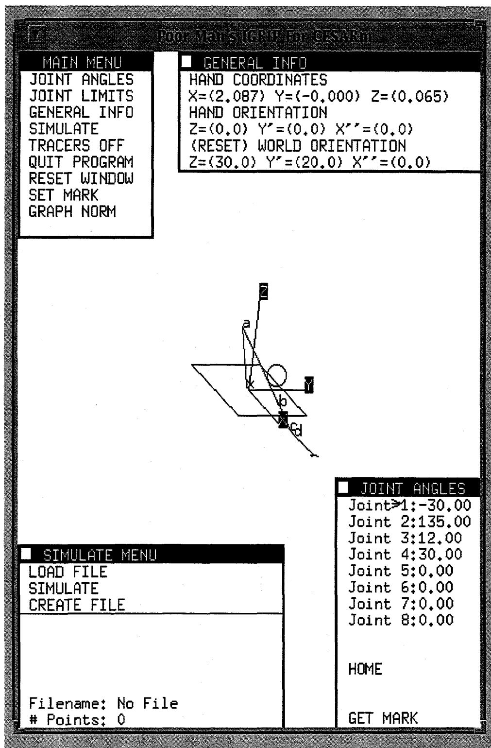
Figure B1d: CheezyIGRIP Simulator
