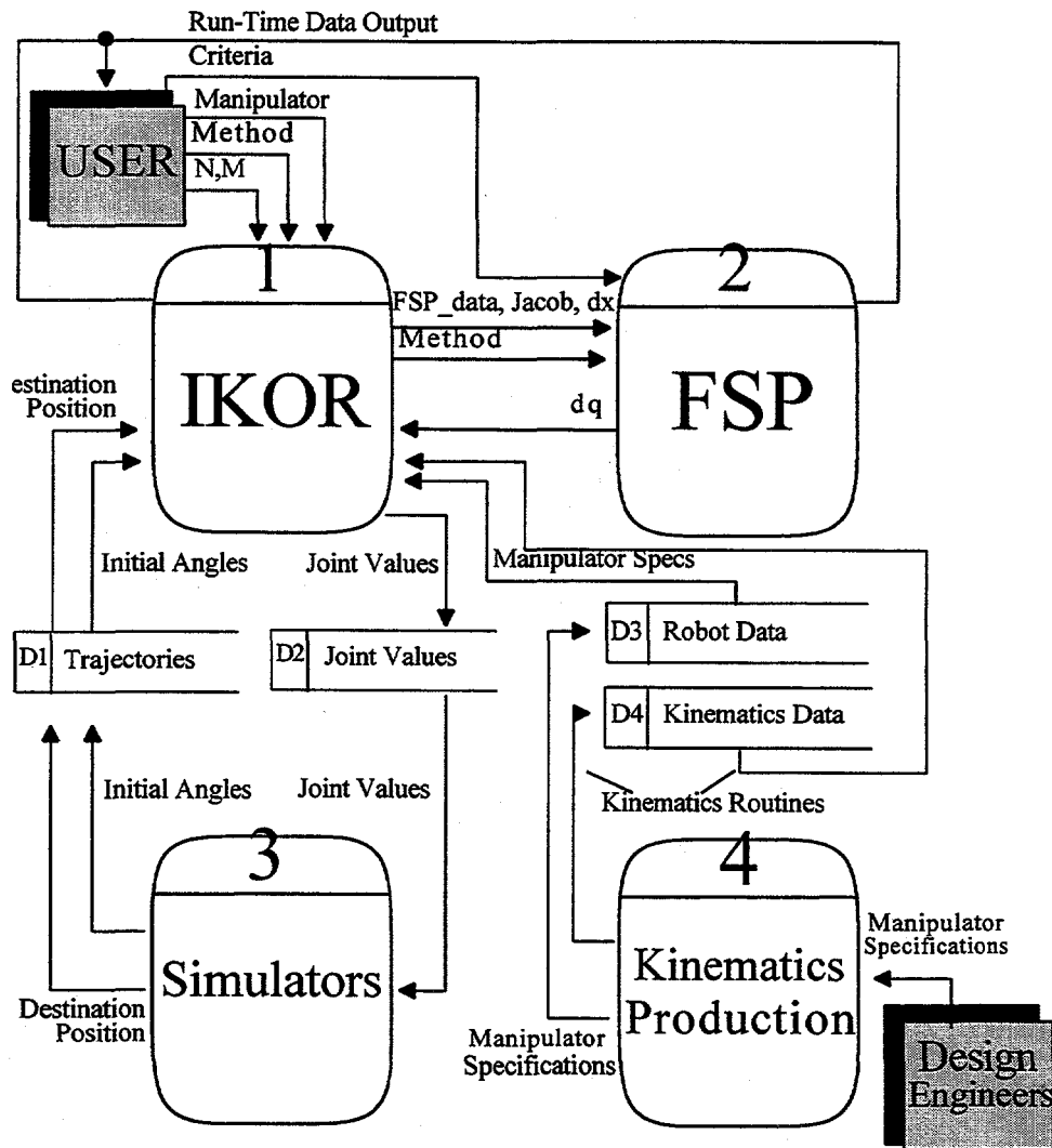
Figure C1a: Context Data Flow Diagram
