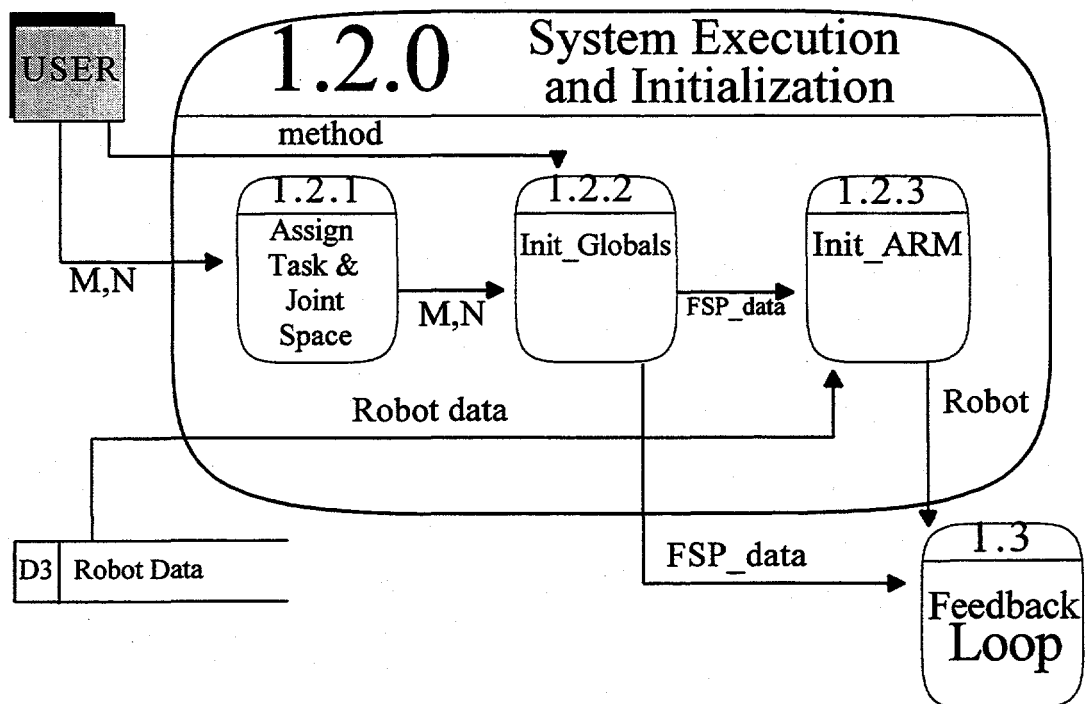
Figure C1e: Level 2 Data Flow Diagram
