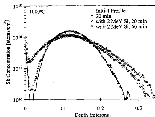
Fig. 1. Sb concentration profiles in SOI showing the initial Sb marker, annealed at 1000°C followed by 20-min anneal, implanted with MeV Si + , and implanted with MeV Si + followed by a 60-min anneal.
