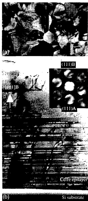
Fig. 1. (a) bright-field plan view image of a thin CdTe layer showing many small domains at the initial growth stage; (b) bright-field cross-sectional image showing the lamellae twins in the CdTe layer and twin-free region with inset showing CBED pattern, indicating the Te-terminated orientation.
