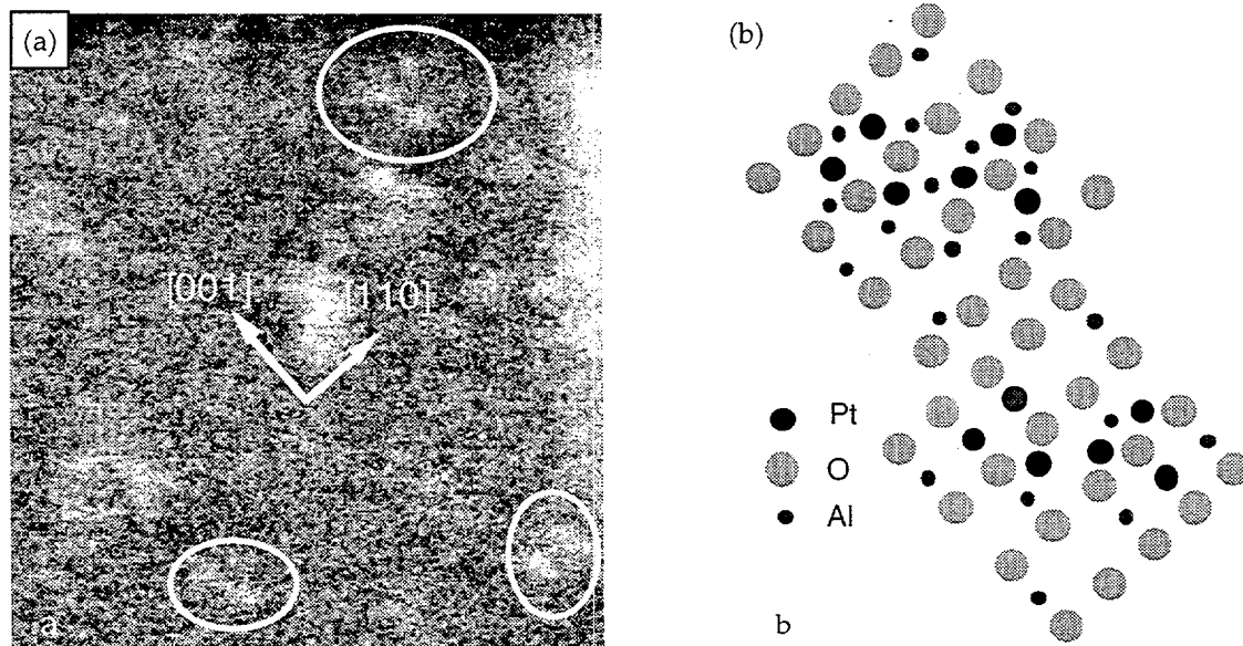
Fig. 1. (a) Z-contrast image of small Pt clusters on \gamma -Al 2 O 3 . Circled are examples where individual Pt atoms form dimers and trimers. (b) Schematic showing the two (110) surfaces possible for \gamma -Al 2 O 3 with possible Pt configurations.
