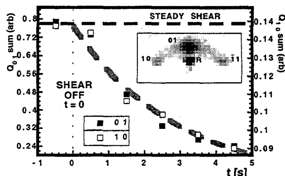
Fig. 1. Decay of integrated 01 and 10 diffraction peak intensities (shown in inset) after cessation of flow ( t = 0 ).
