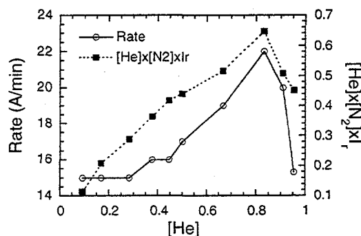
Fig. 3. Graphs of deposition rate and [\text{He}][\text{N}_2]I_r vs. fraction of He in the process gas.
