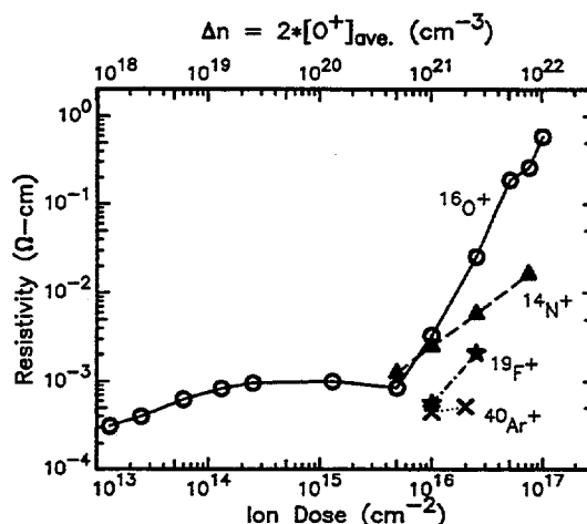
Fig. 1. Conductivity changes induced in ITO films by implantation of \text{N}^+ , \text{O}^+ , \text{F}^+ , and \text{Ar}^+ .
