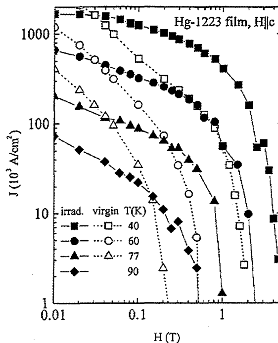
Fig. 1. The persistent current density J vs. magnetic field H , for a Hg-1223 film at the temperatures shown. The film, with a 40- \mu m Pb overlayer, was irradiated with 5.8 \times 10^{16} p/cm 2 . J is significantly increased, especially at higher fields.
