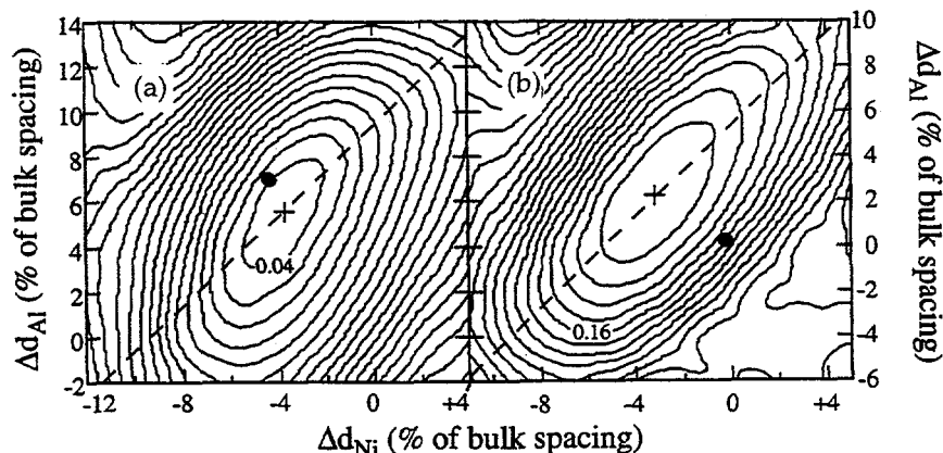
Fig. 1. Contour plot of quality of agreement, indicating Ni and Al outerlayer spacings for clean (a) and H-saturated (b) experiments (+) and theory (●).
