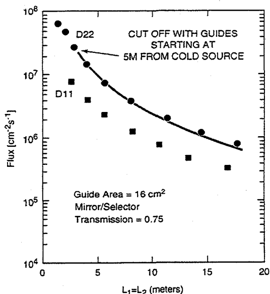
Fig. 1. ORNL flux simulation (4/97) with Monte Carlo neutron photon cold neutron library H2-cross sections ( \lambda = 10 Å, \Delta\lambda/\lambda = 10\% ).
