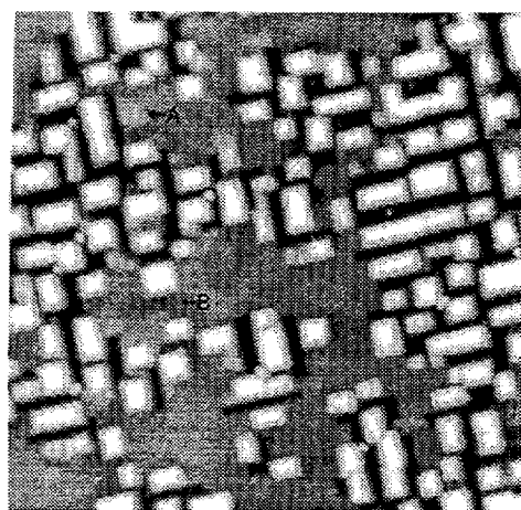
Fig. 1. Atomic force microscopy image of a 5-nm thick \text{Si}_{0.5}\text{Ge}_{0.5} alloy layer grown on \text{Si}(001) and annealed for 5 min. at 550^\circ\text{C} . This image reveals cooperative nucleation of discontinuous surface ripple domains where islands and pits nucleate adjacent to each other as indicated.
