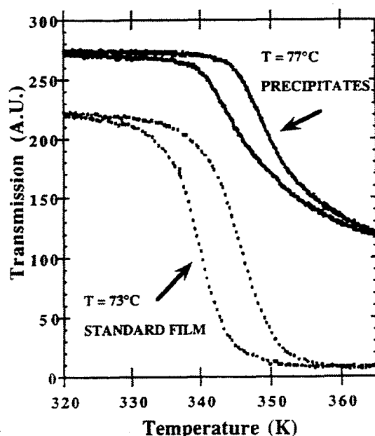
Fig. 1. Optical transmission spectrum at 3.4 \mu m showing the hysteretic VO 2 phase transition for: (a) VO 2 precipitates in Al 2 O 3 coimplanted with V and O and annealed (top: T_c \sim 77^\circ\text{C} ) and (b) a thin film of VO 2 deposited on Al 2 O 3 (bottom: T_c \sim 73^\circ\text{C} ).
