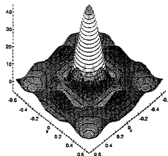
Fig. 1. Magnetization density in \text{SrRuO}_3 determined from polarized neutron diffraction. The density plotted is from the central plane of a pseudo-cubic unit cell. The large peak in the center arises from the Ru atom and the four smaller peaks are the surrounding oxygen atoms.
