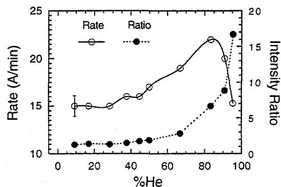
Fig. 2. Deposition rate and ratio of emission line intensities, I[\text{N}]/I[\text{N}_2(0,3)] as a function of %He in the process gas.
