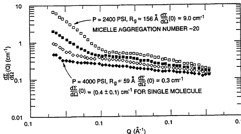
Fig. 1. d\Sigma/\Omega(Q) for 6% (w/v) PVA- b -PFOA block copolymers in CO 2 . At high pressures, the scattering arises from single molecules; as the pressure is lowered, micelles form below a critical density.
