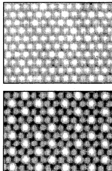
Fig. 1. STM topograph of Sn/Ge(111) at room temperature (upper panel) and at 90 K (lower panel). Between these temperatures, a reversible, two-dimensional phase transition occurs, producing a lower symmetry and new electron distribution.
