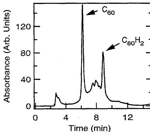
Fig. 1. Chromatogram of an ultrasonically irradiated sample of C_{60} in decahydronaphthalene.
