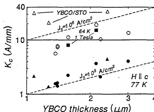
Fig. 1. The loss-free current K_c carried per unit width of tape for different YBCO layer thicknesses at 77 K. Open symbols: zero applied field. Closed symbols: 1-T applied field. Solid line: K_c = 10 A/mm, a proposed practical operation criterion. Squares: data in 64-K liquid nitrogen.
