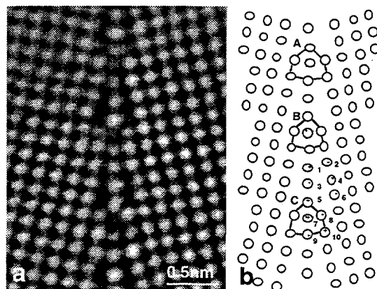
Fig. 1. (a) High-resolution Z-contrast image of a symmetric 27^\circ[001] grain boundary in \text{MgO} and (b) the boundary structure derived from the image.
