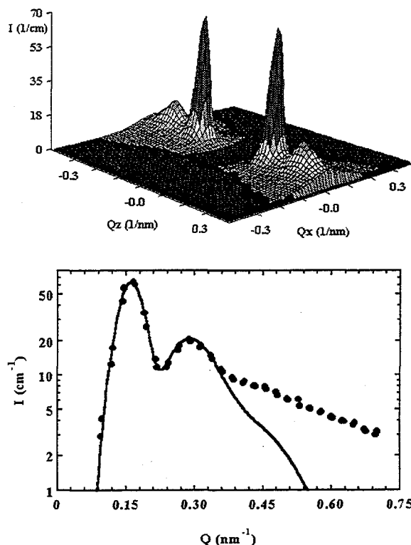
Fig. 1. Couette SANS pattern for 70:30 CTA35CIBz/CTABr in D 2 O at 200 s -1 . Graph shows Q_x = 0 slice data. Line is powder model.
