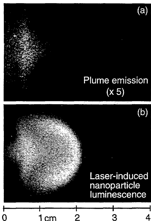
Fig. 1. Intensified CCD-array photographs (3- \mu s exposures) taken 400 \mu s after KrF-laser ablation of a silicon wafer into 10-Torr helium gas showing (a) remaining visible plume emission near the silicon wafer surface and (b) nanoparticle luminescence induced by passing a sheet of 308-nm light through the plume.
