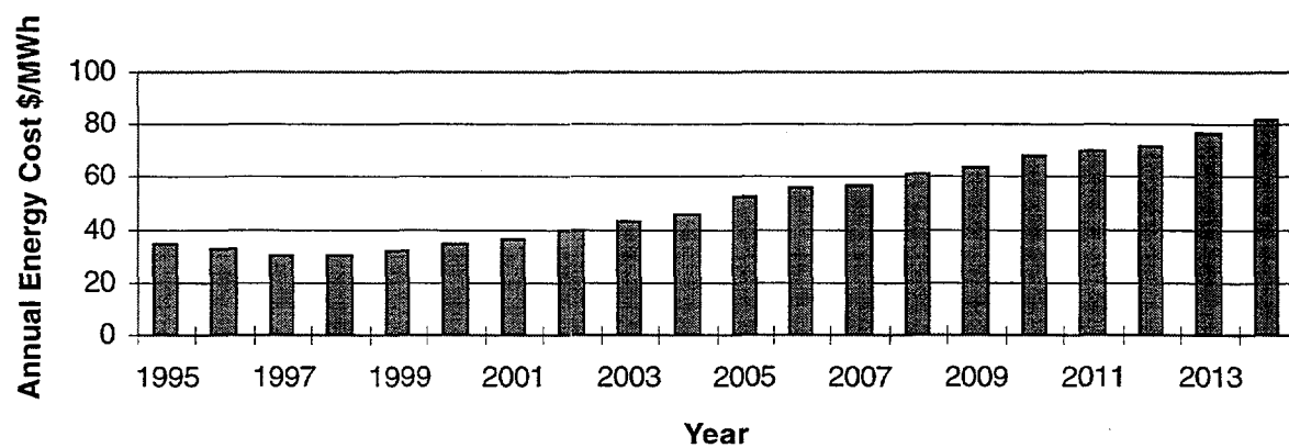
Figure 3-19. Annual SMUD Marginal Energy Costs, Summer Peak Period.
