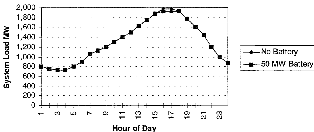
Figure 3-9. Expected Daily Battery Discharge Requirement to Shave Peak—June 1992 Peak Day Load Shape.
