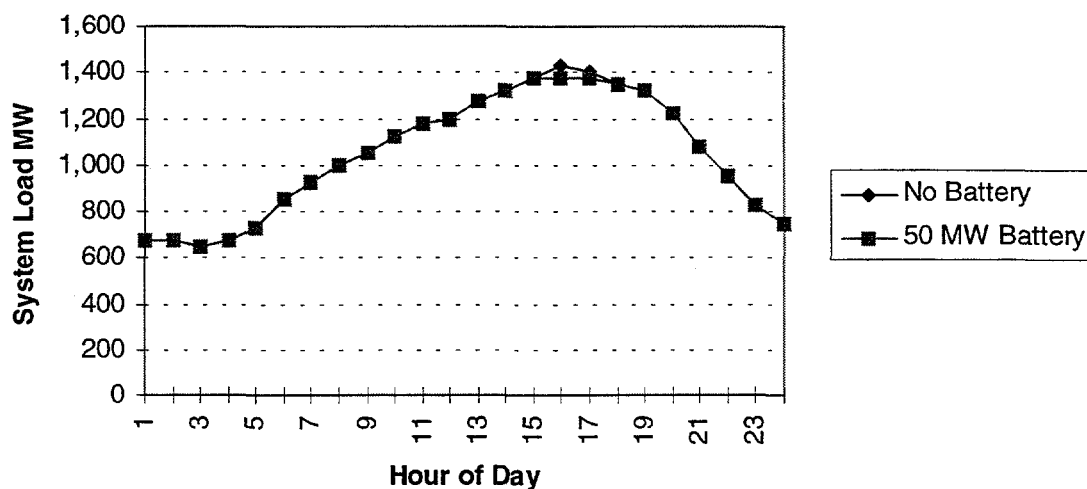
Figure 3-13. Expected Daily Battery Discharge Requirement to Shave Peak—October 1992 Peak Day Load Shape.
