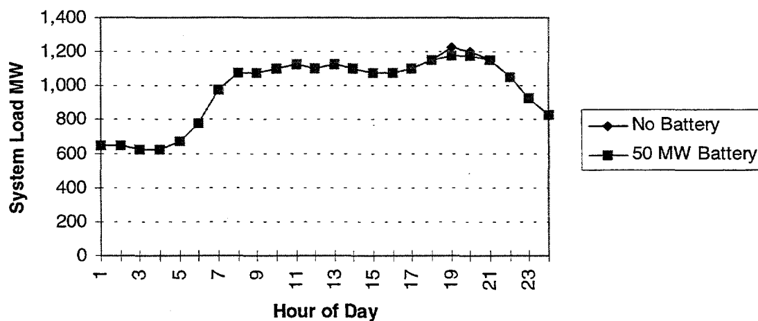
Figure 3-6. Expected Daily Battery Discharge Requirement to Shave Peak—March 1992 Peak Day Load Shape.
