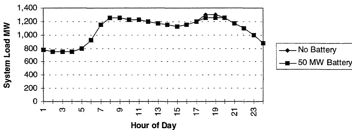
Figure 3-14. Expected Daily Battery Discharge Requirement to Shave Peak—November 1992 Peak Day Load Shape.
