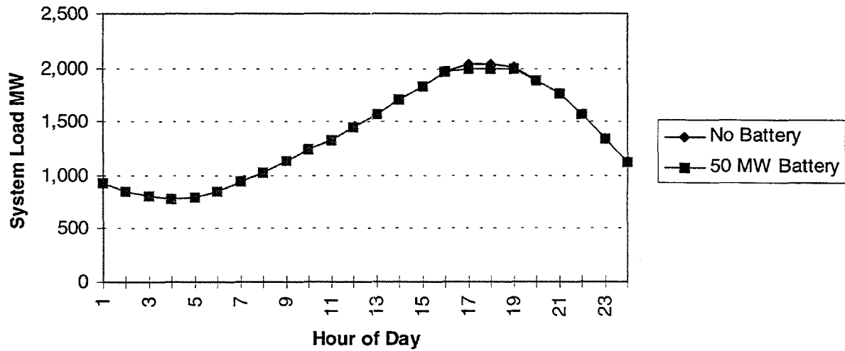
Figure 3-3. Expected Daily Battery Discharge Requirement to Shave Peak—August 16, 1994, Residual Load.
