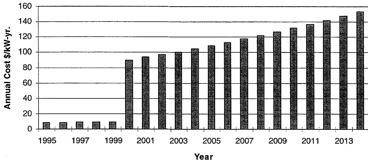
Figure 3-16. Annual SMUD Marginal Capacity Costs.
