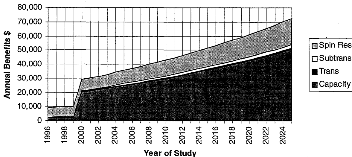
Figure 4-3. Potential Benefits of Adding a 225-kV/2-Hr Battery at Hedge (Case 2).
