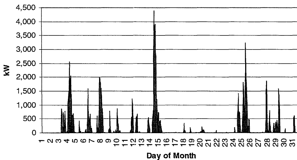
Figure 2-6. Aggregated kW Output of the Solano Wind Plant for December 1994.
