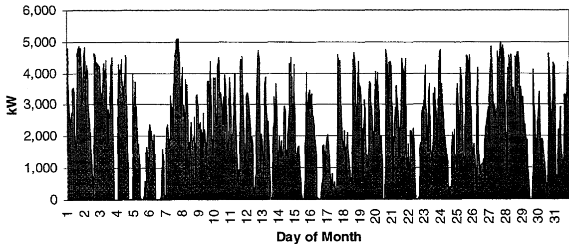
Figure 2-2. Aggregated kW Output of the Solano Wind Plant for August 1994.
