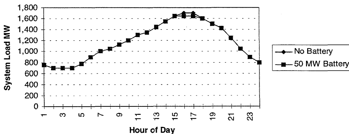
Figure 3-12. Expected Daily Battery Discharge Requirement to Shave Peak—September 1992 Peak Day Load Shape.
