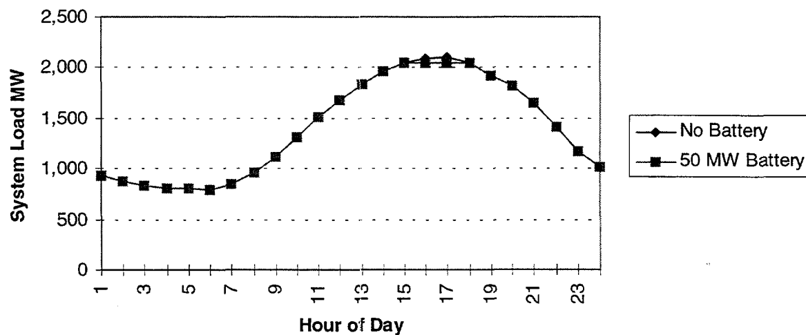
Figure 3-11. Expected Daily Battery Discharge Requirement to Shave Peak—August 1992 Peak Day Load Shape.
