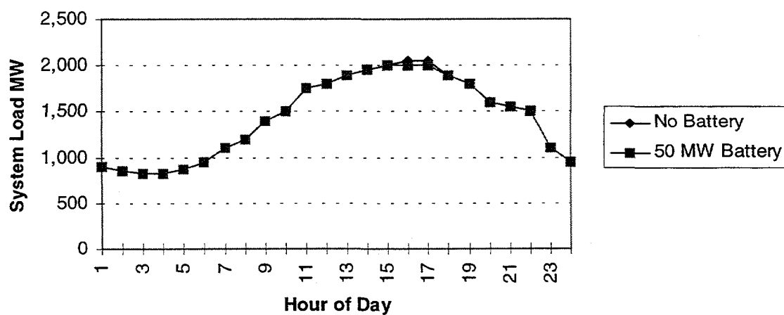
Figure 3-10. Expected Daily Battery Discharge Requirement to Shave Peak—July 1992 Peak Day Load Shape.
