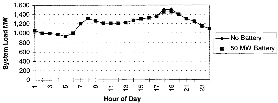
Figure 3-4. Expected Daily Battery Discharge Requirement to Shave Peak—January 1992 Day Load Shape.
