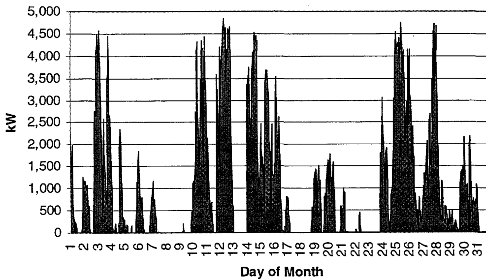
Figure 2-4. Aggregated kW Output of the Solano Wind Plant for October 1994.
