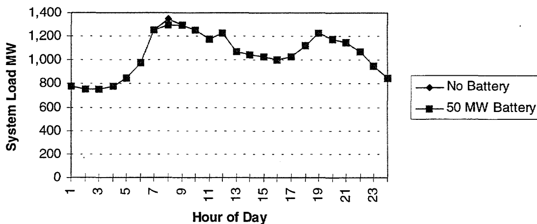
Figure 3-5. Expected Daily Battery Discharge Requirement to Shave Peak—February 1992 Peak Day Load Shape.
