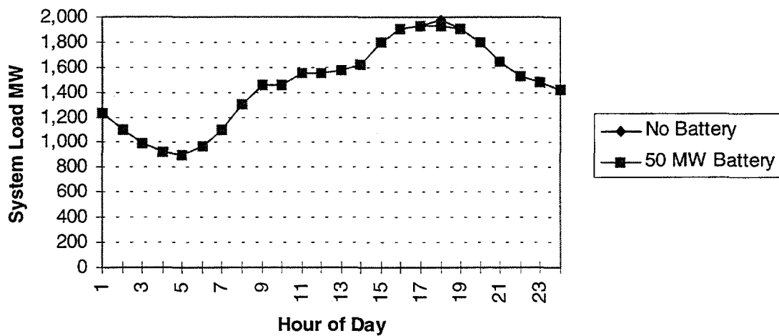
Figure 3-1. Expected Daily Battery Discharge Requirement to Shave Peak—Projected 112°F Peak Day Residual Load.
