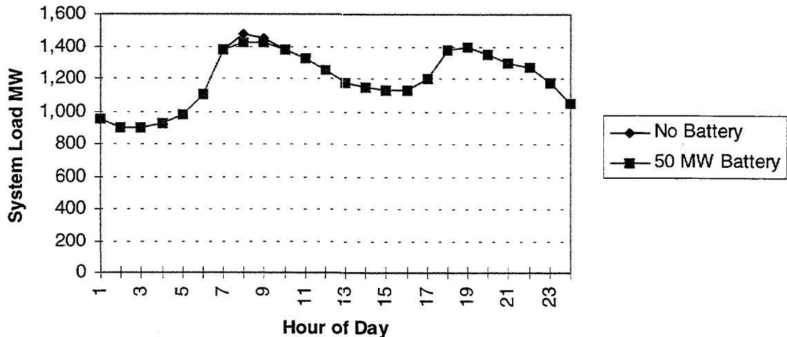
Figure 3-15. Expected Daily Battery Discharge Requirement to Shave Peak—December 1992 Peak Day Load Shape.
