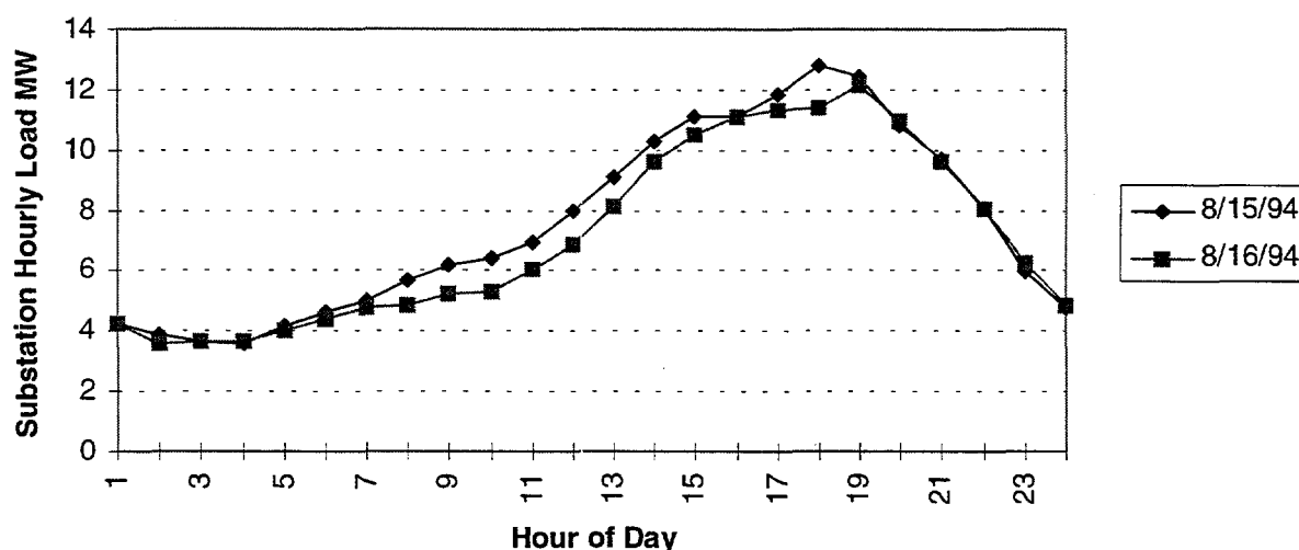
Figure 3-18. Representative Daily Elk Grove Florin/Gerber Substation Load Shape.
