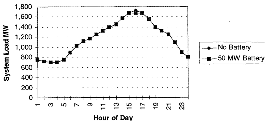
Figure 3-8. Expected Daily Battery Discharge Requirement to Shave Peak—May 1992 Peak Day Load Shape.
