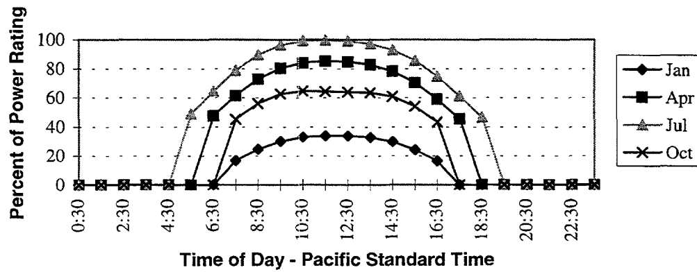
Figure 2-9. SMUD Single-Axis Tracking PV Seasonal Percent of Power Rating.
