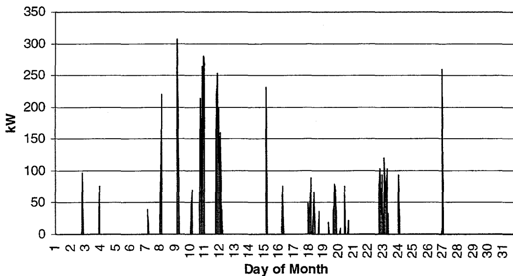
Figure 2-7. Aggregated kW Output Exceeding 5,000 kW for the Solano Wind Plant for July 1994.
