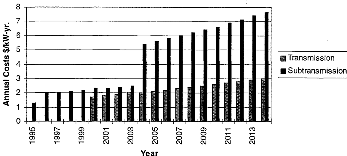
Figure 3-17. Annual Marginal Transmission and Subtransmission Capacity Costs.
