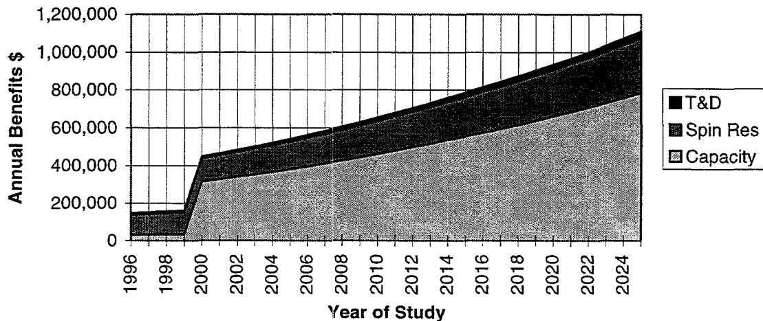
Figure 4-1. Potential Benefits of Adding a 3.5-MW/2-Hr Battery at Solano (Case 1).
