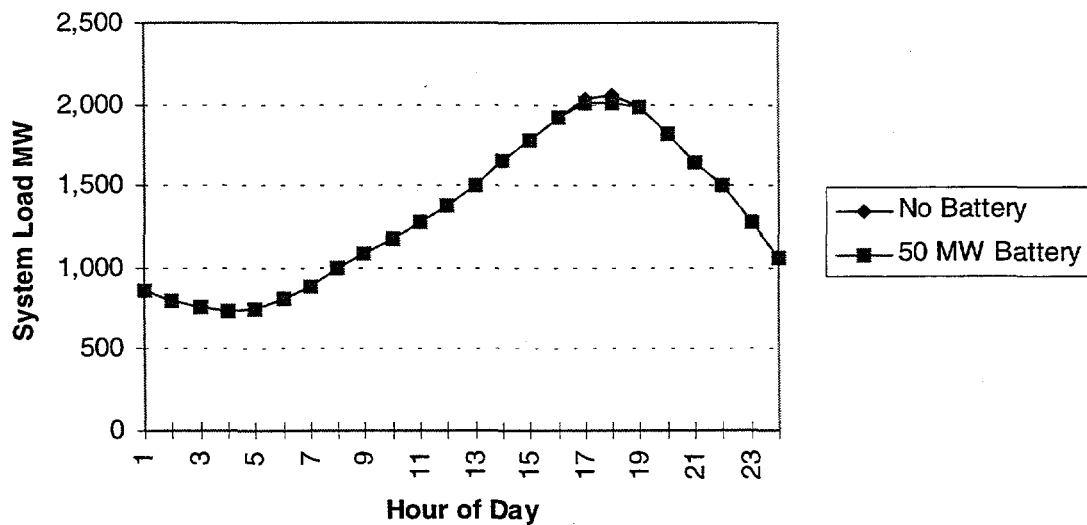
Figure 3-2. Expected Daily Battery Discharge Requirement to Shave Peak—July 14, 1994, Residual Load.
