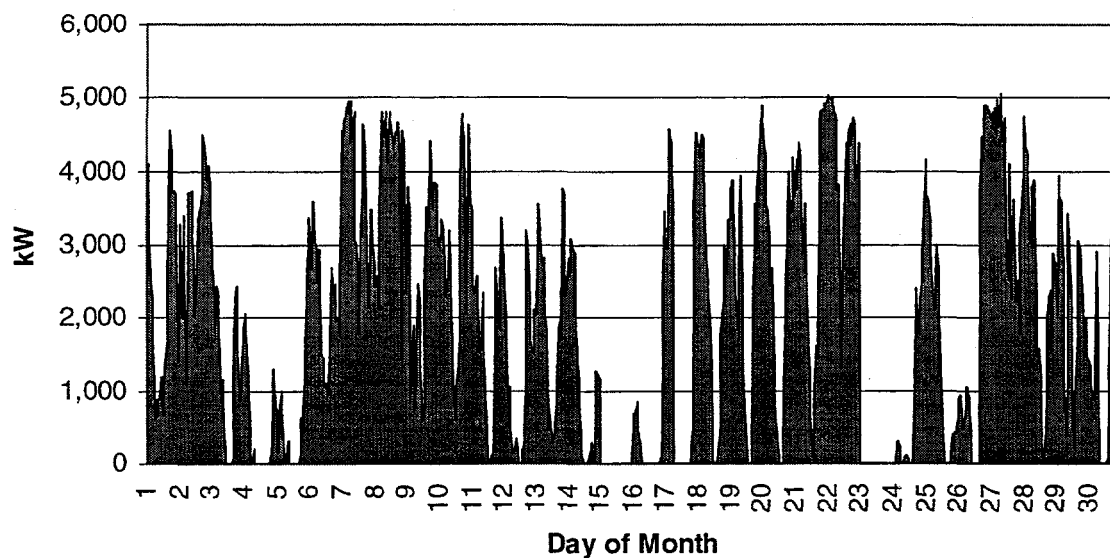
Figure 2-3. Aggregated kW Output of the Solano Wind Plant for September 1994.
