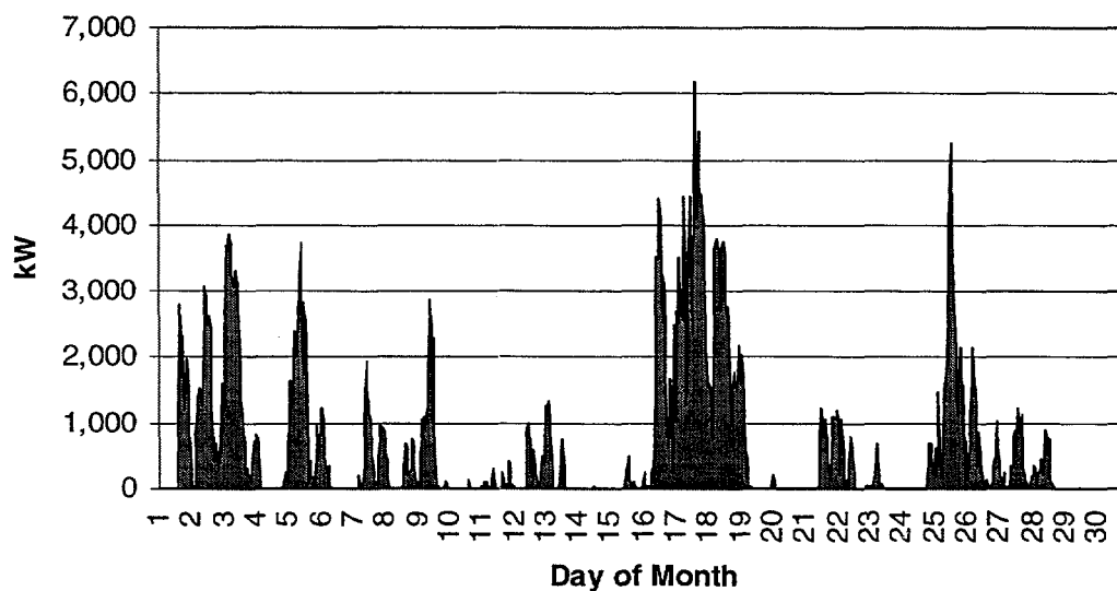
Figure 2-5. Aggregated kW Output of the Solano Wind Plant for November 1994.
