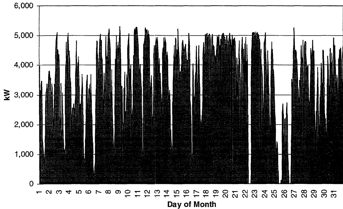
Figure 2-1. Aggregated kW Output of the Solano Wind Plant for July 1994.
