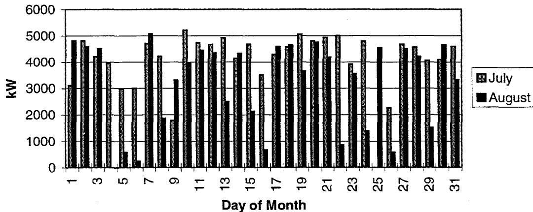
Figure 2-8. Aggregated kW Output of the Solano Wind Plant at 6:00 p.m. for July and August 1994.
