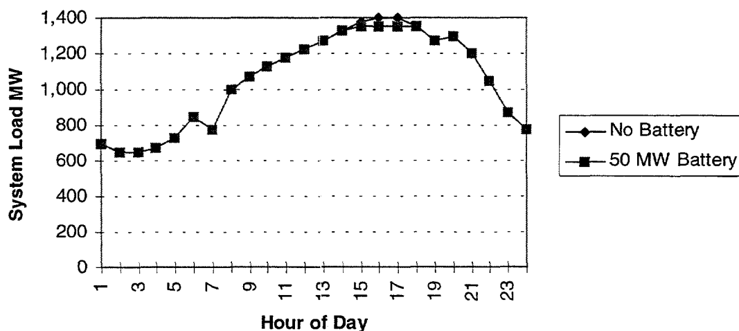
Figure 3-7. Expected Daily Battery Discharge Requirement to Shave Peak—April 1992 Peak Day Load Shape.
