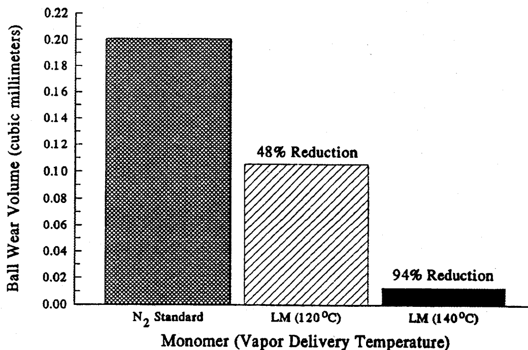
Fig. 2. Effect of Lauryl Methacrylate Vapor on Ceramic Wear Using Nitrogen as the Carrier Gas ( 145^{\circ}\text{C} Bulk Temperature) [11]
