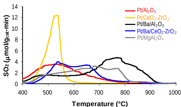
FIGURE 5. Pt/Al 2 O 3 , Pt/Ceria-Zirconia, Pt/Ba/Al 2 O 3 , Pt/Ba/Ceria-Zirconia, and Pt/MgAl 2 O 4 desulfation profiles following sulfation at 400°C.
