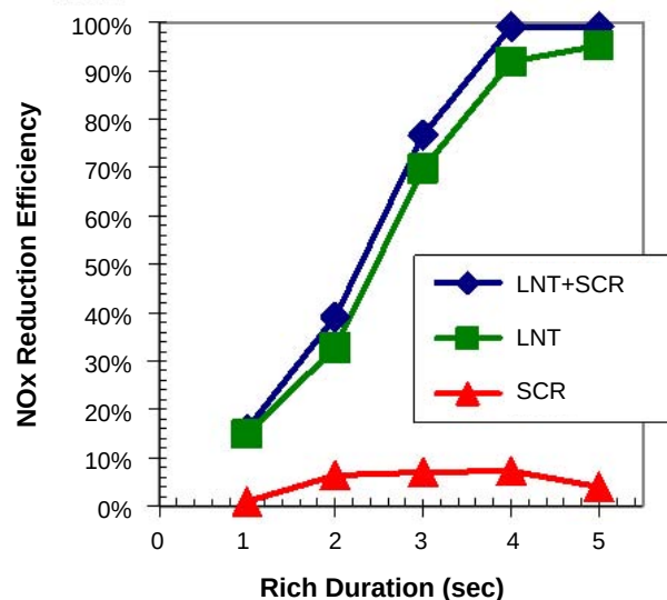
FIGURE 4. NO x reduction efficiency of the LNT and SCR components as well as the combined LNT+SCR NO x reduction efficiency as a function of the rich duration of the LNT regeneration.
