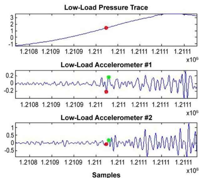
FIGURE 2. Comparison of the identification of the start of combustion using the developed algorithm with the industry standard method.
