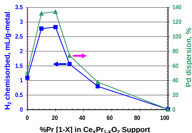
FIGURE 5. Summary of H_2 chemisorption studies, presented as mL H_2 chemisorbed ( 0^\circ\text{C} , 1 atm) per gram of metal, and effective percentage palladium metal dispersion, for 2\%\text{Pd}/\text{Ce}_x\text{Pr}_{1-x}\text{O}_2 where X = 1, 0.9, 0.8, 0.7, 0.5 , and 0 .
