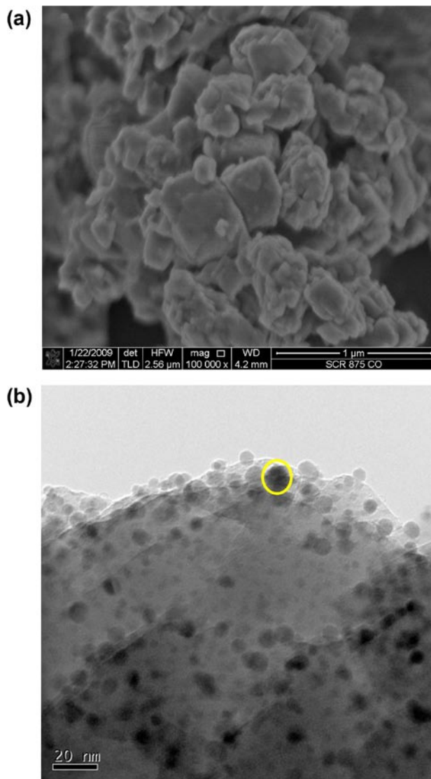
FIGURE 5. SEM (a) and TEM (b) Micrographs of a Heavily Aged Urea-SCR Catalyst
