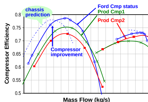
Turbocharger Compressor Efficiency 70,000 RPM, Bench Test and Simulation Results (Sun, Ford)
