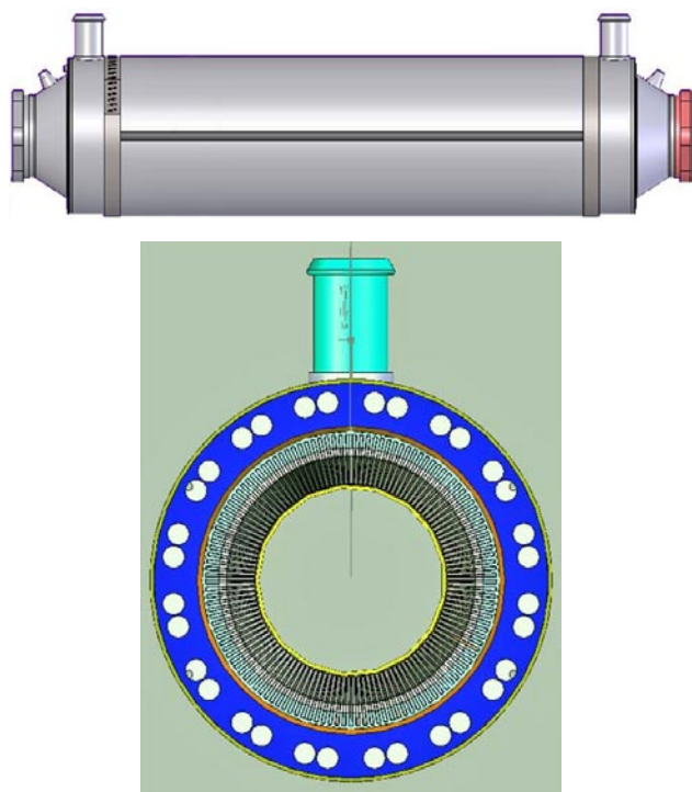
FIGURE 3. TEG Plan and Cross Section Views
