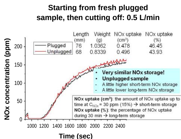
FIGURE 1. 'Flow-Through' versus 'Wall-Flow' NOx Uptake Performance
