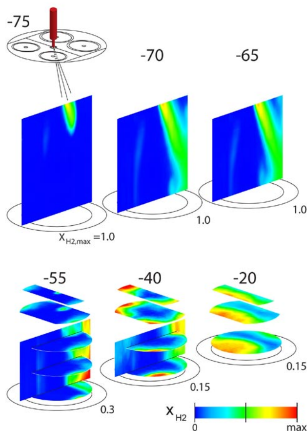
FIGURE 1. Time series of mean fuel mole-fraction x_{H_2} in two orthogonal sets of planes for injection from a single-hole injector with SOI = -80^\circ crank angle (CA). The crank angle of the measurement is indicated above each image assembly. The color scale varies as indicated below the images. The vertical dimension has been stretched by about a factor of three to better visualize the stacked horizontal planes. Piston top and engine-head geometry are shown schematically. Note that the valves are not in a flat configuration in the actual engine, but in the pent-roof geometry typical for spark-ignition engines.
