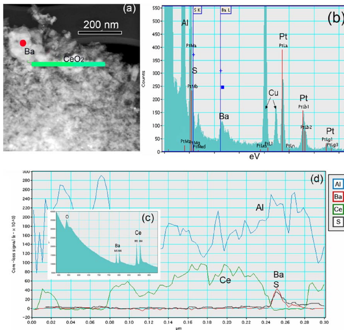
FIGURE 3. (a) STEM image for aged 30-100 showing \text{Al}_2\text{O}_3 support and Ba-rich nodules, as well as a \text{CeO}_2 -rich area. The solid line indicates the EELS line scan region; (b) EDS spectrum recorded at the marked dotted area shown in (a); (c) EELS spectrum taken at the dotted area in (a); (d) EELS trace-line: the line is shown in (a). The trace line included 30 EELS measurements along the distance. S-enrichment is seen at the interface between \text{Al}_2\text{O}_3 and \text{CeO}_2 .
