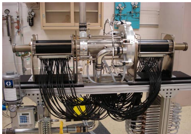
FIGURE 3. The Sandia HFPE Research Prototype
