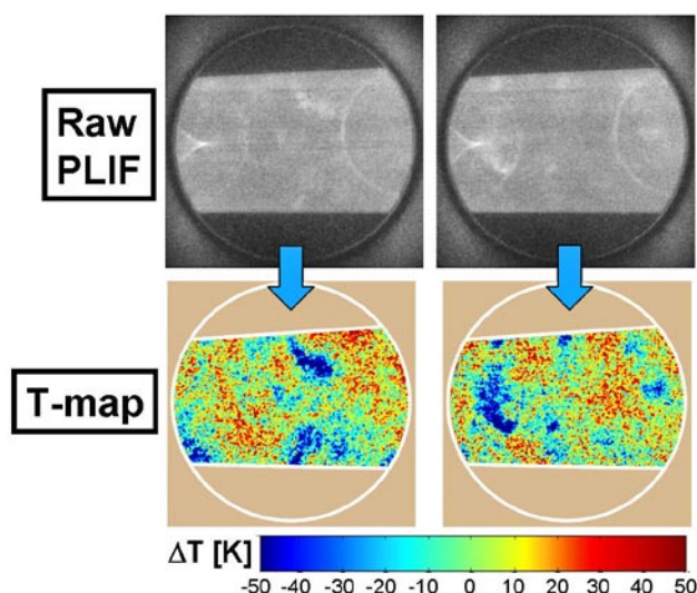
FIGURE 2. Conversion of raw toluene PLIF images to temperature maps.
