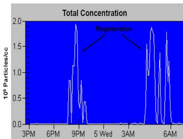
FIGURE 1. Real-Time Particle Number Concentrations in Inhalation Chamber during 16-hr Cycle
