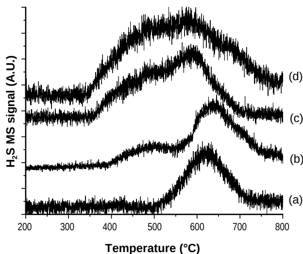
FIGURE 1. \text{H}_2 TRPX spectra of Pt-BaO(20)/ \text{Al}_2\text{O}_3 and Pt-BaO(8)/ \text{Al}_2\text{O}_3 in the absence of \text{CO}_2 (a and c) and in the presence of \text{CO}_2 (b and d).
