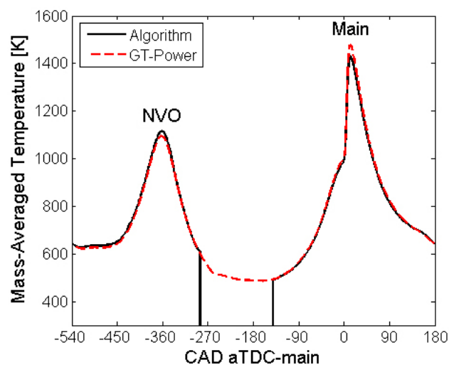
FIGURE 2. Computed (algorithm) and modeled (GT-Power) temperature traces for a typical low-load main-fuel experiment. The same comparison could not be made for an NVO-fuel test because of limitations of GT-Power. As in all report figures, the main fuel injection is 7.9 mg/cycle of iso-octane, and the symmetric (negative) valve overlap is 150 CAD.
