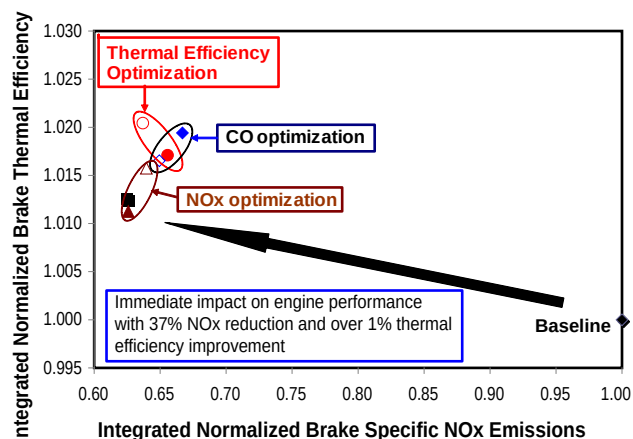
FIGURE 4. Controller Optimization over Transient Cycle
