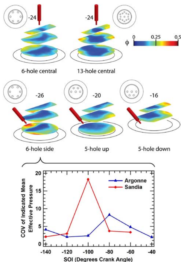
FIGURE 3. Top: Fuel distribution towards the end of the compression stroke for five different injector configurations with intermediately retarded injection ( \text{SOI} = -80^\circ\text{CA} ). Images were taken at maximum break-torque spark timing (crank angle indicated above each image stack) as determined in the fired metal engine at ANL. Bottom: Coefficient of variation (COV) for the 6-hole injector in side location as a function of injection timing. Measurements in Sandia’s optical engine and ANL’s metal engine are shown. Operating conditions as for Figure 2.
