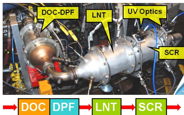
FIGURE 1. Picture and schematic of the LNT+SCR catalyst system on the light-duty diesel engine.
