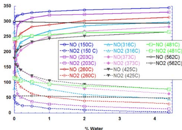
FIGURE 4. Effect of \text{H}_2\text{O} on NO oxidation as a function of temperature and \text{H}_2\text{O} concentration. Feed gas: NO of 350 ppm, 14% \text{O}_2 , 5% \text{CO}_2 .
