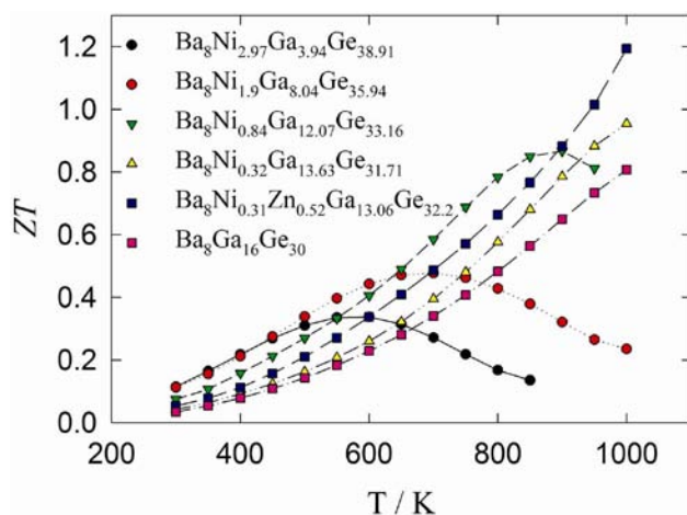
FIGURE 4. Temperature Dependence of the TE Figure of Merit ZT for TM-Substituted \text{Ba}_8\text{Ga}_{16}\text{Ge}_{30}
