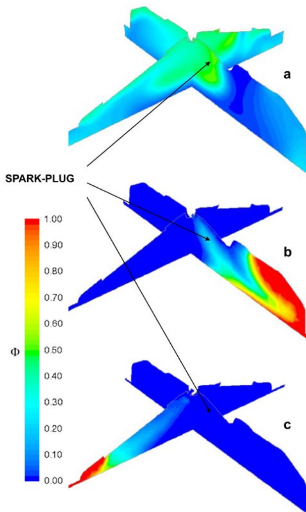
FIGURE 2. Simulated equivalence ratio ( \Phi ) at maximum brake torque (MBT) spark timing for: a) Injection angle of 0^\circ and \text{SOI} = -140^\circ\text{CA} ( \text{MBT} = -23^\circ\text{CA} ); b) Injection angle of 0^\circ and \text{SOI} = -40^\circ\text{CA} ( \text{MBT} = -8^\circ\text{CA} ); c) Injection angle of 90^\circ and \text{SOI} = -40^\circ\text{CA} ( \text{MBT} = \text{TDC} )
