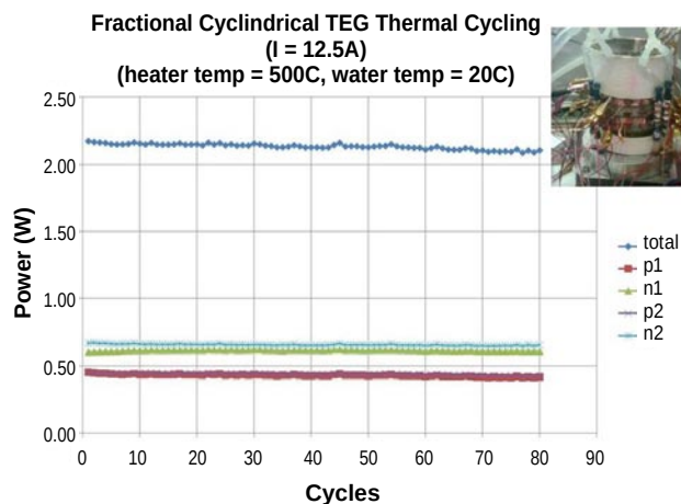
FIGURE 4. Fractional TEG Test Results
