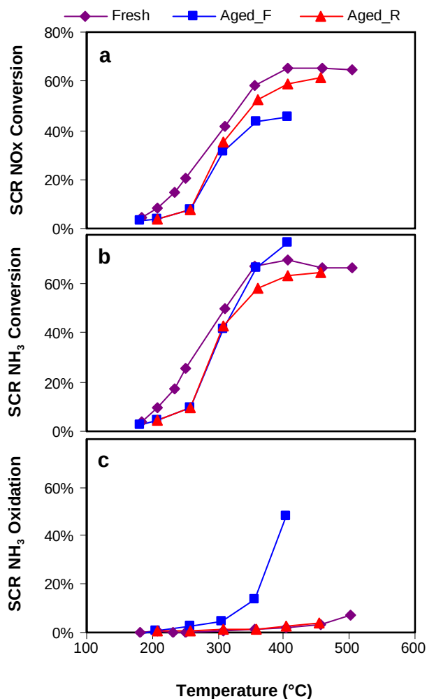
FIGURE 6. (a) SCR NOx conversion, (b) SCR \text{NH}_3 conversion, and (c) \text{NH}_3 oxidation conversion as a function of temperature for fresh (Fresh), front face of aged brick (Aged_F), and rear face of aged brick (Aged_R) SCR catalyst core samples.
