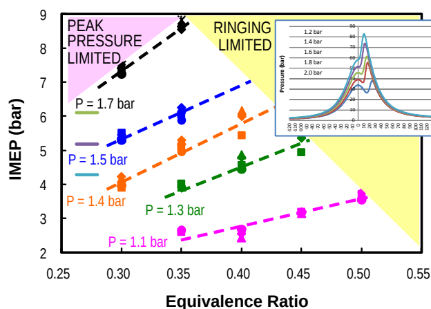
FIGURE 2. Extended high-load LTC operation achieved by leaning the mixture along with boosting to maintain acceptable R.I. values below \sim 5.0 \text{ MW/m}^2
