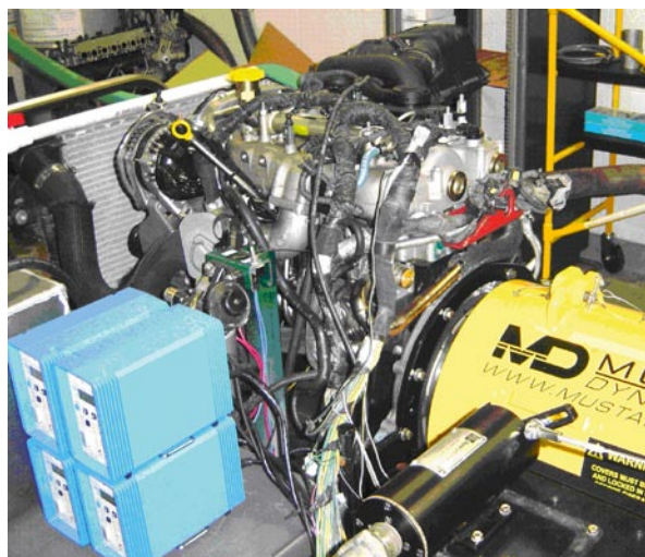
Wayne State University Engine Test Setup
