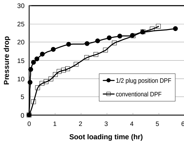
FIGURE 2. Effects of Soot Loading on Pressure Drop
