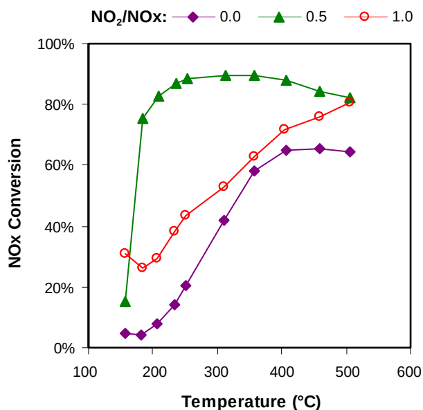
FIGURE 1. SCR \text{NO}_x conversion as a function of temperature for \text{NO}_2/\text{NO}_x ratios of 0.0, 0.5, and 1.0. Data collected with a fresh catalyst sample operated at a GHSV of 120,000 \text{hr}^{-1} under 300 ppm \text{NO} , stoichiometric quantities of \text{NO}_x (300 ppm \text{NO} , 150 ppm \text{NO} + 150 ppm \text{NO}_2 , and 225 ppm \text{NO}_2 , respectively), 10% \text{O}_2 , 5% \text{H}_2\text{O} , and 5% \text{CO}_2 .
