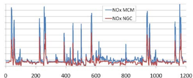
FIGURE 5. Comparison of Federal Test Procedure NO x Emissions for Baseline Control and Next Generation Controller (NGC)
