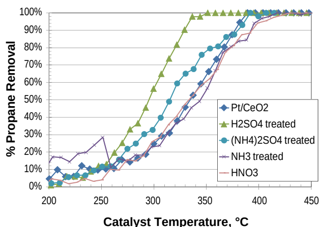
FIGURE 6. Effect of pretreatment on the propane activity of the 2\%\text{Pt}/\text{Ce}_{0.9}\text{Pr}_{0.1}\text{O}_2 catalyst.
