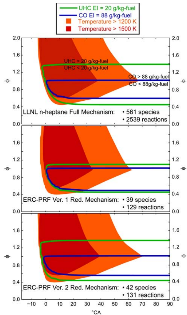
FIGURE 3. CO and UHC yield and gas temperature as a function of equivalence ratio and crank angle. Reduced mechanisms can result in a significant narrowing of the equivalence ratio band within which low UHC emissions are predicted. As shown in the bottom figure, this shortcoming can be remedied without adding significant complexity.
