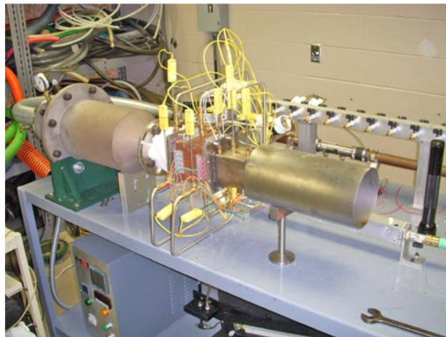
FIGURE 2. System Consisting of a Heater, Cooling System and Electrical Components used for Testing a TEG
