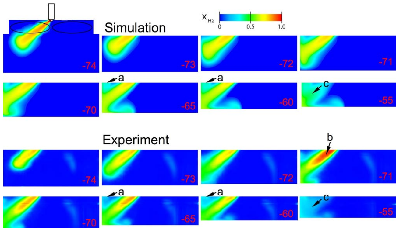
FIGURE 4. Experimental/numerical comparison of the mean fuel mole-fraction fields for injection from a single-hole injector for SOI = -80°C. The field of view spans the whole width of the cylinder bore and the height from piston top to just below the fire deck, but not the pent-roof combustion chamber. Features designated by arrows and letters are referred to in the text. Operating conditions as for Figure 2.
