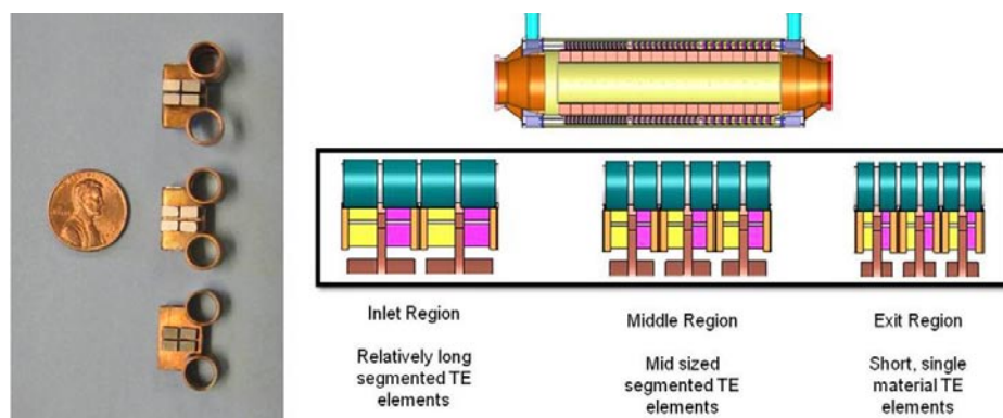
FIGURE 2. TE Subassemblies Optimized for Performance in the Direction of Gas Flow
