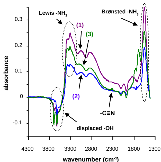
FIGURE 4. DRIFT spectra of the CLEERS reference Fe zeolite urea SCR catalyst at 200°C under (1) 350 ppm \text{NH}_3 , 14% \text{O}_2 , 4.5% \text{H}_2\text{O} , 5% \text{CO}_2 , (2) 350 ppm \text{NO} , 350 ppm \text{NH}_3 , 14% \text{O}_2 , 4.5% \text{H}_2\text{O} , 5% \text{CO}_2 , and (3) 50 ppm toluene, 350 ppm \text{NO} , 350 ppm \text{NH}_3 , 14% \text{O}_2 , 4.5% \text{H}_2\text{O} , 5% \text{CO}_2 . (background spectrum: 14% \text{O}_2 , 4.5% \text{H}_2\text{O} , 5% \text{CO}_2 )
