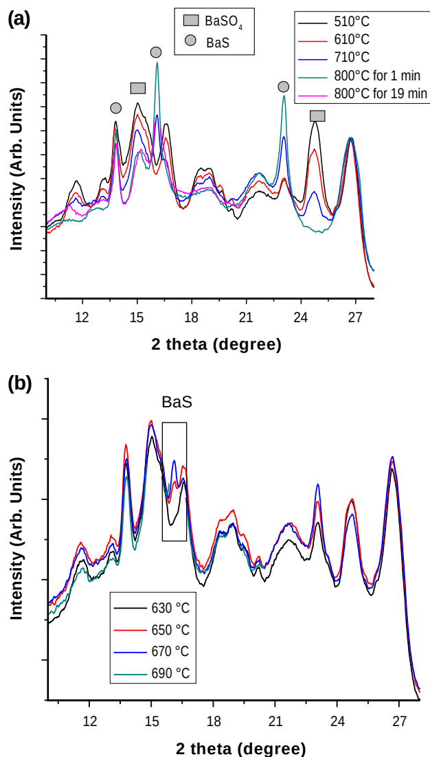
FIGURE 2. TR-XRD diffractograms of pre-sulfated Pt-BaO(20)/ \text{Al}_2\text{O}_3 obtained during the temperature ramping in the presence of both \text{H}_2 and \text{CO}_2 . Figure 2(a) and 2(b) plot the XRD data for temperature ranges of 510 – 800^\circ\text{C} and 630 – 690^\circ\text{C} , respectively.
