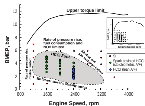
Operating Limits Explored to Date with the Multi-Cylinder Engine. (Wagner, ORNL)
