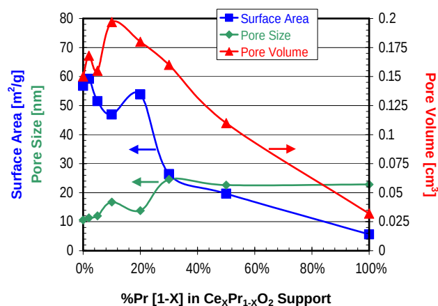
FIGURE 2. Summary of BET results presented as total surface area, average pore size, and total pore volume for 2%Pd/ \text{Ce}_x\text{Pr}_{1-x}\text{O}_2 where x = 1, 0.98, 0.95, 0.9, 0.8, 0.7, 0.5 , and 0.
