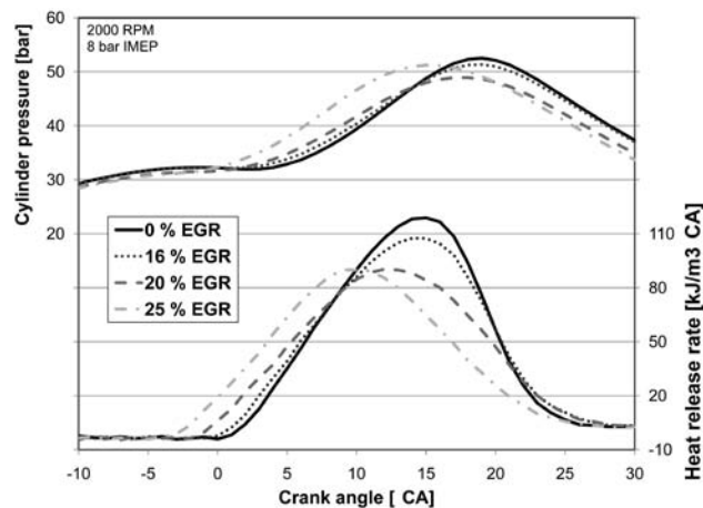
FIGURE 5. Influence of EGR on pressure traces and heat release rates at high engine load.
