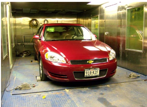
FIGURE 2. Light-duty “normal” emitter tested in the CLOSE Project, a 2006 Chevrolet Impala.
