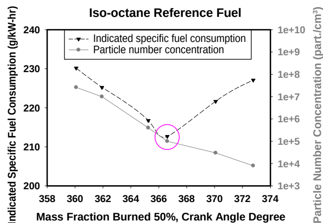
FIGURE 4. HCCI engine cycle timing for minimum fuel consumption (black) and particle number concentration emissions for each operating point (grey). The operating point for simultaneous low emissions and fuel consumption is circled (pink). (Engine conditions: 1,800 rpm, nominal 3.0 indicated mean effective pressure)
