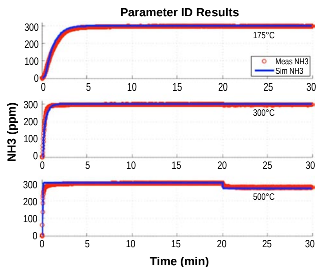
FIGURE 5. Comparison between measured and simulated \text{NH}_3 concentration profiles during the \text{NH}_3 adsorption and oxidation steps of the transient SCR catalyst evaluation protocol run at 175, 300, and 500°C and a GHSV of 90,000 \text{hr}^{-1} .
