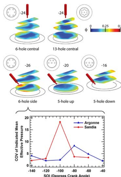
Top: Hydrogen distribution towards the end of the compression stroke for five different injector configurations with intermediately retarded injection (SOI = -80°CA). Bottom: Coefficient of variation for the 6-hole injector in side location as a function of injection timing. (Kaiser, SNL)
