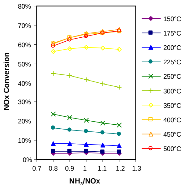
FIGURE 2. SCR \text{NO}_x conversion as a function of \text{NH}_3/\text{NO}_x ratio at various operating temperatures. Data collected with a fresh catalyst sample operated at a GHSV of 120,000 \text{hr}^{-1} under 300 ppm \text{NO} , 10% \text{O}_2 , 5% \text{H}_2\text{O} , and 5% \text{CO}_2 .
