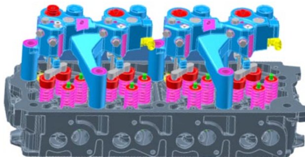
FIGURE 1. VVA System on Cylinder Head
