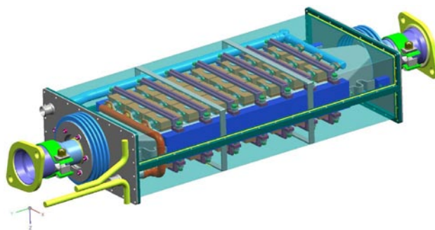
FIGURE 1. Side View of the TE Generator Design
