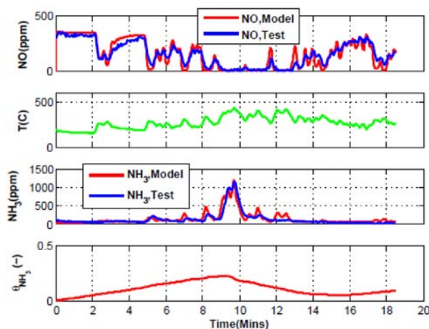
FIGURE 3. Standard SCR kinetic model validation on a thermal transient micro-reactor. Feed gas: 350 ppm \text{NO}_x , 350 ppm \text{NH}_3 , 14% \text{O}_2 , 5% \text{CO}_2 , 2.5-5% \text{H}_2\text{O} and the balance \text{N}_2 .
