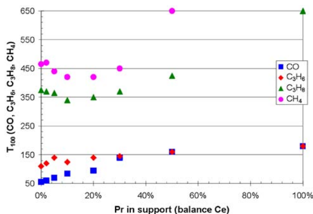
FIGURE 1. Summary of T_{100} temperatures at 240 L/(g-hr) space velocity for CO, \text{C}_3\text{H}_6 , \text{C}_3\text{H}_8 , and \text{CH}_4 on 2%Pd/ \text{Ce}_x\text{Pr}_{1-x}\text{O}_2 where x = 1, 0.98, 0.95, 0.9, 0.8, 0.7, 0.5 , and 0.
