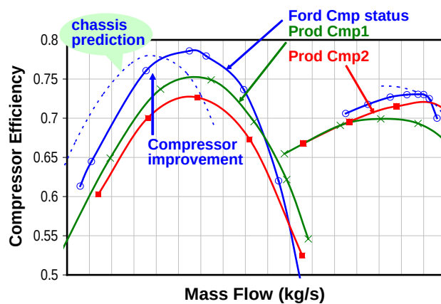
FIGURE 3. Compressor Efficiency, CFD vs. Flow Bench Test at 70,000 RPM
