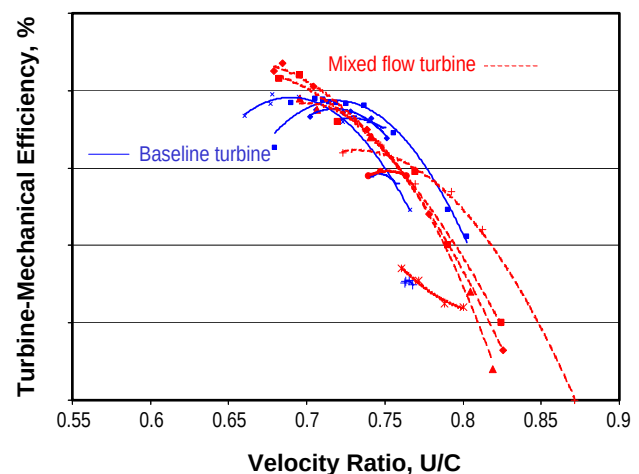
FIGURE 2. Gas Stand Result – Mixed Flow Turbine Stage
