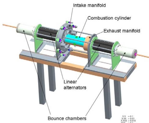
FIGURE 2. The HFPE Research Prototype Computer-Aided Design Model
