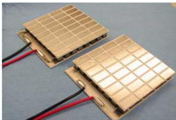
FIGURE 2. Prototype PbTe Modules
