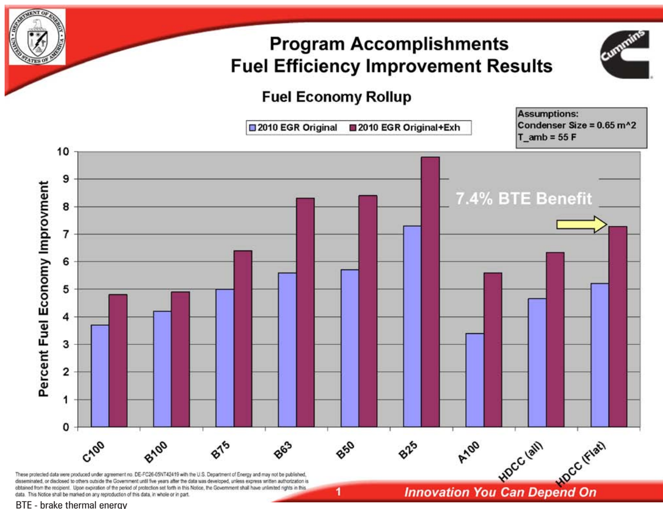
FIGURE 1. Performance of the First-Generation Cummins ISX-Based ORC Energy Recovery System
