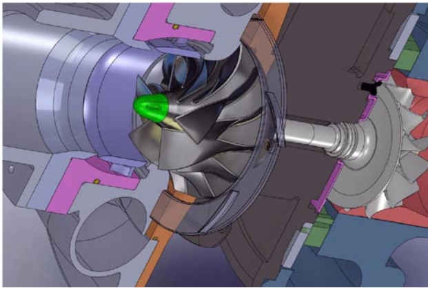
FIGURE 2. Turbocharger Assembly
