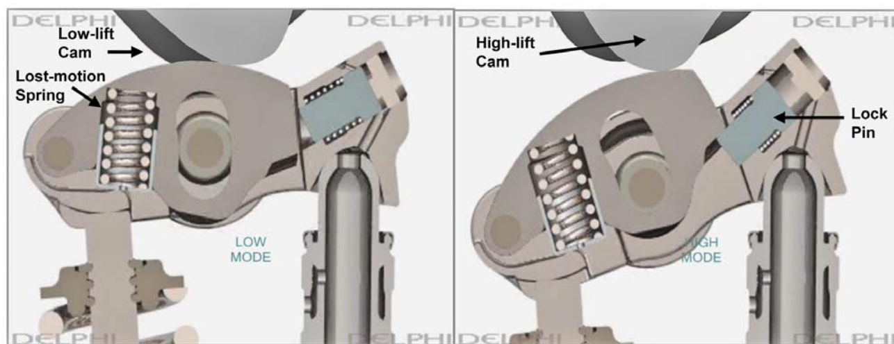
FIGURE 3. Schematic of Delphi Two-Step Valve-Lift Mechanism [1]
