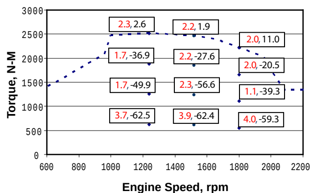
FIGURE 6. Piston Optimization [%BSFC (Red), %Smoke (Black) – Positive numbers indicate increase]
