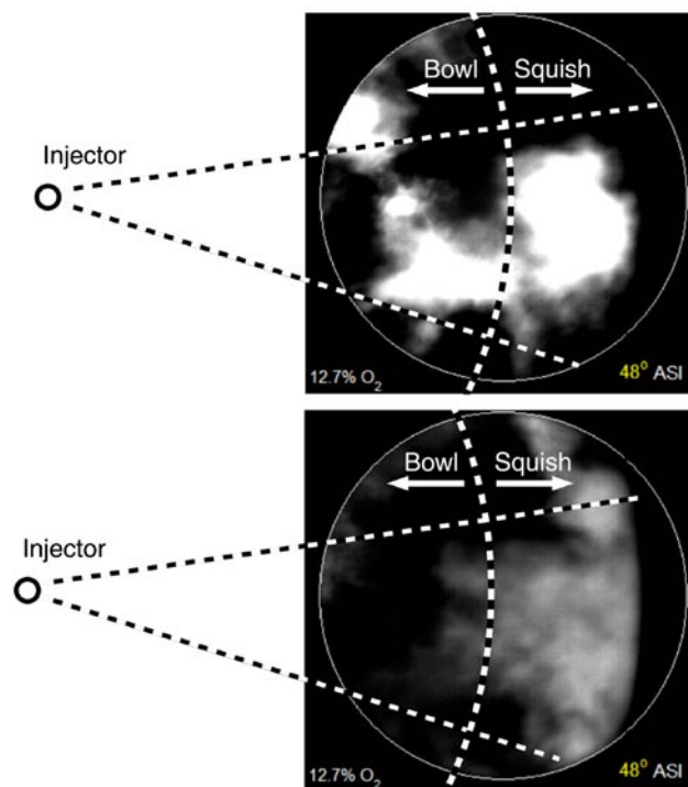
FIGURE 4. Soot luminosity images in the squish region above the piston for a main-injection only (top) and with a post injection (bottom) acquired through the cylinder head window (see Figure 1). A portion of one of the eight jets is visible and the injector is to the left, outside of the field of view, as indicated by the straight dashed lines. The curved dashed lines show the contour of the piston bowl, with the squish region on the right.
