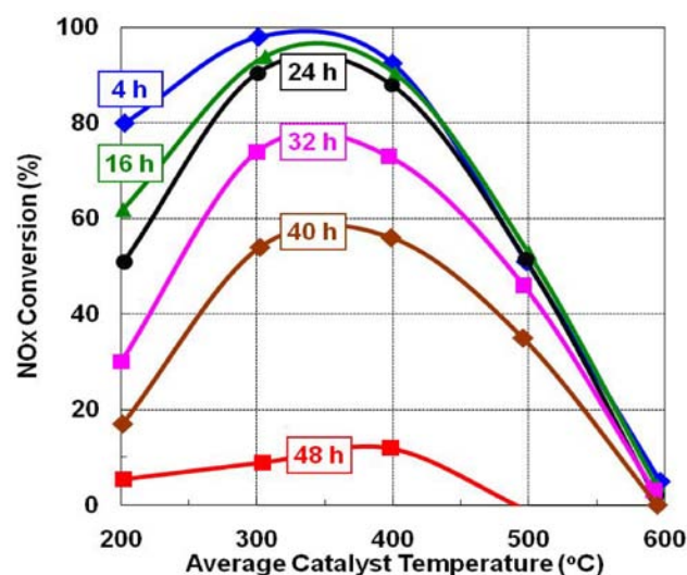
FIGURE 4. Changes in NOx Conversion over Aged Urea-SCR Catalysts as a Function of Aging Time
