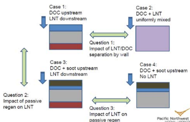
FIGURE 2. 1-D Micro-Modeling Cases
