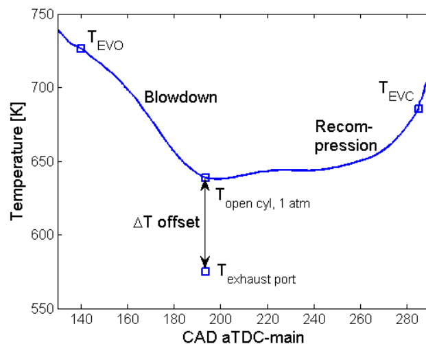
FIGURE 1. Initial steps of algorithm for computing cycle temperatures from measured cylinder pressures. Temperatures are shown for the open portion of the cycle between EVO and EVC.
