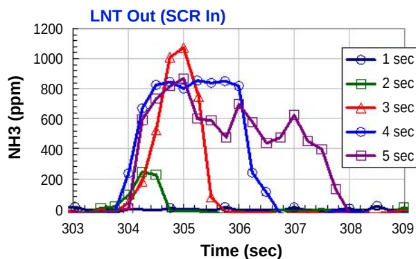
FIGURE 3. NH 3 vs. time at the LNT-out position as a function of the rich duration of the LNT regeneration event.
