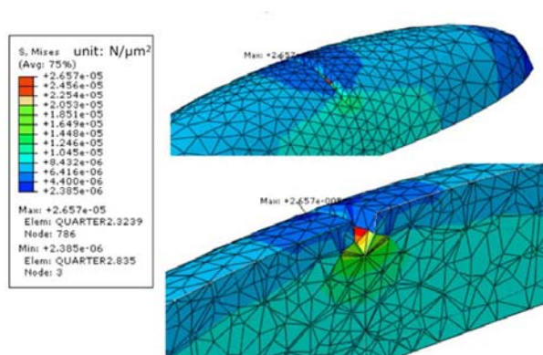
Figure V- 106: Stress Distribution in Cathode Model and Opening of a Pre-existing Crack
