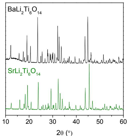
Figure IV- 30: X-ray diffraction powder patterns of \text{MLi}_2\text{Ti}_6\text{O}_{14} prepared by sol-gel method.
