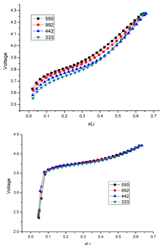
Figure V- 25: Open circuit voltages on (top) charging and (bottom) discharging \text{Li}_{1-x}\text{Ni}_y\text{Mn}_y\text{Co}_{1-2y}\text{O}_2 , where the composition is represented by the y y 1-2 y notation in the graphs (for y=0.45 , the notation is 992).
