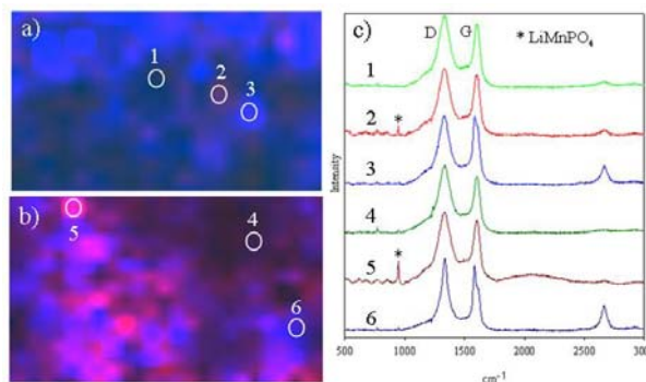
Figure V- 62: Raman images of \text{LiMnPO}_4 electrodes before (a) and after (b) \text{O}_2 -plasma etching. Blue areas correspond to carbon additives, red areas represent \text{LiMnPO}_4 . Selected Raman spectra are shown in (c).
