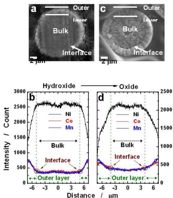
Figure IV- 42: Scanning electron microscopy (SEM) and electron-probe X-ray micro-analysis (EPMA) results; (a) SEM photograph and (b) EPMA line scan of precursor hydroxide; (c) SEM photograph and (d) EPMA line scan of the final lithiated oxide \text{Li}[\text{Ni}_{0.64}\text{Co}_{0.18}\text{Mn}_{0.18}]\text{O}_2 . In both cases, the gradual-concentration changes of Ni, Mn, and Co in the interlayer are clearly evident. The nickel concentration decreases and the Co and Mn concentrations increase toward the surface.
