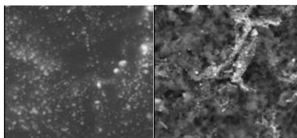
Figure IV- 26: Fate of a lithium metal electrode coated with Li 4 Sn -VEC composite coatings. Initial coating (left) shows good dispersion of nanoscale Li 4 Sn clusters within the VEC matrix. After 200 cycles (right) particles have moved away from lithium metal surface into dendritic layer, concentrating on the top of electrode.
