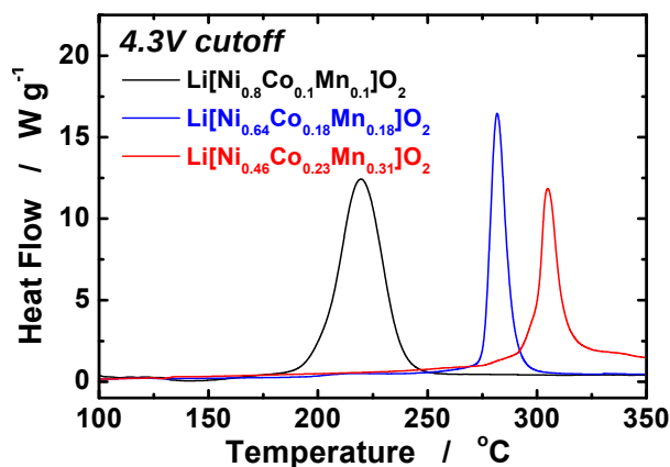
Figure IV- 44: DSC traces showing heat flow from the reaction of the electrolyte with \text{Li}_{1-\delta}[\text{Ni}_{0.8}\text{Co}_{0.1}\text{Mn}_{0.1}]\text{O}_2 , gradient material \text{Li}_{1-\delta}[\text{Ni}_{0.64}\text{Co}_{0.18}\text{Mn}_{0.18}]\text{O}_2 , and \text{Li}_{1-\delta}[\text{Ni}_{0.46}\text{Co}_{0.23}\text{Mn}_{0.31}]\text{O}_2 charged to 4.3 V.
