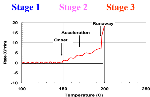
Figure III-71: Cell heating rate during thermal ramp showing three stages of thermal runaway leading to explosive loss of the cell.
