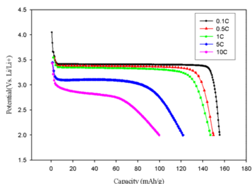
Figure V- 26: Discharge curves of \text{LiFePO}_{0.95}\text{V}_{0.05}\text{O}_4 at different rates showing the high rate capability.
