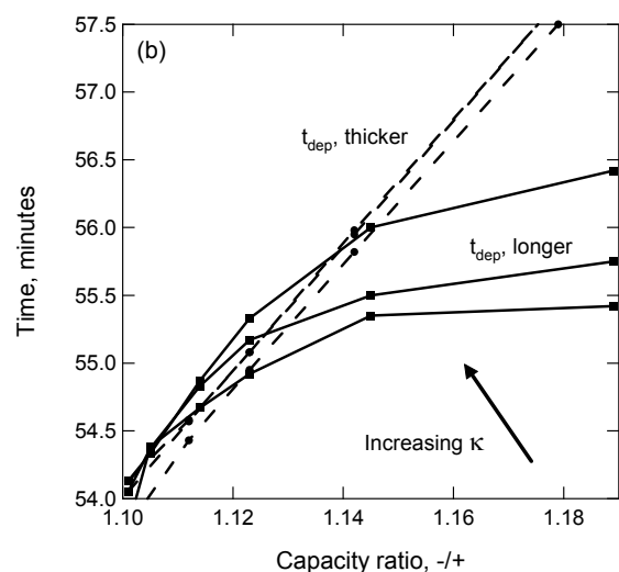
Figure V- 117: (a) Time to reach deposition ( t_{dep} , solid lines) and cutoff potential ( t_{vcut} , dashed lines) as the electrode is extended, for K_{eff} = 0.33 , 0.533 (baseline), and 1.3 \text{ S m}^{-1} . (b) Time to reach deposition as electrode is either extended (solid lines) or thickened (dashed lines), for the same values of K_{eff} . As the conductivity increases, there is less ohmic resistance through the separator to the extension and thus extending the electrode becomes more effective at preventing deposition. Neither the time to reach the cutoff potential nor the time to reach deposition is strongly affected when the electrode is made thicker.
