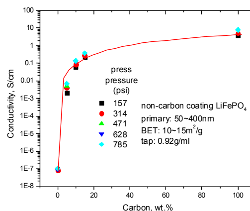
Figure IV- 13: Carbon Additive Effect on Conductivity of \text{LiFePO}_4 /Carbon Blend
