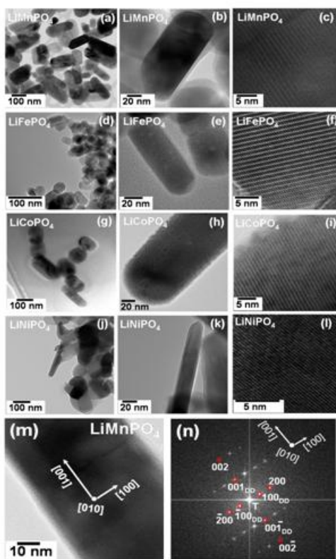
Figure V- 22: TEM images of olivine \text{LiMPO}_4 ( M = \text{Mn, Fe, Co, Ni} ) prepared by the MW-ST method.
