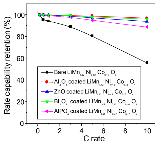
Figure V- 21: Rate capability retention of bare and surface modified \text{LiMn}_{1.42}\text{Ni}_{0.42}\text{Co}_{0.16}\text{O}_4 cathodes after 50 cycles
