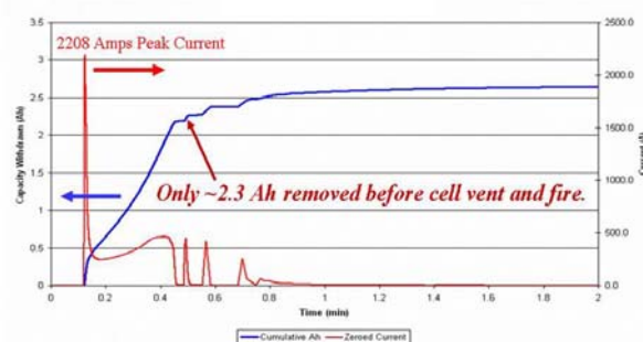
Figure III-66: Current and integrated capacity profiles for 12 cell pack during hard short circuit test showing cascade failure of the cells.
