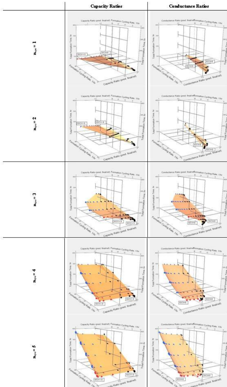
Figure IV- 93: Surface plots of capacity (left column) and conductance (right column) ratios (predicted final to referent) plotted against total formation time and formation cycling rate for all to_{cv} and for each total number of formation cycles ( n_{\text{cyc}} ).
