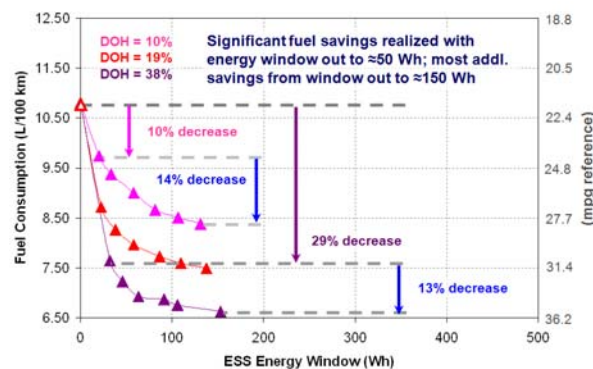
Figure III-51: Simulation Results over the Urban Dynamometer Driving Schedule (UDDS) Driving Cycle
