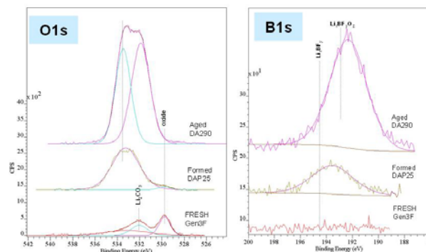
Figure IV- 74: O1s and B1s XPS data from fresh, formed and aged (4V, 38 wks at 55°C) pouch cells show significant differences.
