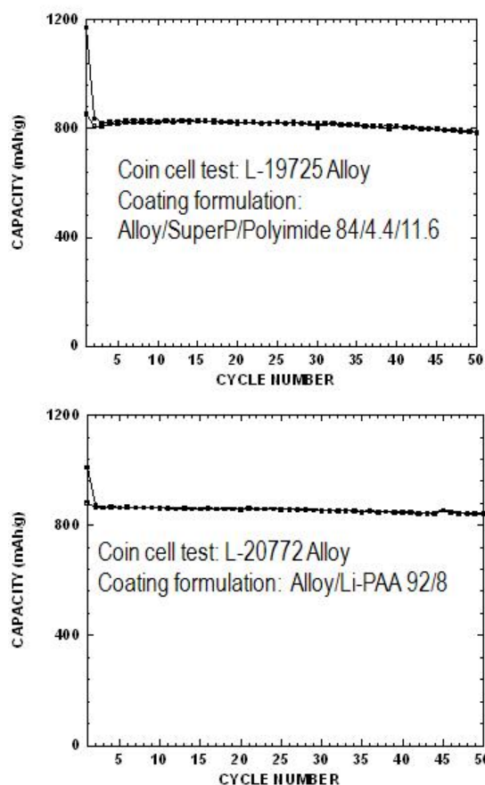
Figure III-24: Coin cell cycling tests of L-19725 and L-20772 alloys chosen for development in this project. Coin cells were cycled between 5 mV and 0.9 V at a rate of C/4.
