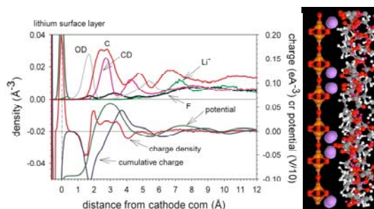
Figure V-91: Atom density profile charge density and electrostatic potential near the LiFePO 4 cathode in an EC/DMC electrolyte. Figure on the right shows the electrolyte structure near the cathode/electrolyte interface.
