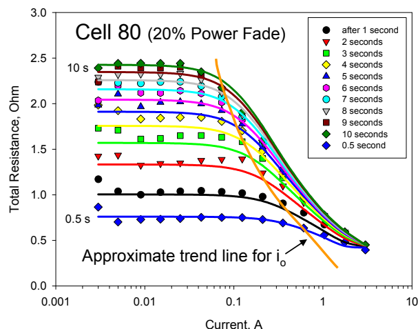
Figure IV- 94: Total impedance at -30^{\circ}\text{C} over pulse timeline for Cell 80 under discharge conditions. The symbols represent data and the solid lines represent model results.
