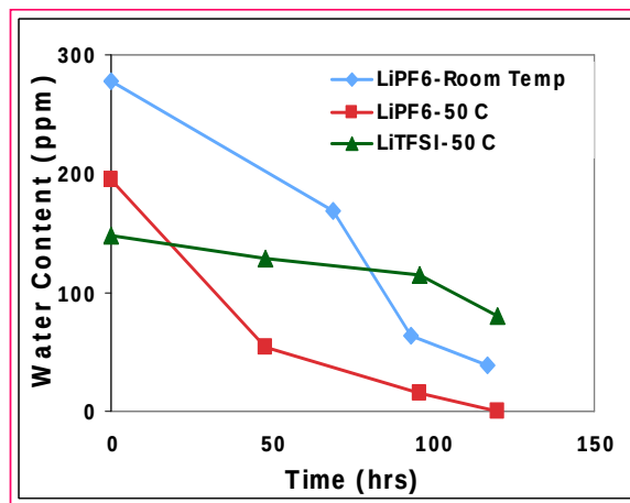
Figure V- 87: K-F titration measures of water content of EC/EMC solutions of \text{LiPF}_6 and \text{LiTFSI} over time at different temperatures.
