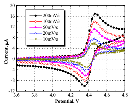
Figure IV- 113: CV of 10 mM 2-(pentafluorophenyl)-tetrafluoro-1,3,2-benzodioxaborole and 1.2 M \text{LiPF}_6 in EC/PC/DMC (1:1:3) in tests using a Pt/Li three-electrode electrochemical cell.
