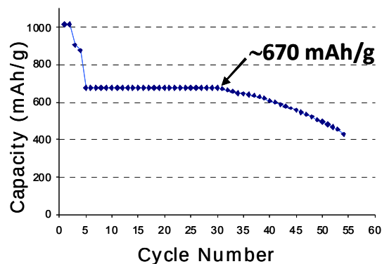
Figure V- 71: Discharge capacity vs. cycle number of a Li/ \text{Cu}_6\text{Sn}_5 -Sn, Cu-foam coin cell.
