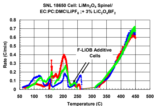
Figure IV- 129: ARC profiles of 18650 cells with \text{LiMn}_2\text{O}_4 cathodes both with and without F-LiOB electrolyte additive showing only slight low-temperature improvement.
