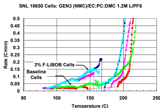
Figure IV- 131: ARC profiles of 18650 cells with \text{LiNi}_{1/3}\text{Co}_{1/3}\text{Mn}_{1/3}\text{O}_2 cathodes both with and without F-LiOB electrolyte additive showing increased reaction rate at low-temperatures.
