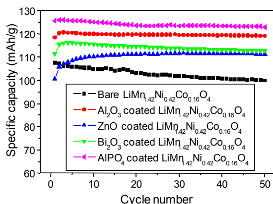
Figure V- 20: Cycling performances of the bare and 2 wt. % \text{Al}_2\text{O}_3 , \text{ZnO} , \text{Bi}_2\text{O}_3 , and \text{AlPO}_4 coated \text{LiMn}_{1.42}\text{Ni}_{0.42}\text{Co}_{0.16}\text{O}_4 .
