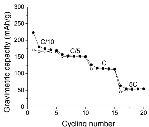
Figure IV- 19: Rate capability of TiO 2 brookite.
