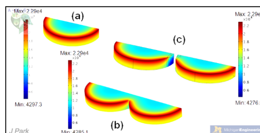
Figure V- 111: Lithium-ion concentration distribution ( \text{mol/m}^3 ) when the surface concentration reaches the stoichiometric maximum value ( 2.29\text{e}4\text{ mol/m}^3 )
