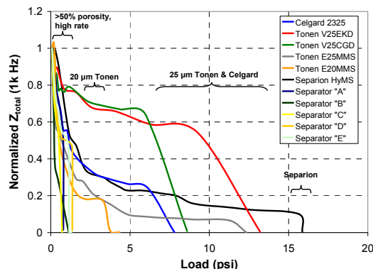
Figure IV- 139: Normalized total impedance (50 mV, 1000 Hz) as a function of applied load to commercial separators punctured with 425 \mu\text{m} copper particles.
