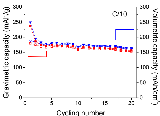
Figure IV- 18: Cycle-ability of TiO 2 brookite performed at C/10 (33.5 mA/g) as function of the gravimetric and volumetric capacity. Empty symbols refer to the charge; filled symbols, to the discharge.
