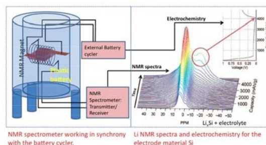
Figure V- 2: A schematic showing the in situ NMR set-up and a 7Li NMR spectrum acquired on the 1st discharge of a Si/Li battery.
