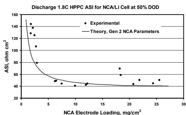
Figure IV- 68: NCA positive electrode loading study: half-cell experimental impedance compares favorably to electrochemical model with Gen 2 electrode parameters
