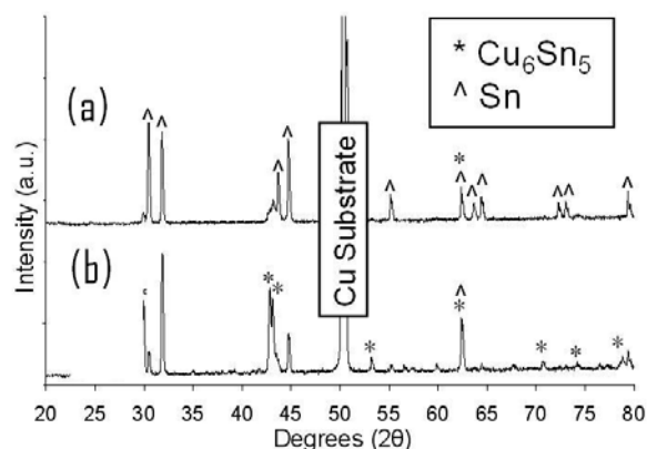
Figure V- 69: XRD patterns of (a) electrodeposited \text{Cu}_6\text{Sn}_5 -Sn product (as-grown) on Cu foil; (b) after annealing at 150^\circ\text{C}
