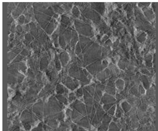
Figure V- 124: Lateral midsection of a 0.4mm Toray sheet with xx % weight loading of \text{LiFePO}_4 as viewed using X-ray tomography. For scale, fibers are 8 \mu\text{m} in diameter.
