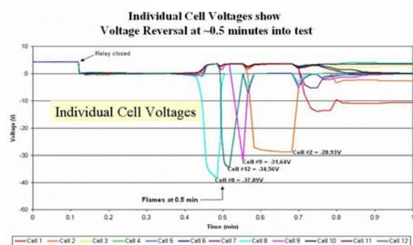
Figure III-65: Voltage profile for 12 cell pack during hard short circuit test showing cascade failure of the cells.
