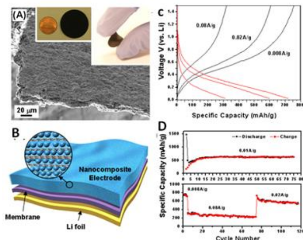
Figure V- 76: (A) Side-view SEM image of a self-assembled free-standing \text{SnO}_2 -graphene nanocomposite (40 wt% graphene sheets) electrode 15- \mu\text{m} thick. Photographs in the insert show a disk-like 3-cm-diameter \text{SnO}_2 -graphene nanocomposite electrode on the left and a folded electrode on the right. (B) A Li-ion battery configuration directly using a free-standing metal oxide-graphene nanocomposite film as an electrode. The graphene sheets in the layered nanostructures functions as both current collector and conductive additives in the anode. (C) Charge/discharge profiles of a \text{SnO}_2 -graphene nanocomposite electrode (40 wt% graphene sheets) between 0.02 V and 1.5 V at a current density of 0.008 A/g, 0.02 A/g and 0.08 A/g, respectively. (D) Top: Specific capacity of \text{SnO}_2 as a function of charge/discharge cycles in the \text{SnO}_2 -graphene nanocomposite electrode at a current density of 0.01 A/g. Bottom: Specific capacity of \text{SnO}_2 as a function of charge/discharge cycles in the \text{SnO}_2 -graphene nanocomposite at different charge/discharge current densities of 0.008 A/g, 0.08 A/g and 0.02 A/g, respectively.
