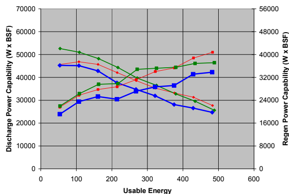
Figure III-12: HPPC Data of (RED, middle crossing point)-CD-size Cell (BLUE, bottom-most crossing point)-Initial A5 cells, (GREEN, top most cross point) Final A5 Cells
