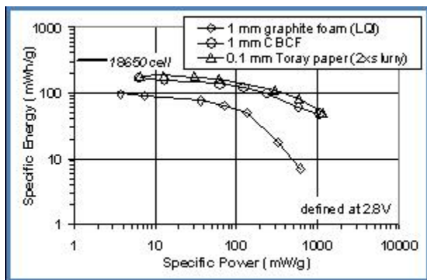
Figure V- 122: Specific energy and power performance for several composite cathodes. The mass includes the carbon current collector, \text{LiFePO}_4 and carbon binder.
