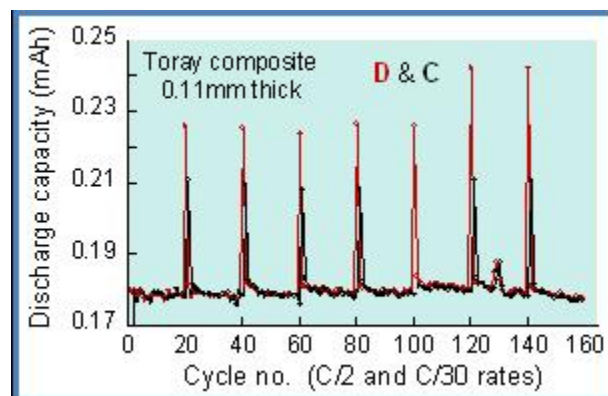
Figure V- 123: Discharge and charge capacity for 0.7 \text{cm}^2 disk with C/2 rates with a slow C/30 every 20 cycles.
