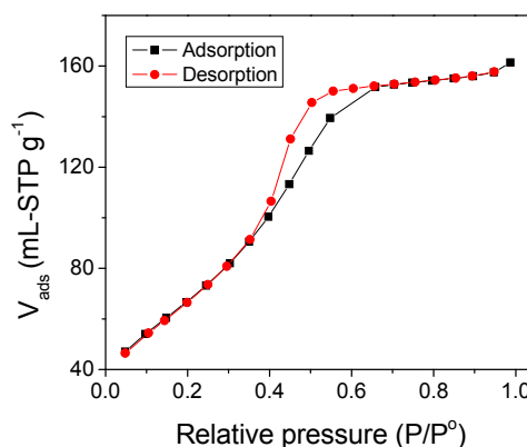
Figure IV- 17: \text{N}_2 adsorption isotherms of \text{TiO}_2 brookite.
