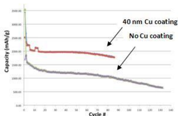
Figure V- 116: Cycling of silicon thin films with and without a copper coating. Note the lowered capacity loss and better efficiency with a 40nm copper coating.
