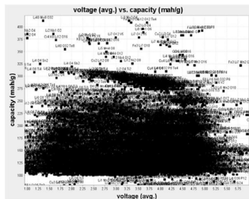
Figure V- 6: Capacity vs. voltage for thousands of compounds (calculated).
