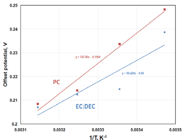
Figure V- 114: Offset potential measured between lithiation and delithiation potentials vs. \text{Li/Li}^+ at 50% state-of-charge is measured as a function of temperature.
