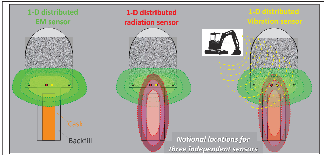
Figure 1. Illustration of three independent 1-dimensional distributed sensors with notional locations.
