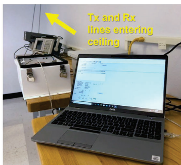
Figure 6. Photographs of the PCC system on the lab bench with transmitting and receiving lines.
