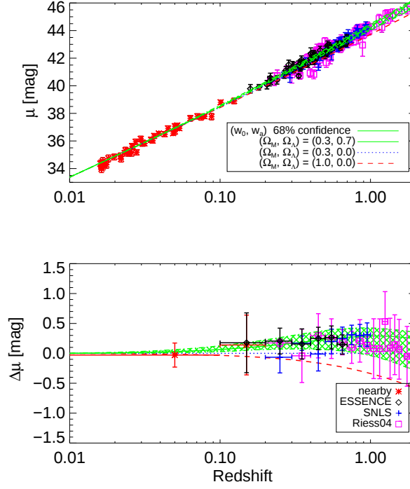
Figure 6: SN Ia results: ESSENCE (diamonds), SNLS (crosses), low-redshift SNe (*), and the compilation of Riess et al. (2004) which includes many of the other published SN distances plus those from HST (squares). Upper : distance modulus vs. redshift measurements shown with three cosmological models: \Omega_M = 0.3 , \Omega_\Lambda = 0 (dotted); \Omega_M = 1 , \Omega_\Lambda = 0 (dashed); and the 68% CL allowed region in the w_0 - w_a plane, assuming spatial flatness and a prior of \Omega_M = 0.27 \pm 0.03 (hatched). Lower : binned distance modulus residuals from the \Omega_M = 0.3 , \Omega_\Lambda = 0 model. Adapted from Wood-Vasey et al. (2007).
