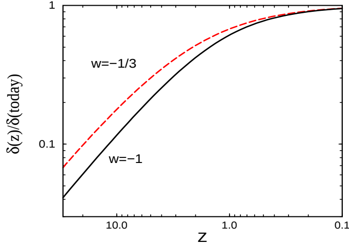
Figure 3: Growth of linear density perturbations in a flat universe with dark energy. Note that the growth of perturbations ceases when dark energy begins to dominate, 1+z = (\Omega_M/\Omega_{DE})^{1/3w} .
