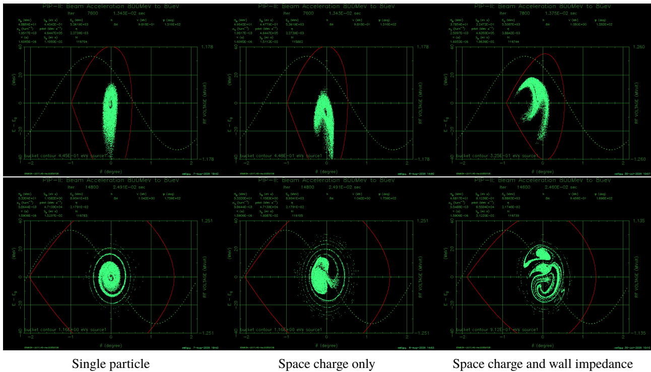
Figure 3: Effect of the space charge and wall impedance. Top: Phase space very shortly after crossing transition. Bottom: Phase space at the end of acceleration.
