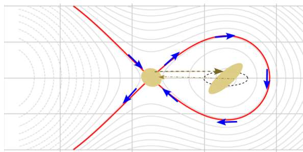
Figure 2: The triple phase jump principle. The bunch is first rotated and then moved to an unstable (saddle) fixed point. Particles are attracted along one of the perpendicular separatrices and repelled along the other, modifying the bunch aspect ratio to achieve a better match.
