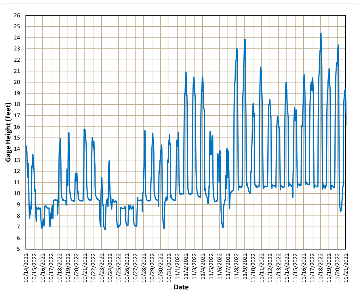
Figure 4. Gauge Height Changes at USGS 12472800 Columbia River Below Priest Rapids Dam During the Fall Chinook Salmon Spawning Period in Calendar Year 2022 (USGS 2023)
