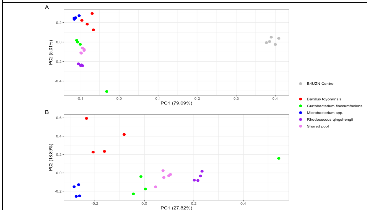
Fig. 10. Principle Component Analysis (PCA) plot illustrating metabolite expression between CSC-A members with B4UZN control media (A), and without control B4UZN media (B) for contrast. The stark difference in variance
