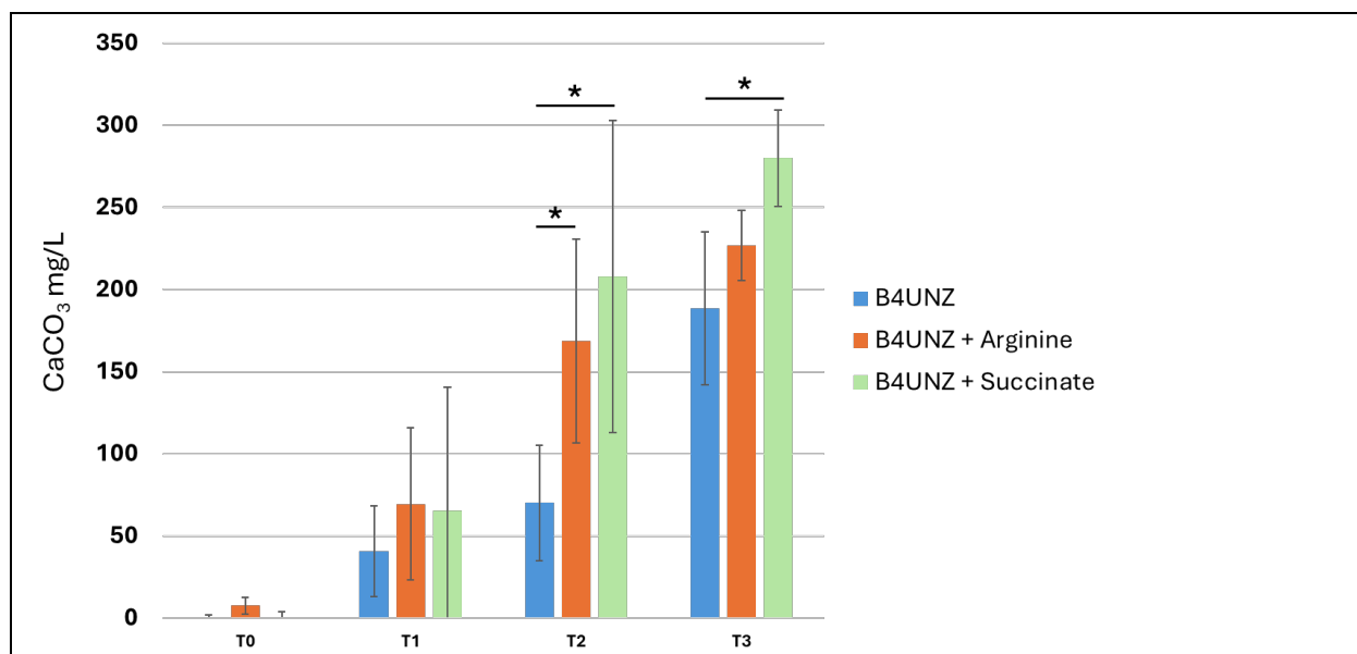
Fig. 12. Production of CaCO 3 by CSC-A during cultivation with added metabolites. Amount of CaCO 3 is shown in the y-axis and timepoints (T0 = 0 hours, T1 = 24 hours, T2 = 48 hours, T3 = 72 hours) are shown on the x-axis. * indicate p-values less than 0.05.
