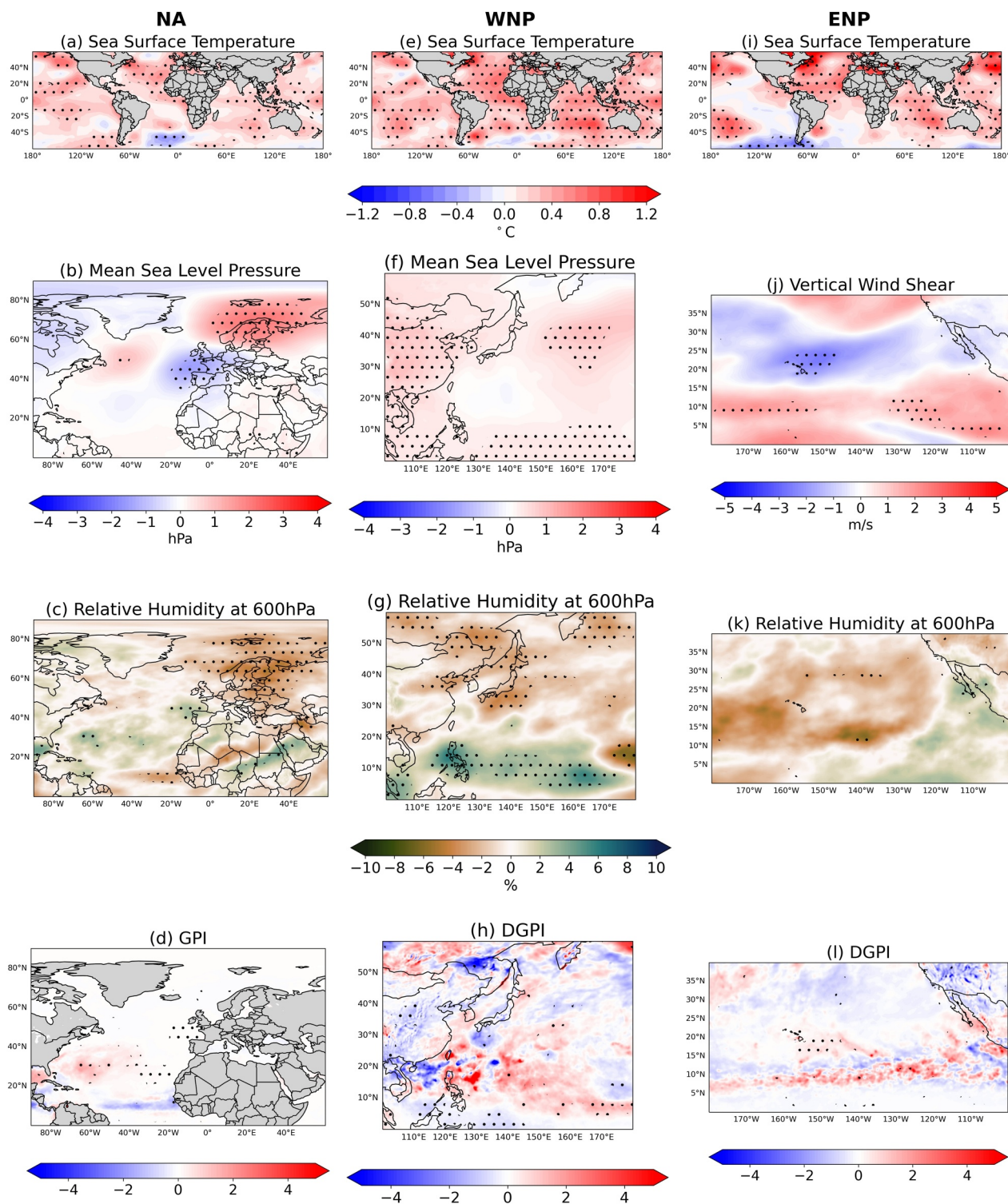
Figure 4. Difference between ASO-averaged environmental variables composited during years with strong minus weak ENSO-TC teleconnections, calculated for the North Atlantic for (a) SST ( ^{\circ}\text{C} ), (b) mean sea-level pressure (hPa), (c) relative humidity at 600 hPa (%), and (d) GPI; In the WNP for (e) SST ( ^{\circ}\text{C} ), (f) sea-level pressure (hPa), and (g) 600 hPa relative humidity (%), (h) DGPI; and in the ENP for (i) SST ( ^{\circ}\text{C} ), (j) VWS ( \text{ms}^{-1} ), (k) 600 hPa relative humidity (%), and (l) DGPI. Dots represent significant anomalies at the 95% confidence interval.
