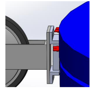
3D views of the connections: wheel – plane (on the left); wheel – station (on the right). Ears in red.
