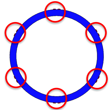
Station: 2 plane rotated 180° each other. 6 couples of ears at 60° each other
