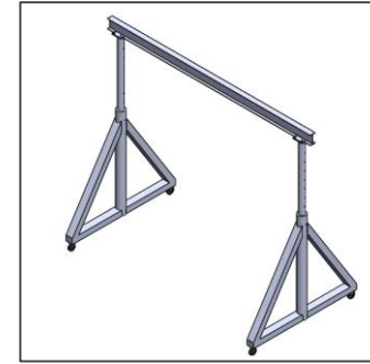
3D model of the FNAL gantry crane with adjustable height
