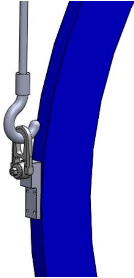
Hoist ring solution
