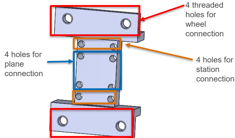
Conceptual design of the flange adapter
