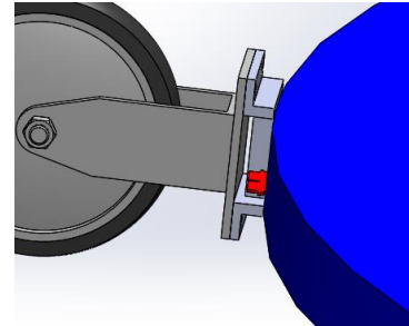
3D views of the connections: wheel – plane (on the left); wheel – station (on the right). Ears in red.
