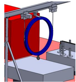
4) Lifted up
