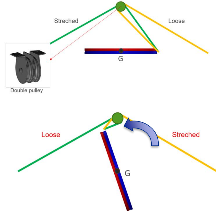
Previous idea for the mechanism of rotation. Only ropes are represented.
