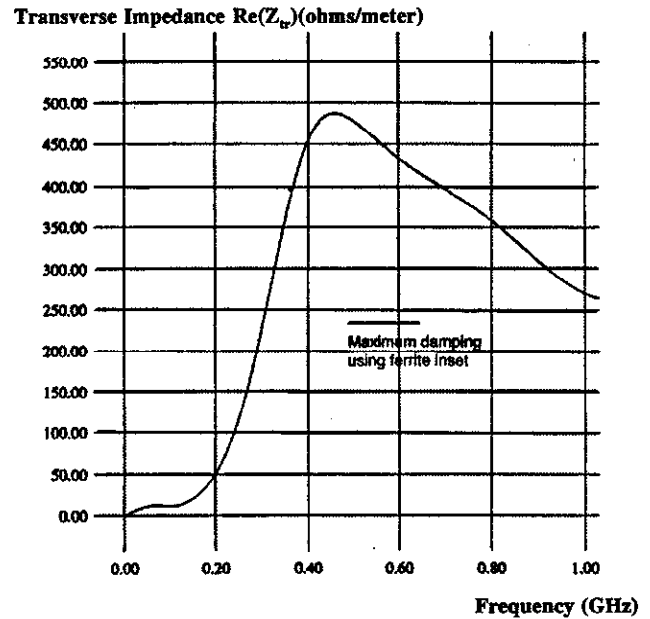
Figure 4. DARHT-2 short pulse dipole impedance spectrum with \eta = 1.1
