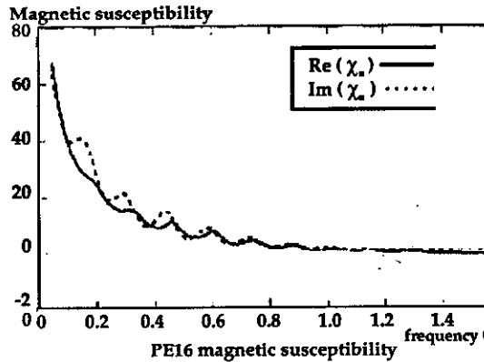
Figure 3. Magnetic dispersion for PE-16 ferrite material
