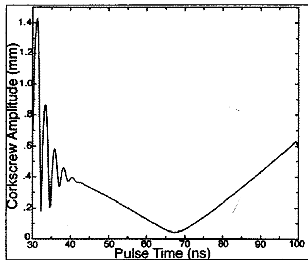
Figure 6. BBU and corkscrew motion at the end of the DARHT-2 accelerator for the short pulse option
