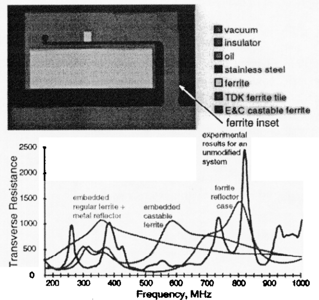
Figure 5. Computed impedance spectrum for FXR cell upgrade
