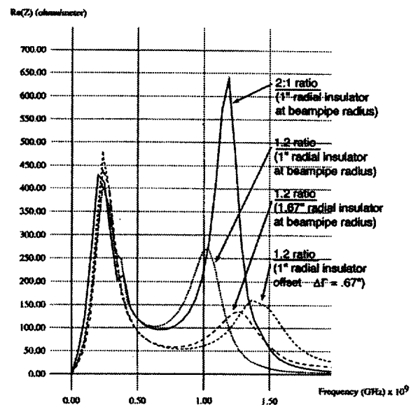
Figure 7. High gradient insulator structure in damped pillbox with ID=5.75", OD=10", and gap = 1"
