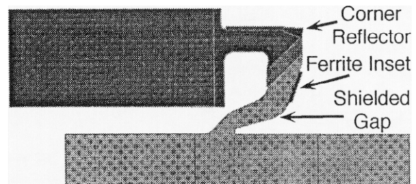
Figure 2. DARHT-2 short pulse design with ferrite inset.
