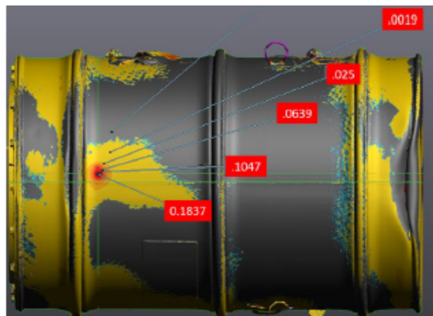
Figure 30. Post-process 3D scan.
