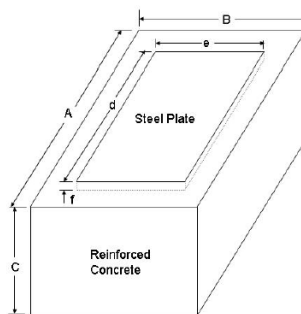
Figure 5. Drop pad general dimensions.
