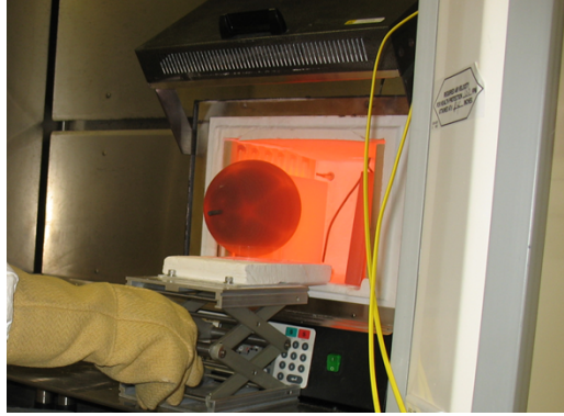
Figure 21. Special form heat test in a fume hood furnace.
