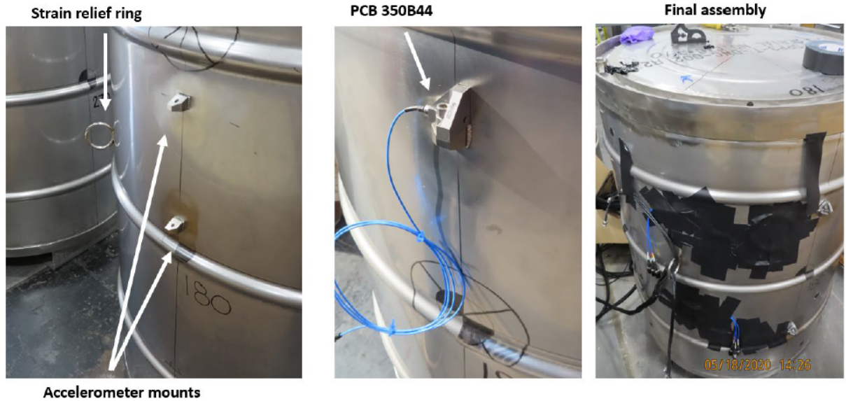
Figure 26. Package accelerometer placement.
