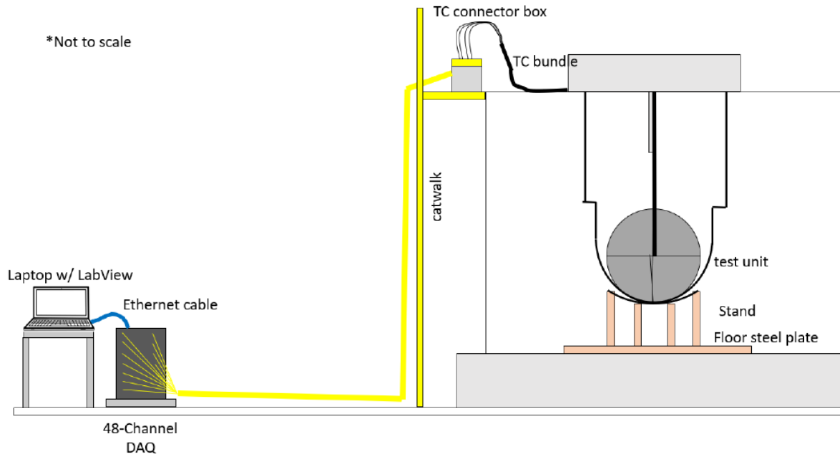
Figure 28. Typical thermal test wiring set-up.
