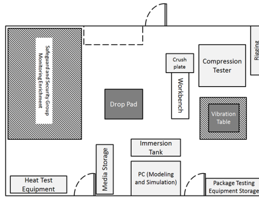
Figure 4. PEF layout.
