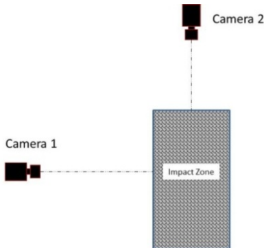
Figure 24. High-speed camera position relative to drop pad.
