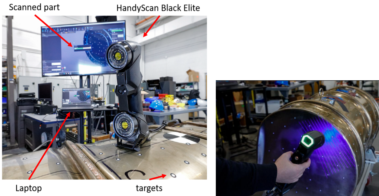
Figure 29. HandyScan Black Elite.
