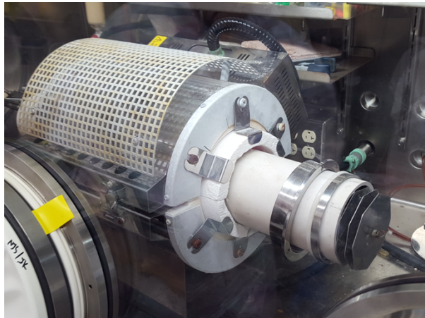
Figure 22. Special form heat test in a glove box furnace.
