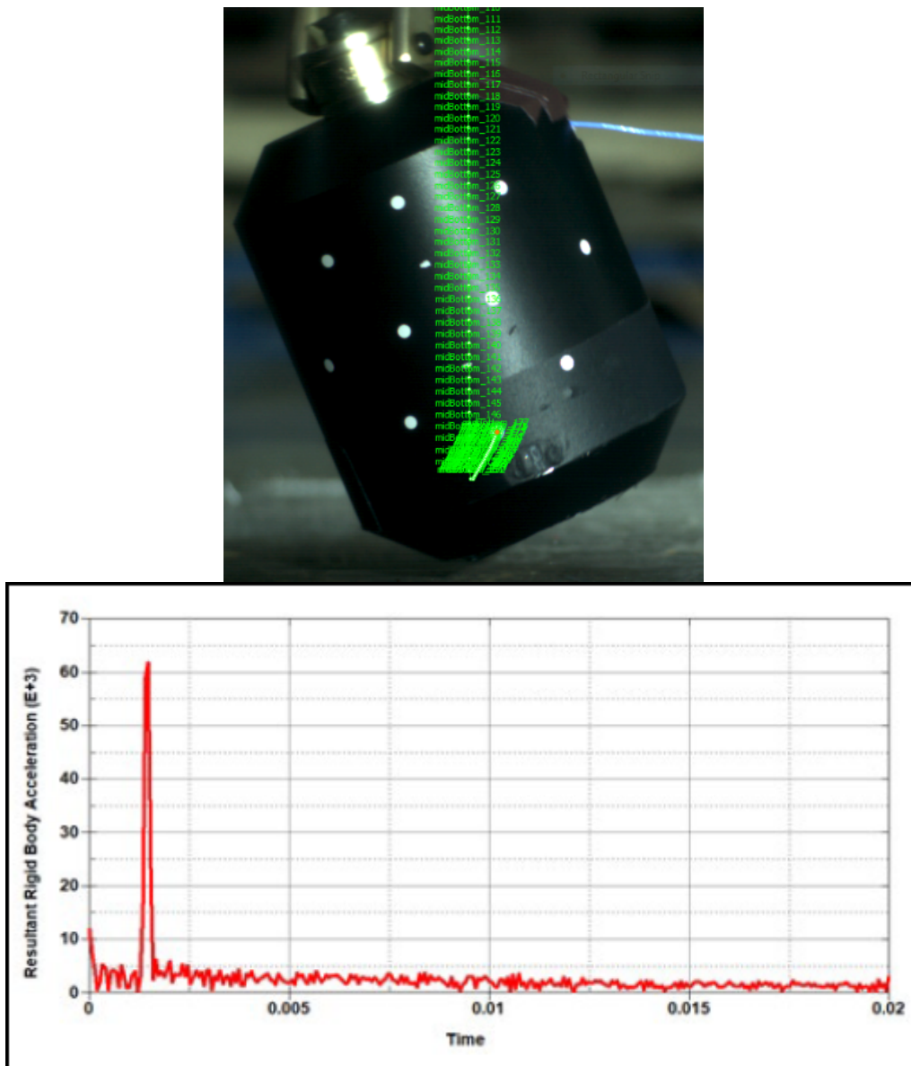
Figure 25. Digital image correlation object tracking.
