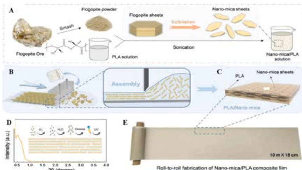
Fig. 5. PLA-Based Nanocomposites for Packaging Applications. (A) Exfoliation process of nano-mica sheets from natural phlogopite. (B) Shear force assembly process used to fabricate PLA-coated nano-mica sheets. (C) Diagram illustrating the "brick-and-mortar" configuration of nacre-inspired PLA/nano-mica films. (D) Small-angle XRD analysis of the structural organization of nano-mica sheets within the films. (E) Nacre-inspired films in rolled form, highlighting their potential for large-scale applications [130].
