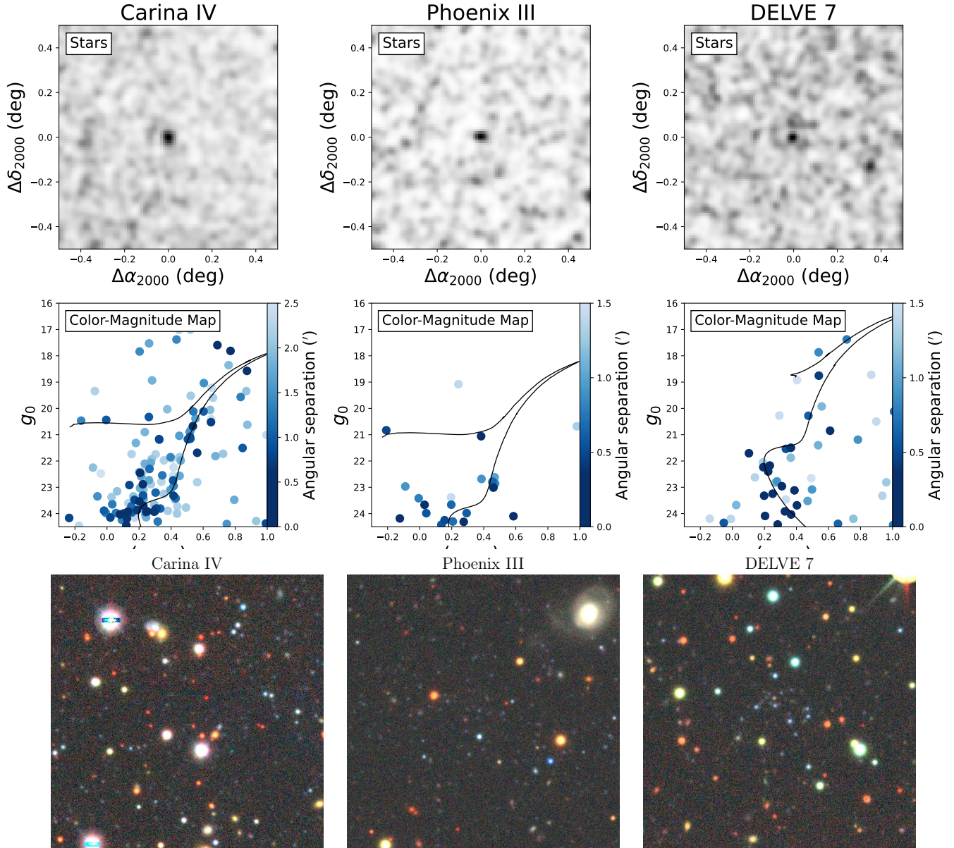
Figure 1. Diagnostic plots for each of the three newly-discovered satellites, closely matching those used to identify the systems in our search. (Top) Stellar density maps for a 1^\circ \times 1^\circ degree region centered on each candidate, smoothed with a 0.5 Gaussian kernel. (Middle) Color-magnitude diagrams for stars within 2.5' of Carina IV and 1.5' of Phoenix III and DELVE 7, centered on each candidate system. Stars are colored by separation from each system’s centroid, with darker colors representing smaller separations. Also overlaid is the best-fit old, metal-poor PARSEC isochrone, with parameters taken from the best-fit ugali results in Table 1. (Bottom) False-color coadded images ( \sim 2' \times 2' , \sim 0.03^\circ \times 0.03^\circ ) of Carina IV, Phoenix III, and DELVE 7 from the Legacy Surveys Sky Viewer DR10. Each cutout has been artificially brightened by a factor of 1.8\times to highlight faint sources.
