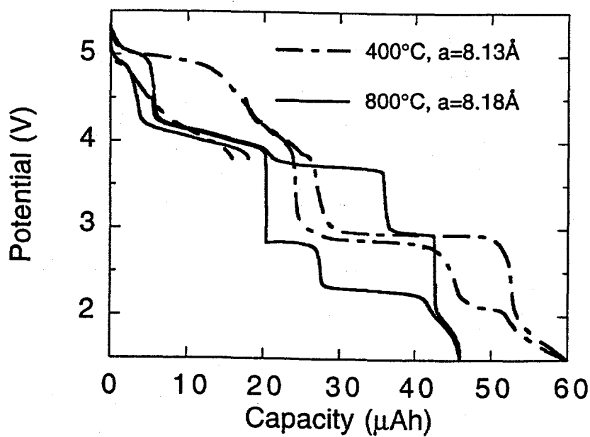
Fig. 3. Low current discharge-charge curves for Li/LiMn 2 O 4 cells with cathodes annealed at 400 and 800°C.
