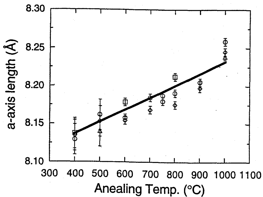
Fig. 2. Change in the a-axis length of LiMn 2 O 4 thin film with annealing temperature.
