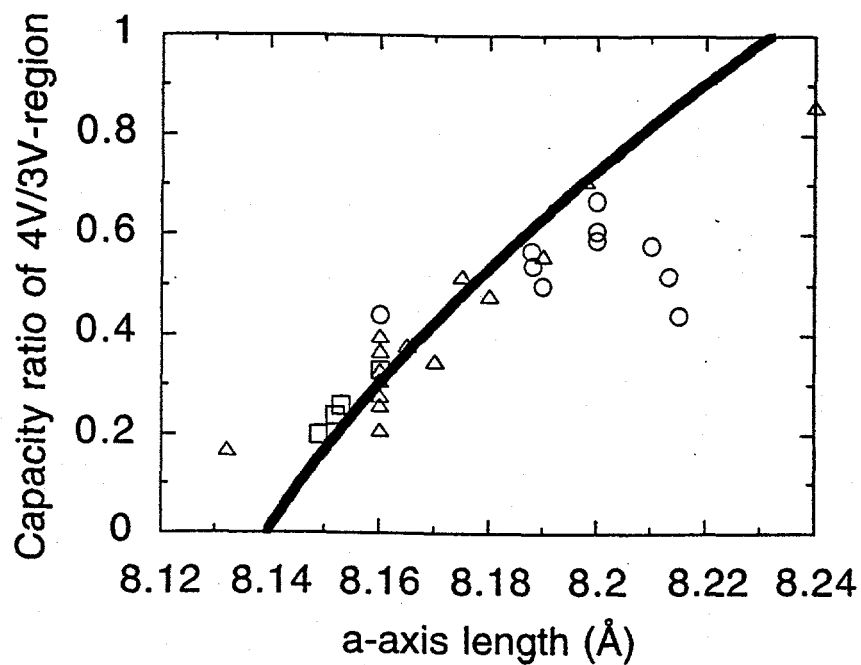
Fig. 4. Measured capacity ratios vs. a-axis length. The solid curve was calculated from a fit of the bulk data for a vs. x in the model \text{Li}[\text{Li}_x\text{Mn}_{2-x}]\text{O}_4 .
