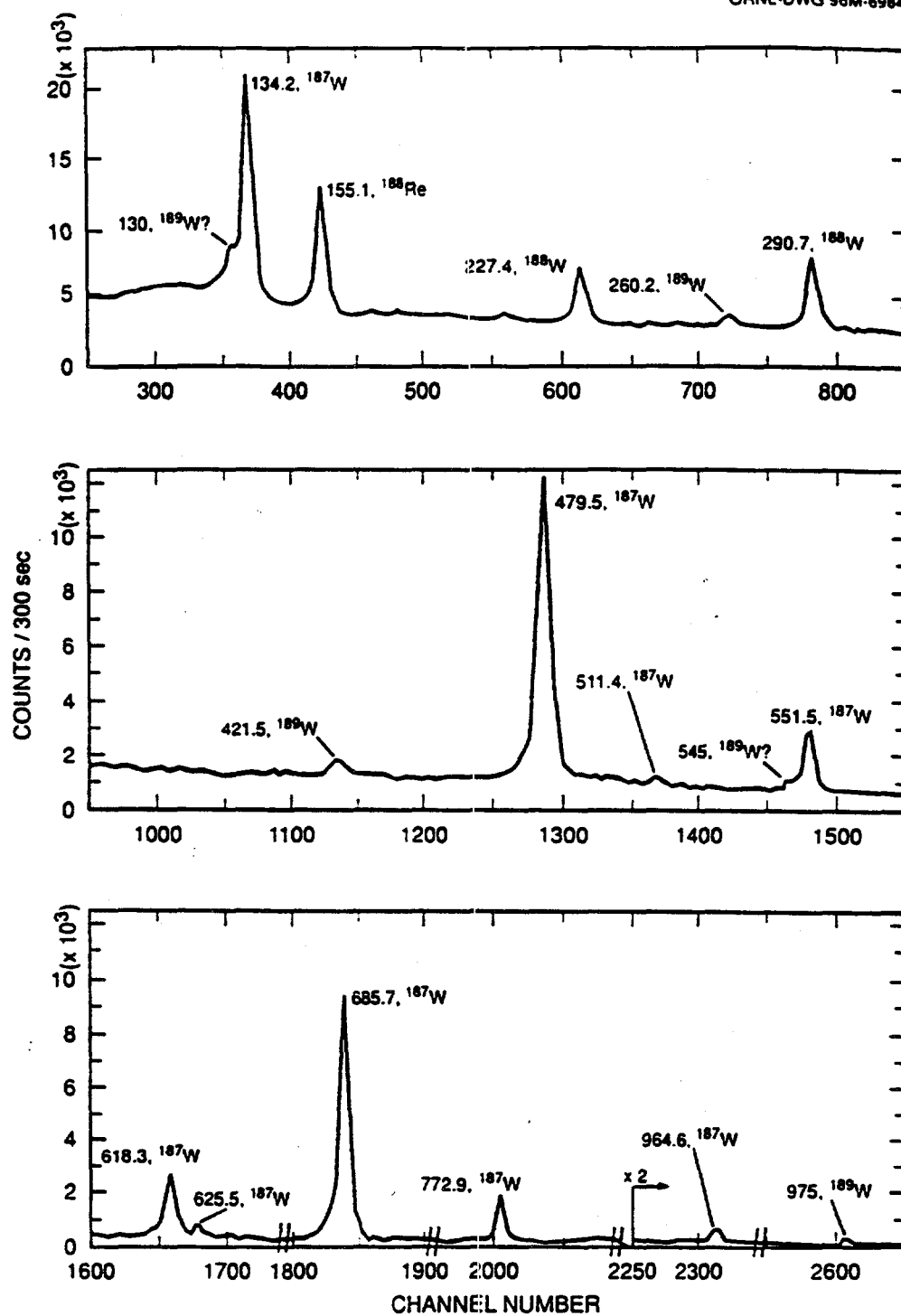
Figure 2. Gamma-ray spectrum of ^{189}\text{W} produced by neutron irradiation of ^{188}\text{W} target.
