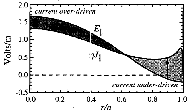
Fig. 2. An illustration showing that \langle E \rangle_\parallel \neq \eta \langle J \rangle_\parallel for an equilibrium modeled using typical MST parameters.
