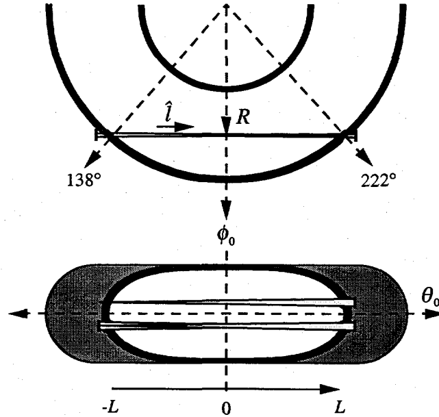
Fig. 6. The toroidal viewing chords, with both the opposing views and the views symmetrically placed above and below the mid-plane shown.
