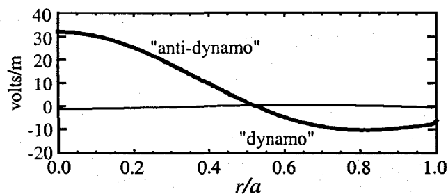
Fig. 14. From Ohm's law modeling, the electric field \eta J_{\parallel} - E_{\parallel} that must be supplied by the RFP dynamo during (heavy line) and away (light line) from the sawtooth crash. "Anti-dynamo" refers to suppression of J_{\parallel} in the core, and "dynamo" refers to driving of J_{\parallel} in the edge.
