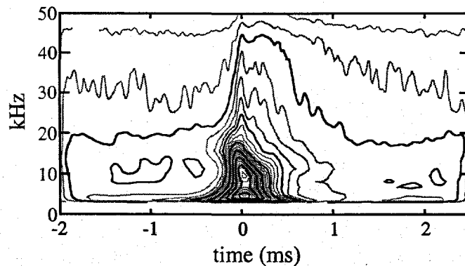
Fig. 11. Wavelet spectra of the toroidal velocity fluctuation power density over a sawtooth cycle.
