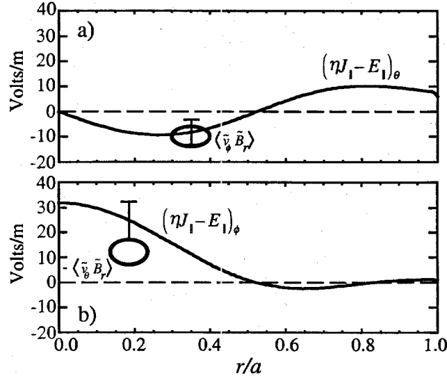
Fig. 15. The a) poloidal and b) toroidal components of \eta J_1 - E_1 estimated from modeling, compared to two experimental measurements of the MHD dynamo at the sawtooth crash. The uncertainties in \eta J_1 - E_1 are represented by error bars; the uncertainties in spatial localization and amplitude of the dynamo measurements are represented by the heavy oval datapoints.
