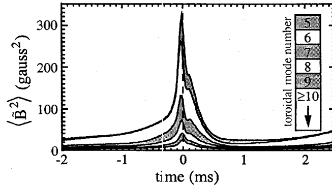
Fig. 8. \tilde{B}_{\theta,n}^2(t) ensemble over a sawtooth window. The total magnetic fluctuation power is traced out by the top curve. The light and dark bands indicate the distribution of power among the dominant toroidal modes as indicated by the key.
