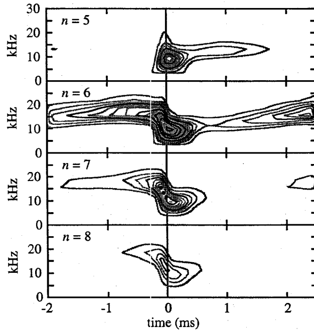
Fig. 9. Wavelet spectra of the magnetic fluctuation power density of dominant m = 1 modes over a sawtooth cycle.
