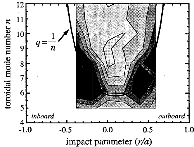
Fig. 13. Amplitude contours of mode-resolved \left(\sqrt{\tilde{v}_\theta^2}\right)_n , estimated by dividing the mode-resolved dynamo product \langle \tilde{v}_\theta \tilde{B}_r \rangle_n by \tilde{B} for that mode, measured at various poloidal viewing chord impact parameters. The velocity fluctuation amplitude for a particular n -mode peaks approximately at the impact parameter where that mode is expected to be resonant (estimated from the q -profile), indicating that the velocity fluctuation eigenfunction for a particular n -mode peaks near the 1/n resonant surface in the plasma.
