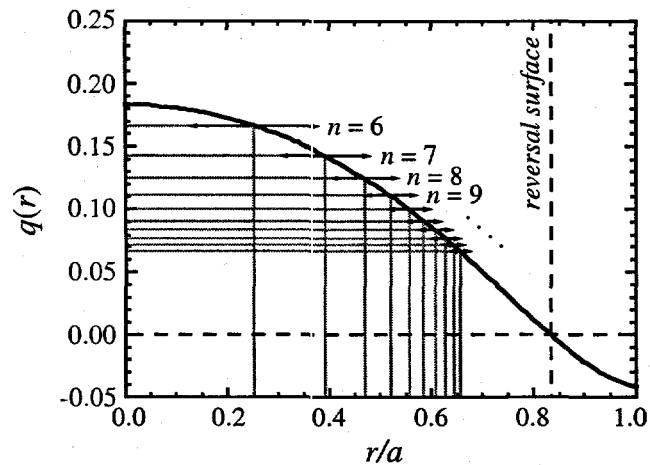
Fig. 3. A cylindrical model of the safety factor profile before a sawtooth crash for a typical, low current MST discharge. The horizontal arrows represent estimated island widths.
