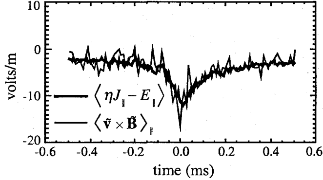
Fig. 16. Comparison of the ensemble averaged MHD dynamo product measured with the optical probe at r/a = 0.9 to parallel Ohm's law during the sawtooth crash.
