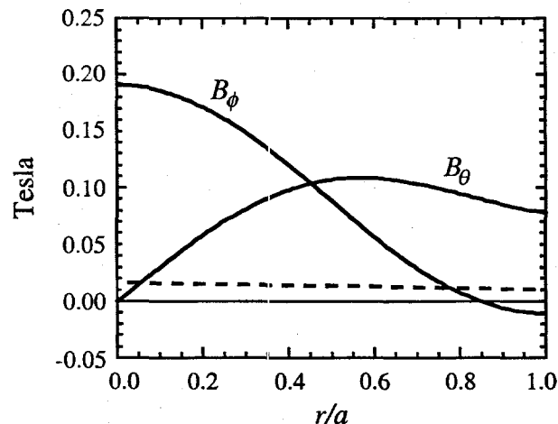
Fig. 1. The solid lines illustrate the magnetic field configuration of an RFP plasma in MST. The dashed line is the toroidal field pre-fill prior to formation of the RFP plasma.
