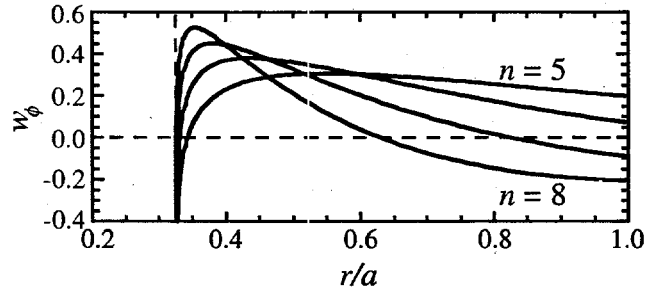
Fig. 7. The toroidal viewing chords geometric sensitivity functions w_\phi for m = 1, n = 5-8 .
