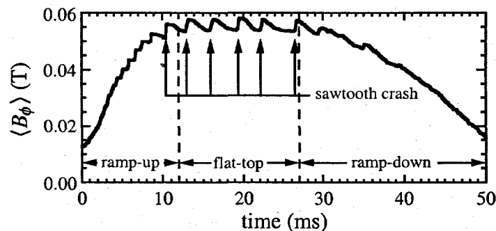
Fig. 4. The volume averaged toroidal field of a standard low current MST discharge. Note the well-defined sawteeth generating toroidal flux during the “flat-top” period.
