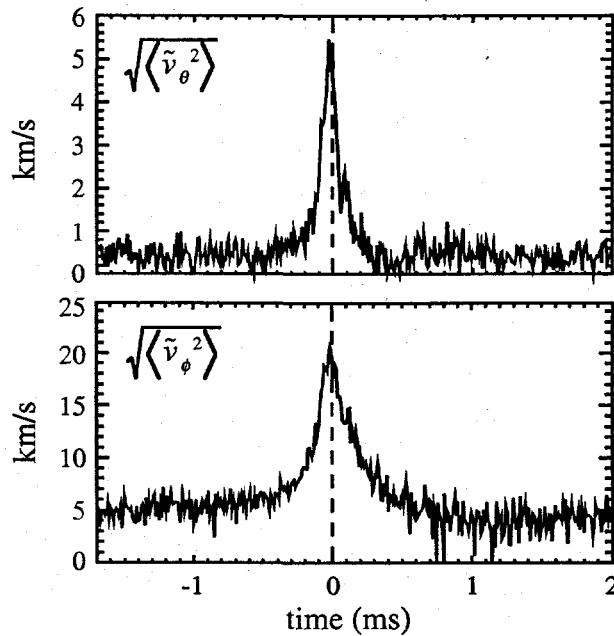
Fig. 10. The rms amplitudes of the poloidal and toroidal velocity fluctuations over a sawtooth cycle.
