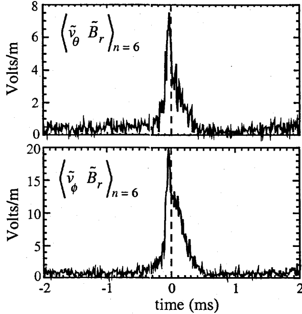
Fig. 12. Two n = 6 components of the dynamo, both of which suppress parallel current in the core of MST. Note the dramatic peaking of the MHD dynamo at the sawtooth crash.
