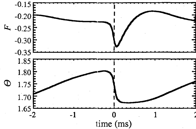
Fig. 5. Two key equilibrium quantities ensemble averaged over a sawtooth cycle: a) the reversal parameter F and b) the pinch parameter \Theta .
