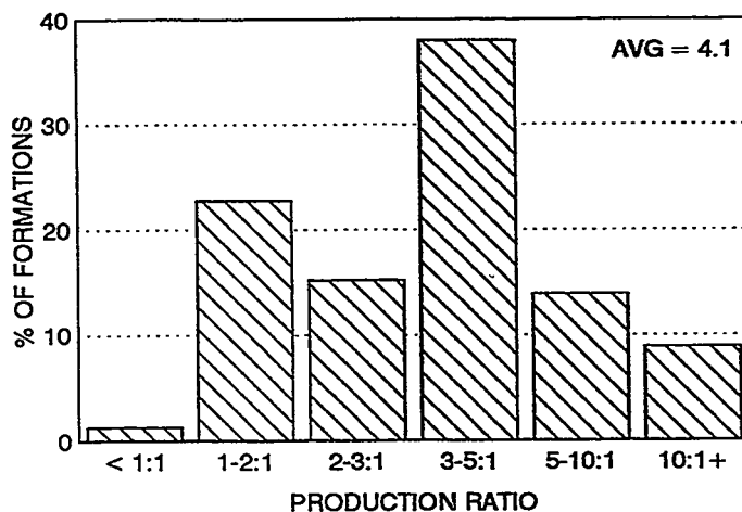
Figure D-13. Production Ratio: All Canadian Pools
