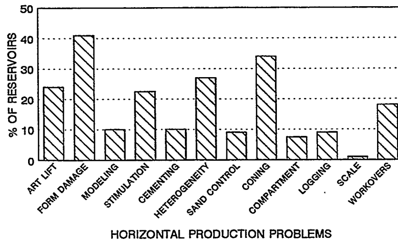
Figure D-27. Horizontal Well Production Problems: All Canadian Pools
