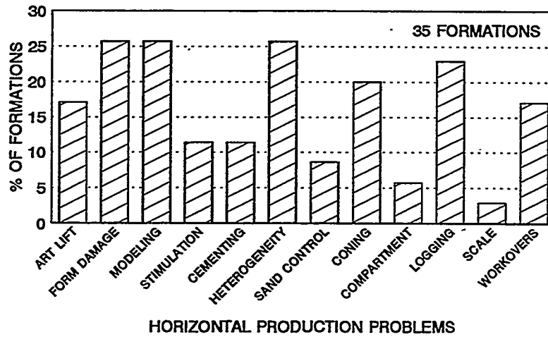
Figure C-27. Horizontal Production Problems: U.S.A. Clastics
