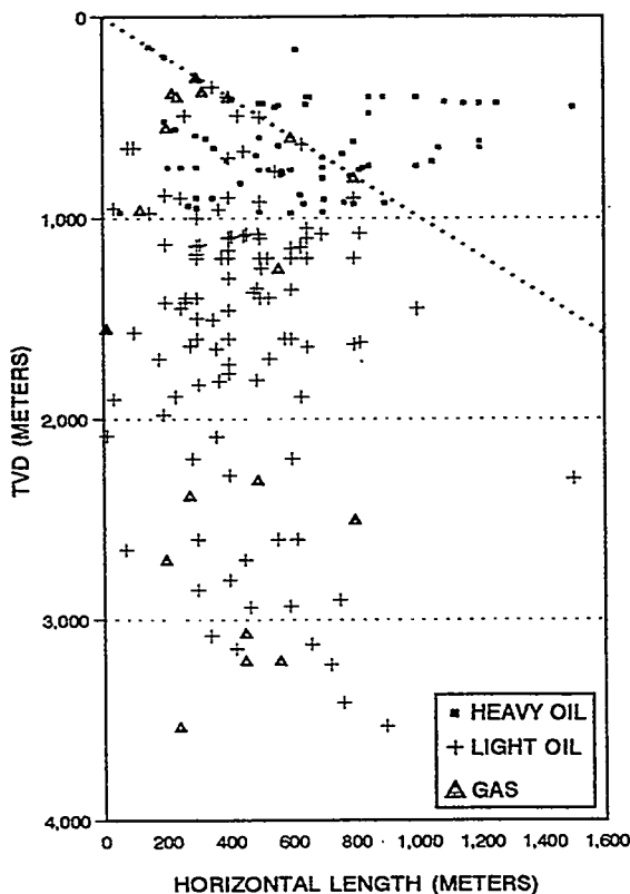
Figure 3-13. TVD and Horizontal Length
