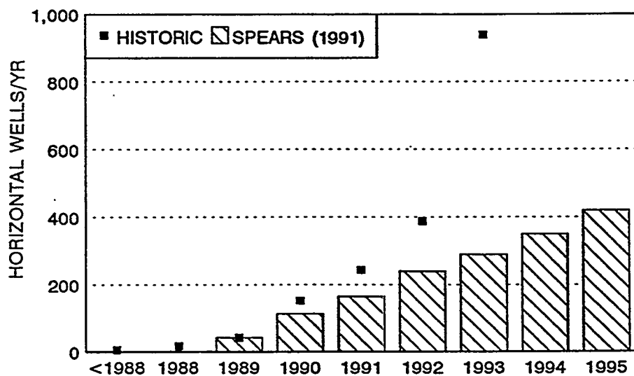
Figure 5-9. Early Canadian Horizontal Forecast (Spears and Associates, 1991)
