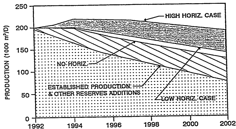
Figure D-2. Production From Canadian Horizontal Wells (NEB, 1993)
