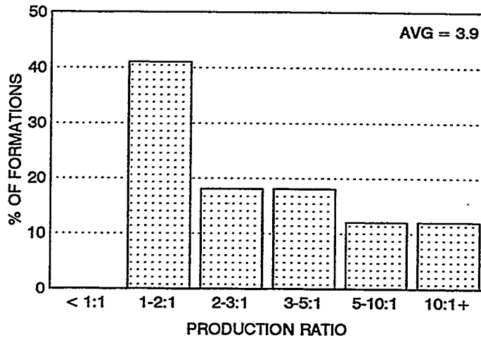
Figure C-20. Production Ratio: U.S.A. Carbonates
