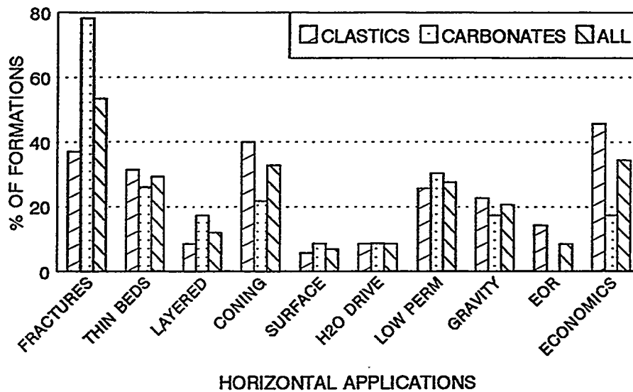
Figure ii. U.S.A. Horizontal Technology Applications
