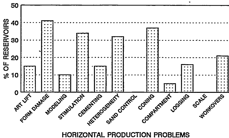
Figure D-29. Horizontal Well Production Problems: Canadian Carbonates
