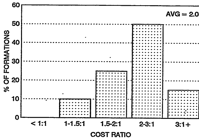
Figure D-19. Cost Ratio: Canadian Carbonates
