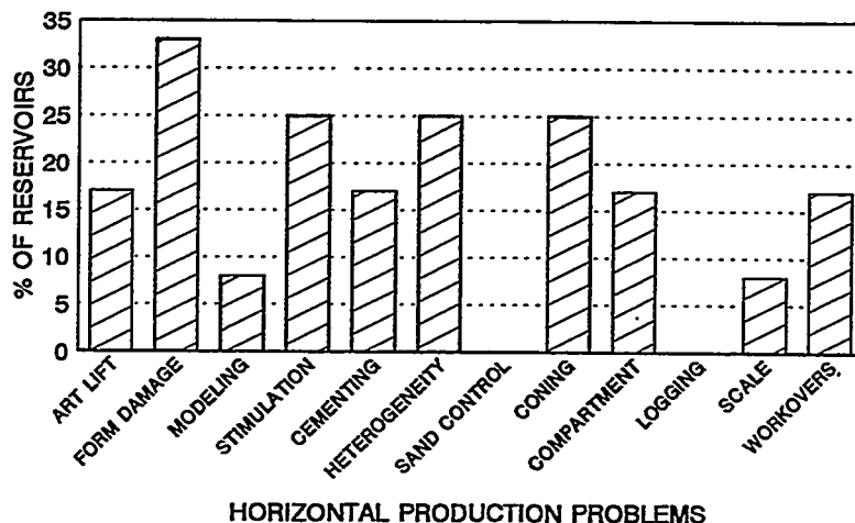
Figure D-28. Horizontal Well Production Problems: Canadian Light-Oil Clastics
