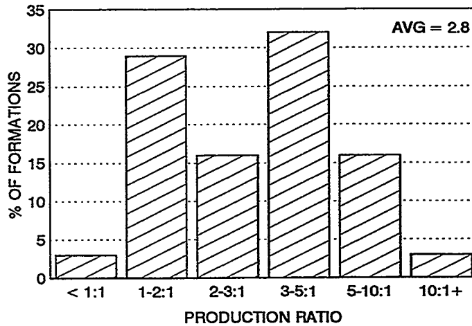
Figure C-18. Production Ratio: U.S.A. Clastics
