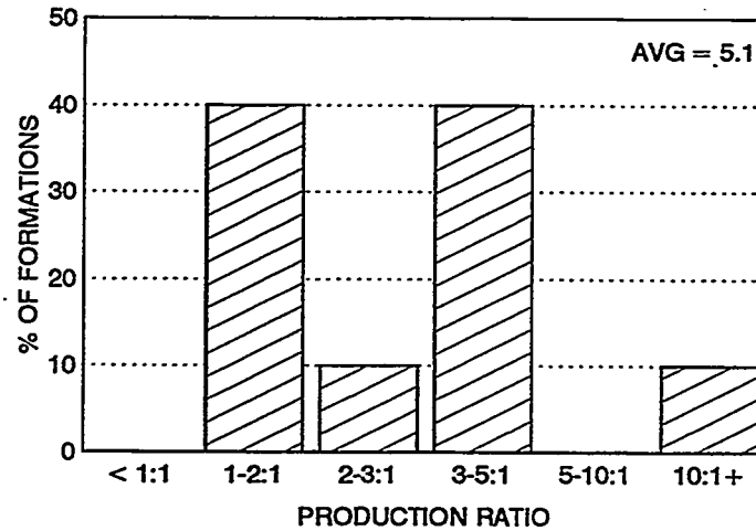
Figure D-14. Production Ratio: Canadian Light-Oil Clastics
