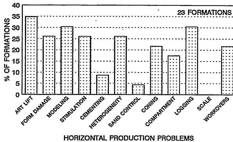
Figure C-28. Horizontal Production Problems: U.S.A. Carbonates
