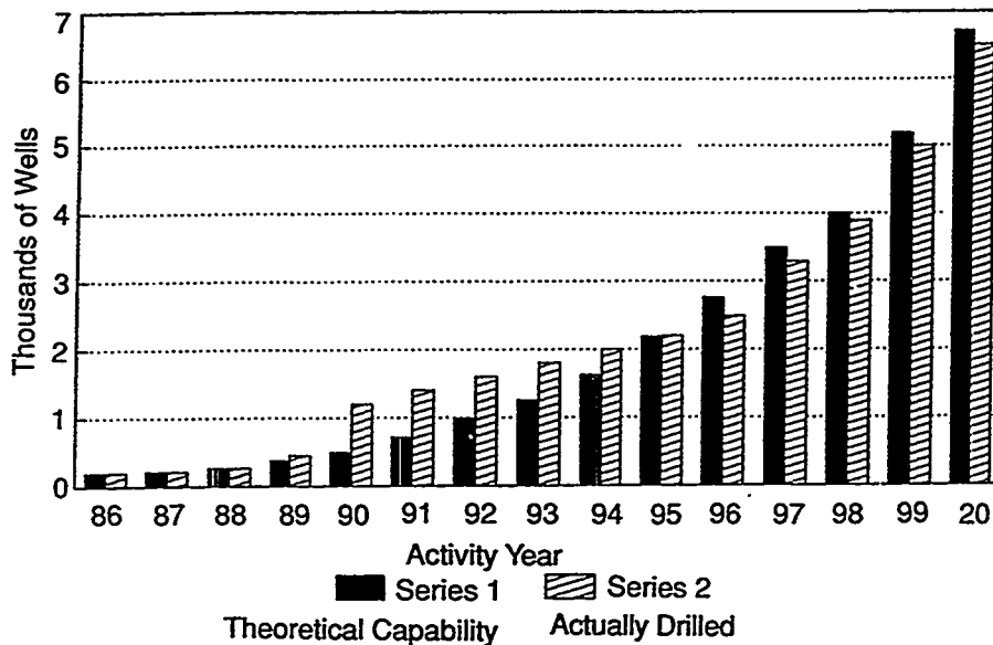
Figure 5-1. Early Worldwide Horizontal Drilling Forecast (Jelsma, 1991)
