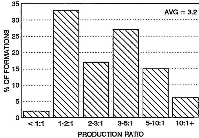
Figure C-16. Production Ratio: All U.S.A. Formations
