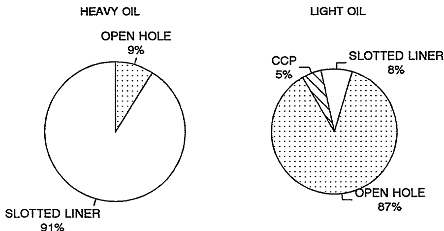
Figure 3-19. Horizontal Completion Types for 1993
