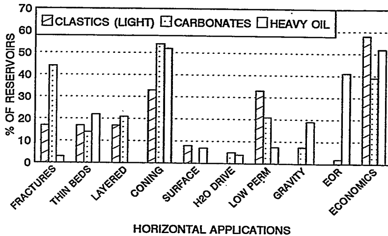
Figure D-7. Horizontal Applications: Canadian Resource Type
