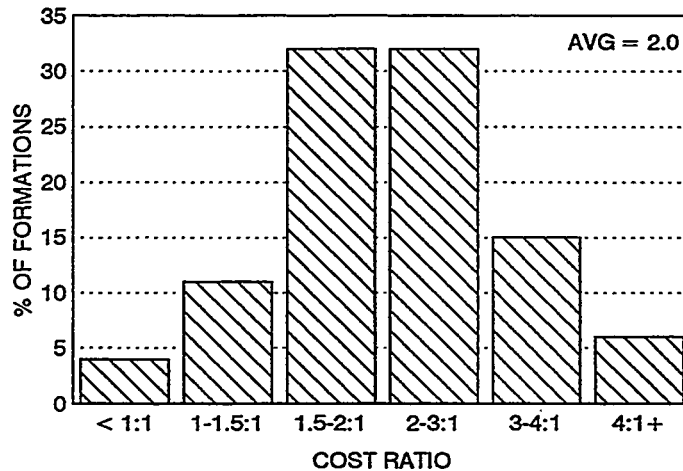
Figure C-17. Cost Ratio: All U.S.A. Formations
