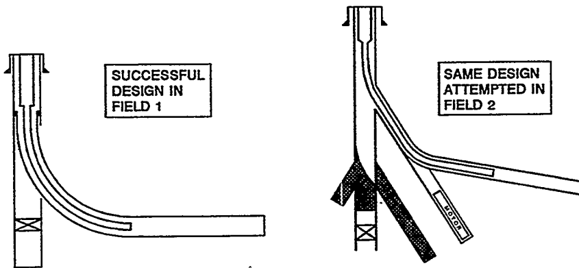
Figure 3-12. Ineffective Use of Standard Well Design
