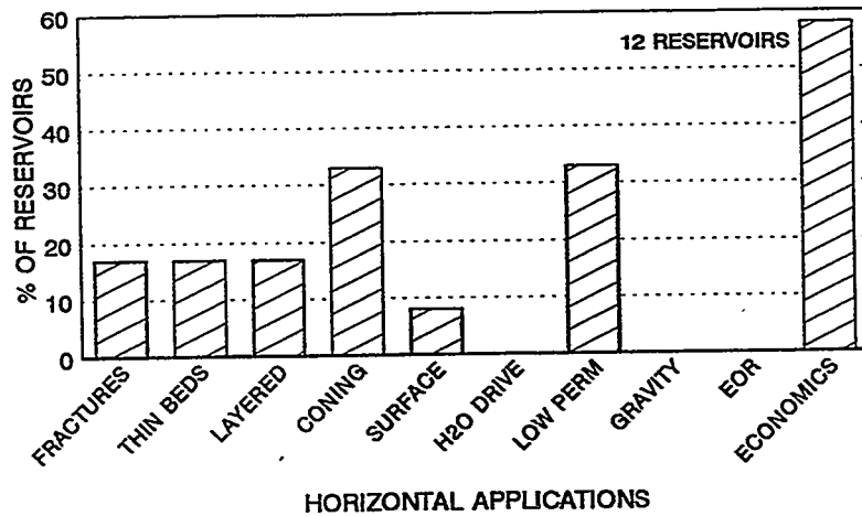
Figure D-4. Horizontal Applications: Canadian Light-Oil Clastics
