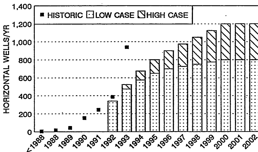
Figure 5-10. NEB Canadian Horizontal Well Forecast (NEB, 1993)
