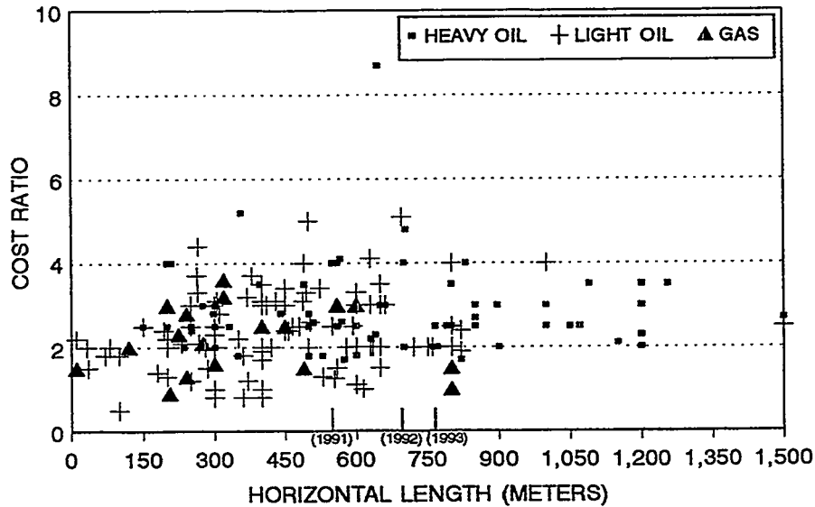
Figure 3-15. Horizontal Length and Cost Ratio
