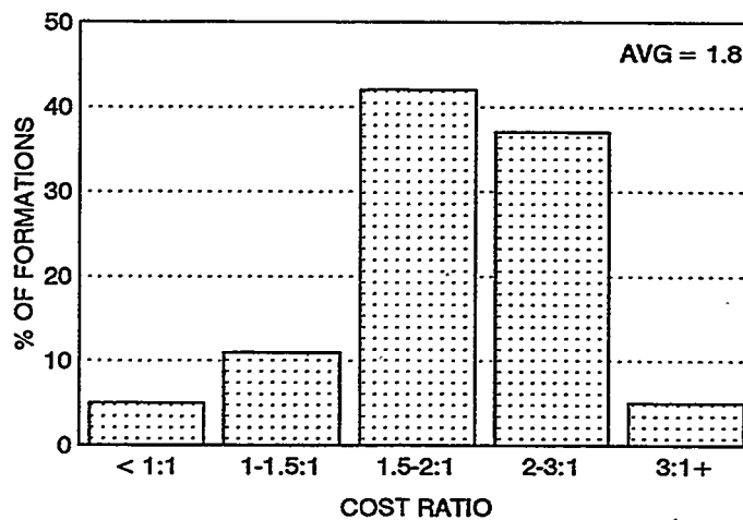
Figure C-21. Cost Ratio: U.S.A. Carbonates
