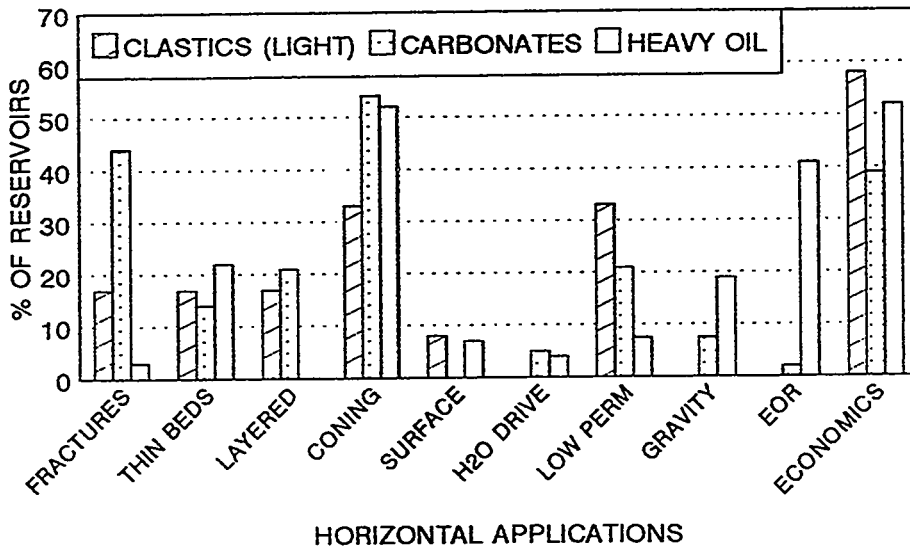
Figure 3-8. Canadian Horizontal Technology Applications
