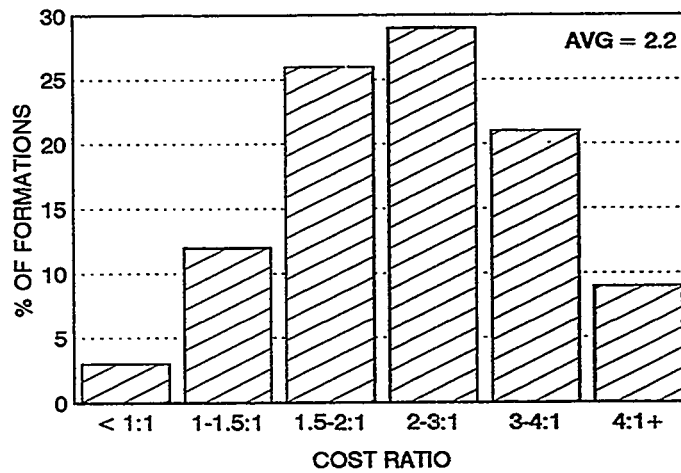
Figure C-19. Cost Ratio: U.S.A. Clastics
