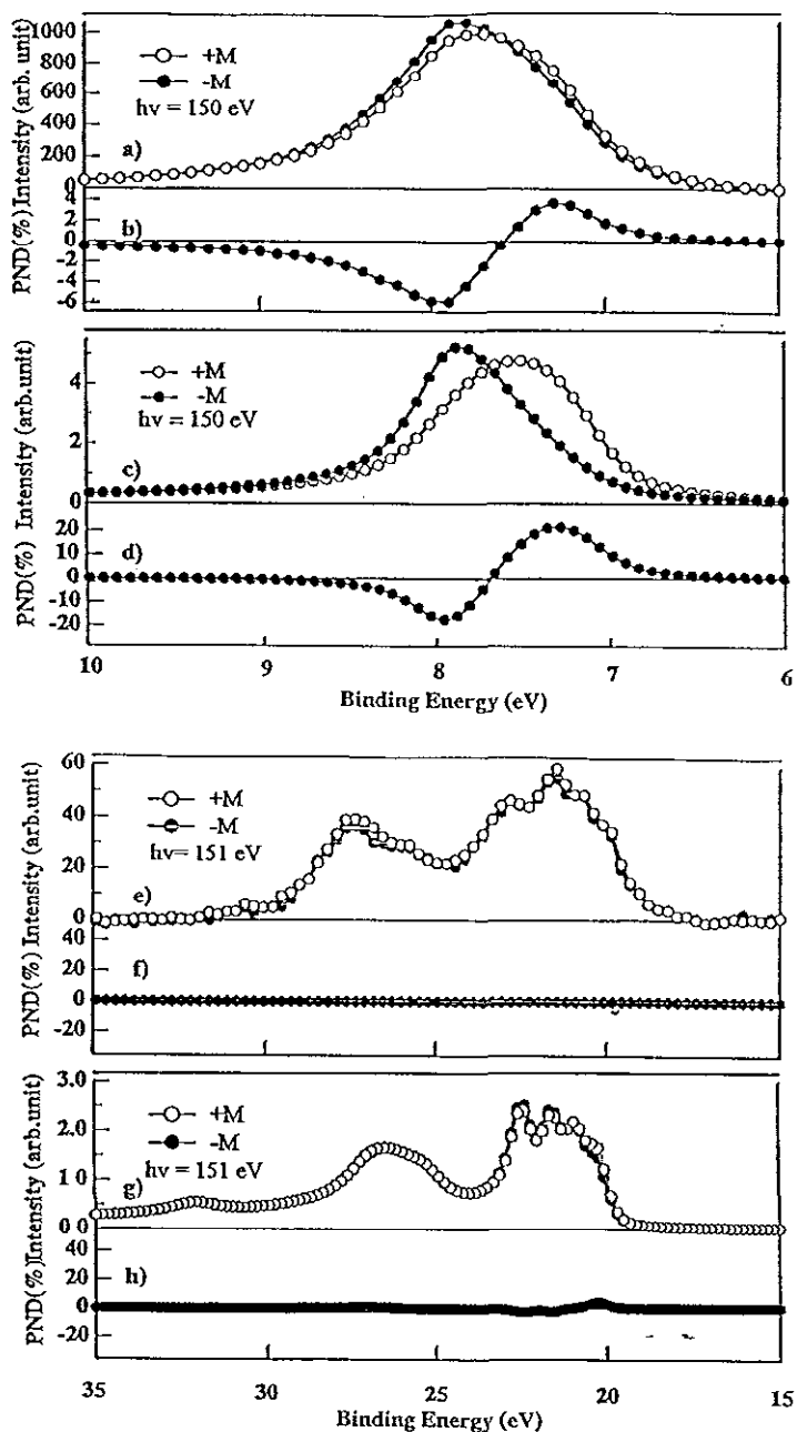
Figure 1. A series of experimental and theoretical 4f and 5p photoemission spectra (for the two opposite magnetization directions) and normalized difference curves. The photon energy was 150 eV for the 4f and 151 eV for the 5p (a) Gd 4f, photoelectron spectra, experimental. (b) Gd 4f, photoelectron spectra difference, experimental (c) Gd 4f, photoelectron spectra, theory. (d) Gd 4f, photoelectron spectra difference, theory. (e) Gd 5p, photoelectron spectra, experimental (f) Gd 5p, photoelectron spectra difference, experimental. (g) Gd 5p, photoelectron spectra, theory. (h) Gd 5p, photoelectron spectra difference, theory. EDC is energy distribution curve. The spectra in (a), (c), (e), & (g) are EDC's, where the photon energy is held constant and the kinetic energy is scanned. PND stands for peak normalized difference, where the dichroism difference at each binding energy is divided by the sum of the two intensity maxima, one from each pair. The photon energies of 150 eV and 151 eV are “on” resonance. The relative intensities of the experimental curves were determined by normalizing to the valence band intensities and then correcting for the valence band cross sections.
