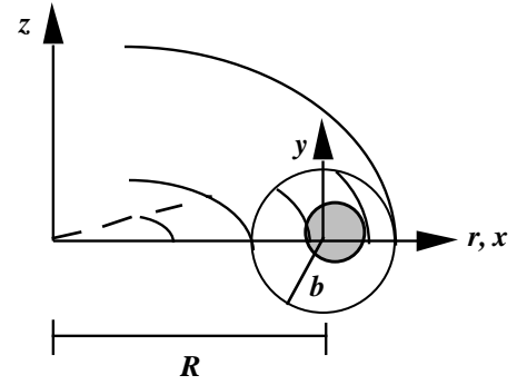
Fig. 1 A displaced round beam in a continuous bend
