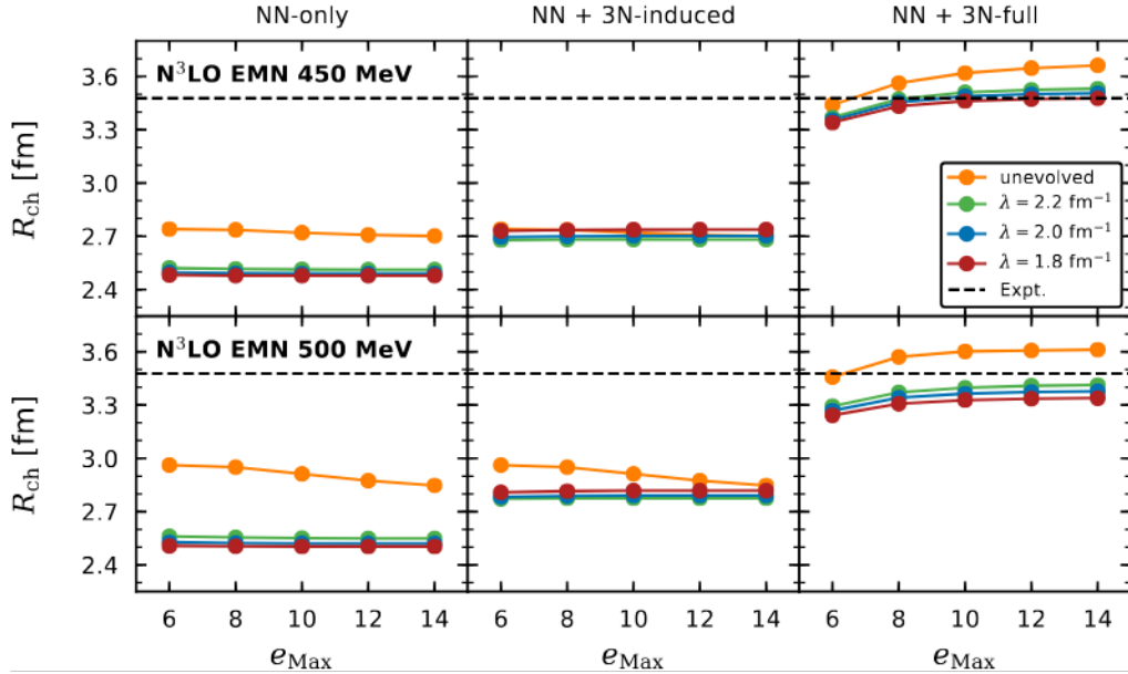
FIG. 5. Same as Fig. 4 but for the charge radius of {}^4\text{Ca} . The experimental value is taken from Ref. [33]. Note that the results for unevolved interactions are barely visible in some panels, as they are on top of the corresponding evolved results.
