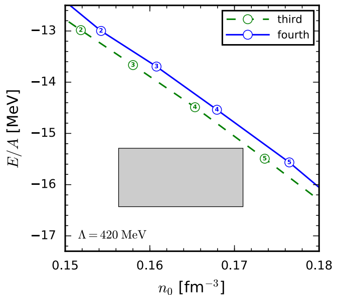
FIG. 1. Saturation point of symmetric nuclear matter at third (green-dashed line) and fourth (blue-solid line) order in MBPT as trajectory of c (see annotated values inside the circles), while c_E is determined by the {}^3\text{H} binding energy. The results are based on the N^3\text{LO} EMN 420 MeV NN potential with consistent 3N forces at N^3\text{LO} . For details on the fits to the empirical saturation region (gray box) see Ref. [6].
