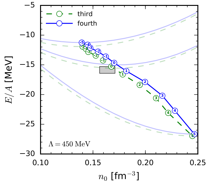
FIG. 9. Same as Fig. 1 but for the N 3 LO EMN 450 MeV interaction. Note the increased range in density and in c couplings (annotated). We also show the energy per particle for three interactions with c = 5, 0.25, 5 at third and fourth order in MBPT. For c = 5 , the saturation point is more exploratory, as this is not as constrained in density from our calculations up to densities of 0.25 \text{ fm}^{-3} .
