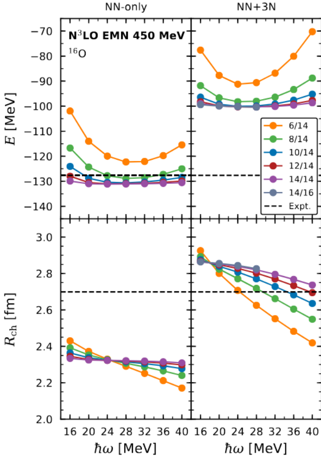
FIG. 2. Ground-state energy (top) and charge radius (bottom panel) of ^{16}\text{O} as a function of the harmonic-oscillator frequency \omega at \text{N}^3\text{LO} for the NN-only EMN 450 MeV potential and the consistent NN+3N interaction in the left and right panels, respectively. Results are shown for different sizes of the single-particle basis, e_{\text{Max}} = 6, 8, 10, 12, and 14 , and for E_{3\text{Max}} = 14 and 16 , denoted by e_{\text{Max}}/E_{3\text{Max}} . The experimental values (black-dashed lines) are taken from Refs. [32, 33].
