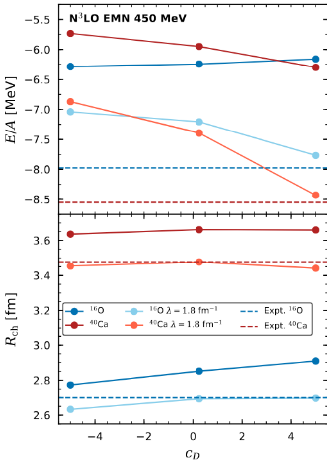
FIG. 8. Ground-state energies (top) and charge radii (bottom panel) for ^{16}\text{O} and ^{40}\text{Ca} as a function of c (with corresponding c_E value from the triton binding energy, see Table I). Results are shown for unevolved and SRG-evolved potentials with \lambda = 1.8 \text{ fm}^{-1} . The experimental values from Refs. [32, 33] are given by the dashed lines.
