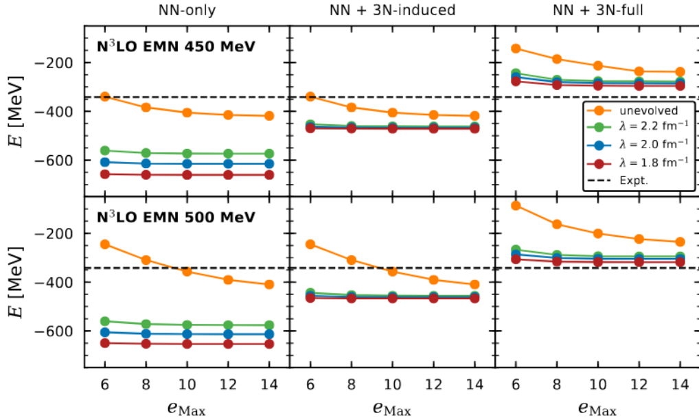
FIG. 4. Ground-state energy of {}^4\text{Ca} as a function of e_{\text{Max}} for the NN-only (left), NN+3N-induced (middle), and NN+3N-full (right) interactions of the \text{N}^3\text{LO} EMN 450 MeV and 500 MeV potentials, unevolved and SRG-evolved to resolution scales \lambda = 2.2, 2.0, and 1.8 \text{ fm}^{-1} , respectively. Results are shown for \omega = 20 \text{ MeV} and E_{3\text{Max}} = 14 . The experimental value from Ref. [32] is given by the black-dashed line.
