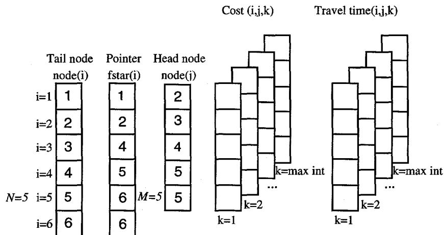
Figure 3.4: Network Representation for the General TDLCP Problem
