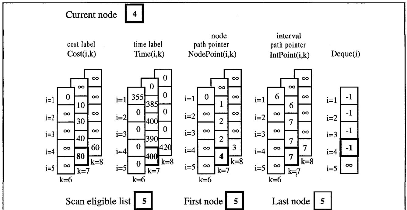
Figure 3.11: - Iteration 4 of the TDLCP Example Problem
