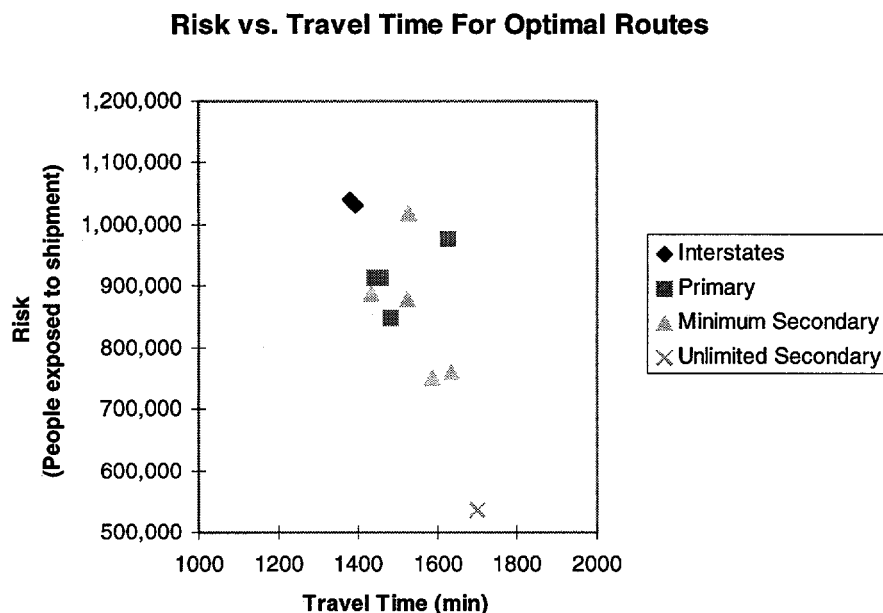
Figure 5.9: Risk vs. Travel Time for Optimal Least-Risk Routes for Each Road Type
