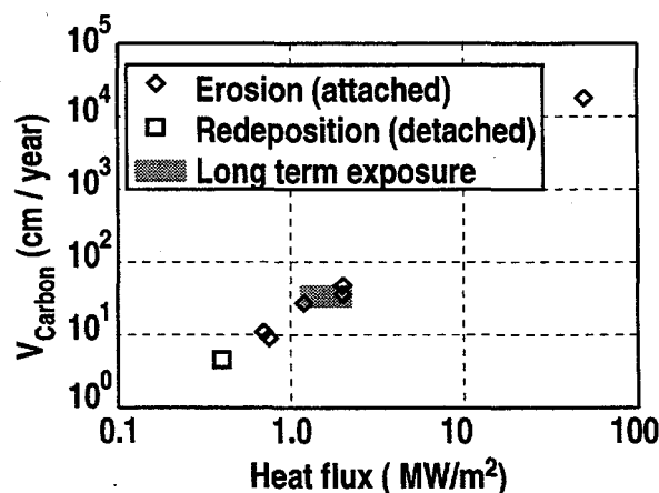
Fig. 5. Summary of peak net carbon erosion rates ( \text{cm/exposure-year} ) vs. peak incident heat flux for attached OSP plasmas (logarithmic plot). The erosion rates from a long-term (9 month, 1400 shots) exposure of lower divertor tiles [1] have been included. JET OSP erosion results from [2].
