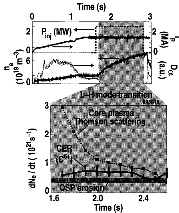
Fig. 4. (Top) Time traces of plasma density and D_\alpha showing ELM-free period used for DiMES erosion measurements (shaded area). (Bottom) Measured rate of change in core electron inventory during ELM-free phase and inferred source rate from core carbon inventory increase and OSP erosion rate. Each carbon atom contributes six electrons.
