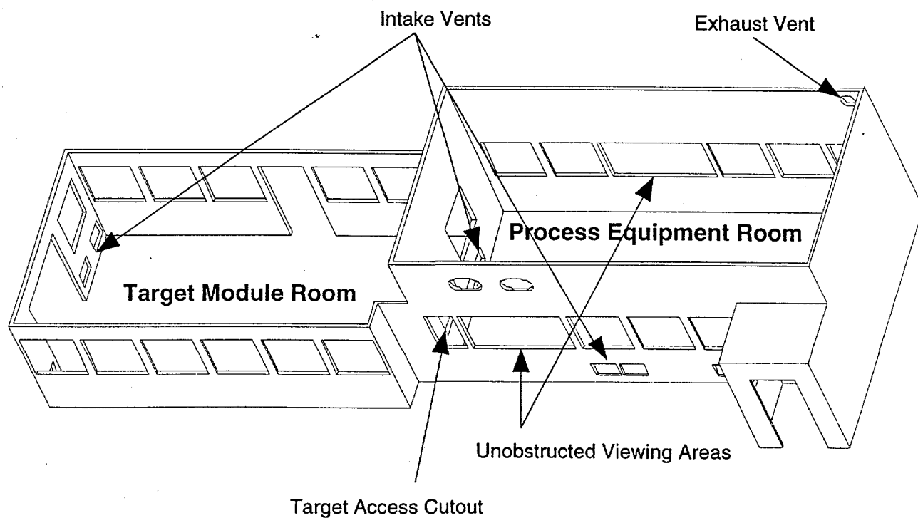
Figure 2. The TTF enclosure arrangement.
