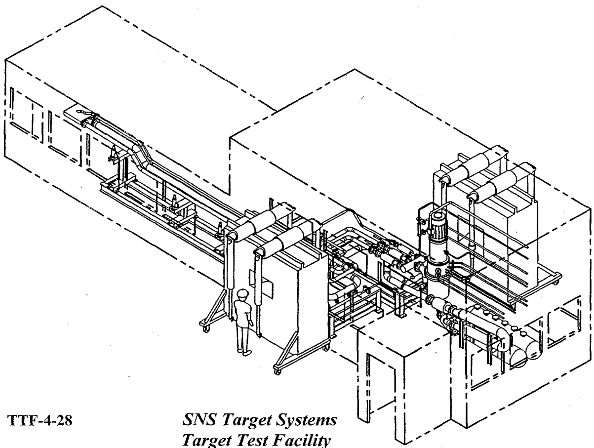
Figure 3. TTF enclosure and mechanical master-slave manipulators.
