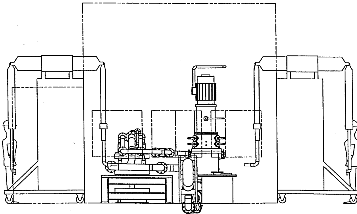
Figure 4. CRL model F manipulators on the TTF east and west sides.
