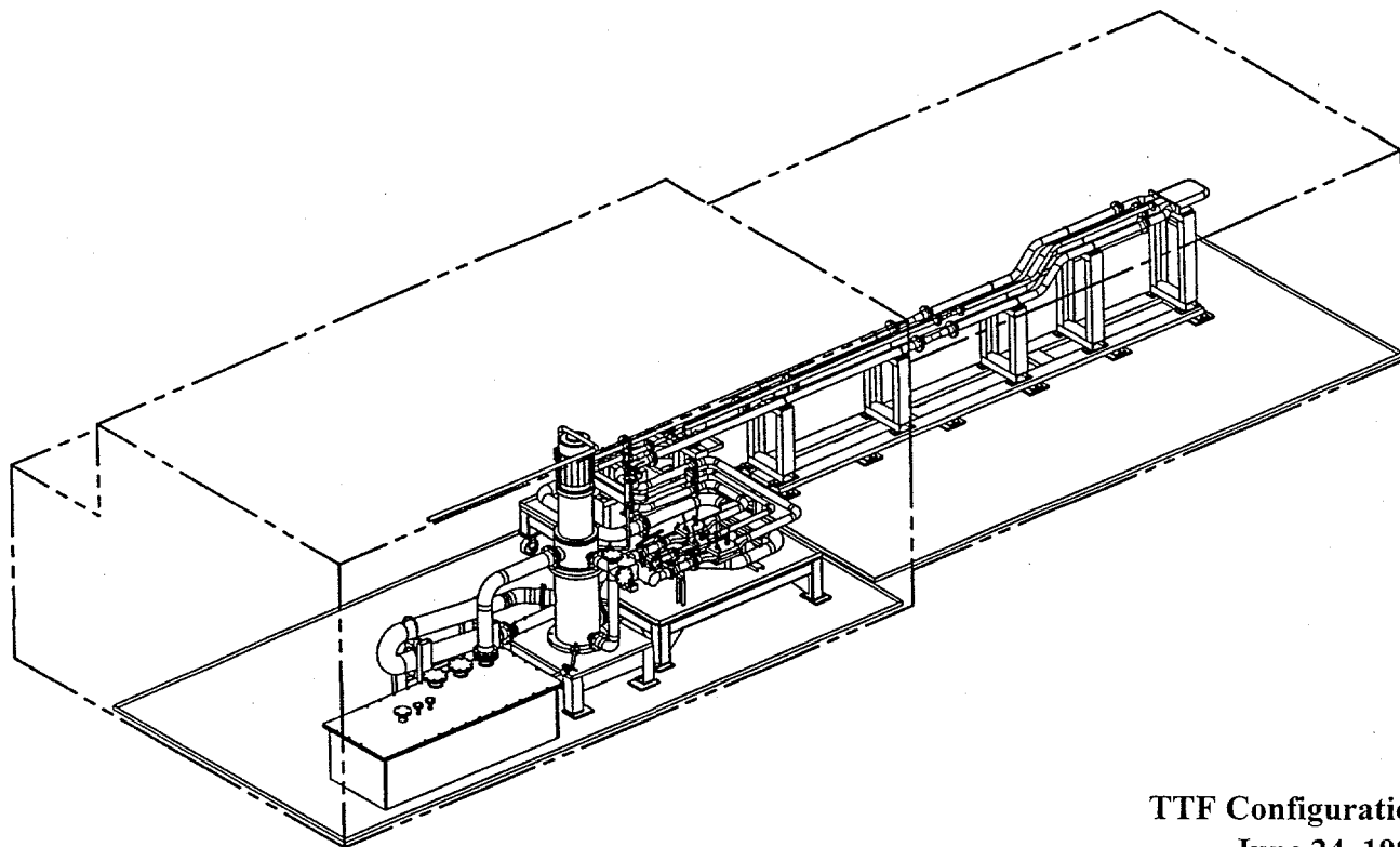
Figure 1. Mercury target flow loop equipment.
