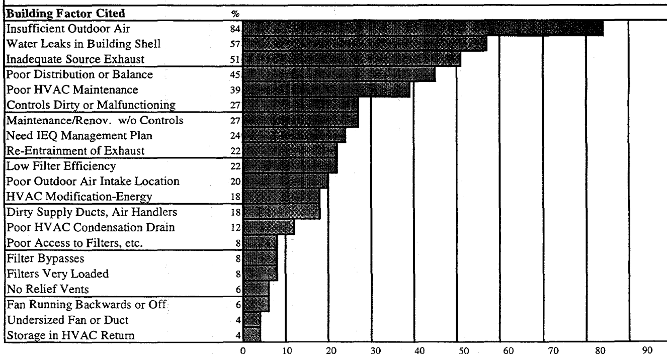
Figure 8.1 Building Factors Associated with IAQ Problems, 49 NIOSH School Health Hazard Evaluation Reports, 1981 - 1994
