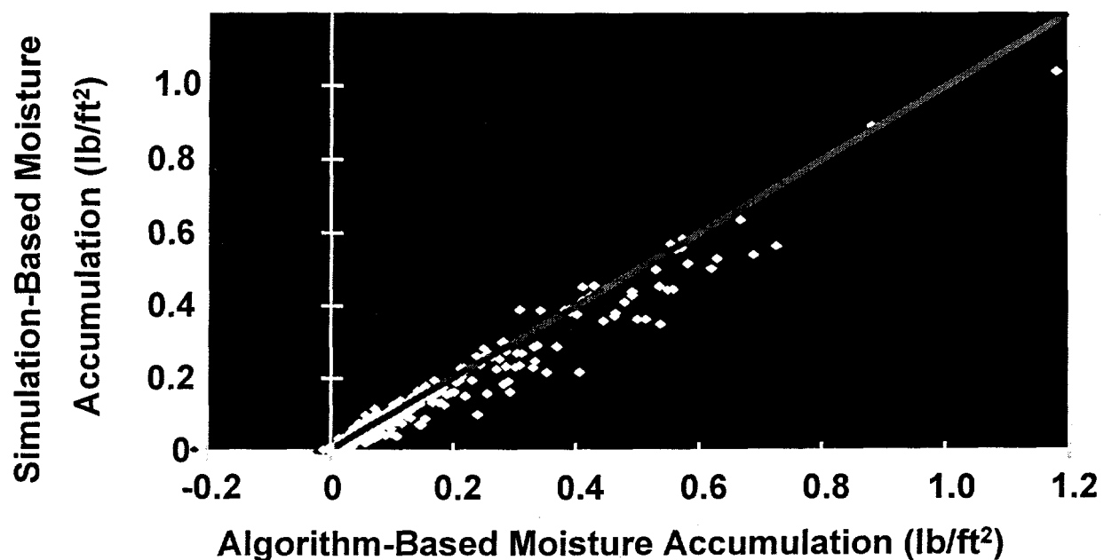
Figure 1 Comparison of the Simulation- and Correlation-Based Moisture Accumulation (Desjarlais and Byars, 1997b)
