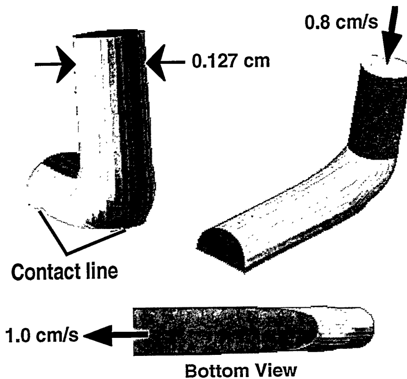
Figure 2: Three-dimensional modelling of bead flow. Three views of the same Newtonian bead laydown solution. The fluid enters the cylindrical nozzle at 0.8 cm/s and the web is moving at 1.0 cm/s.
