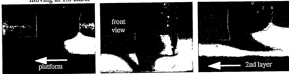
Figure 3: Images of an alumina slurry being deposited onto a moving platform (left and center) and the slurry being deposited onto a previously deposited alumina bead (right).
