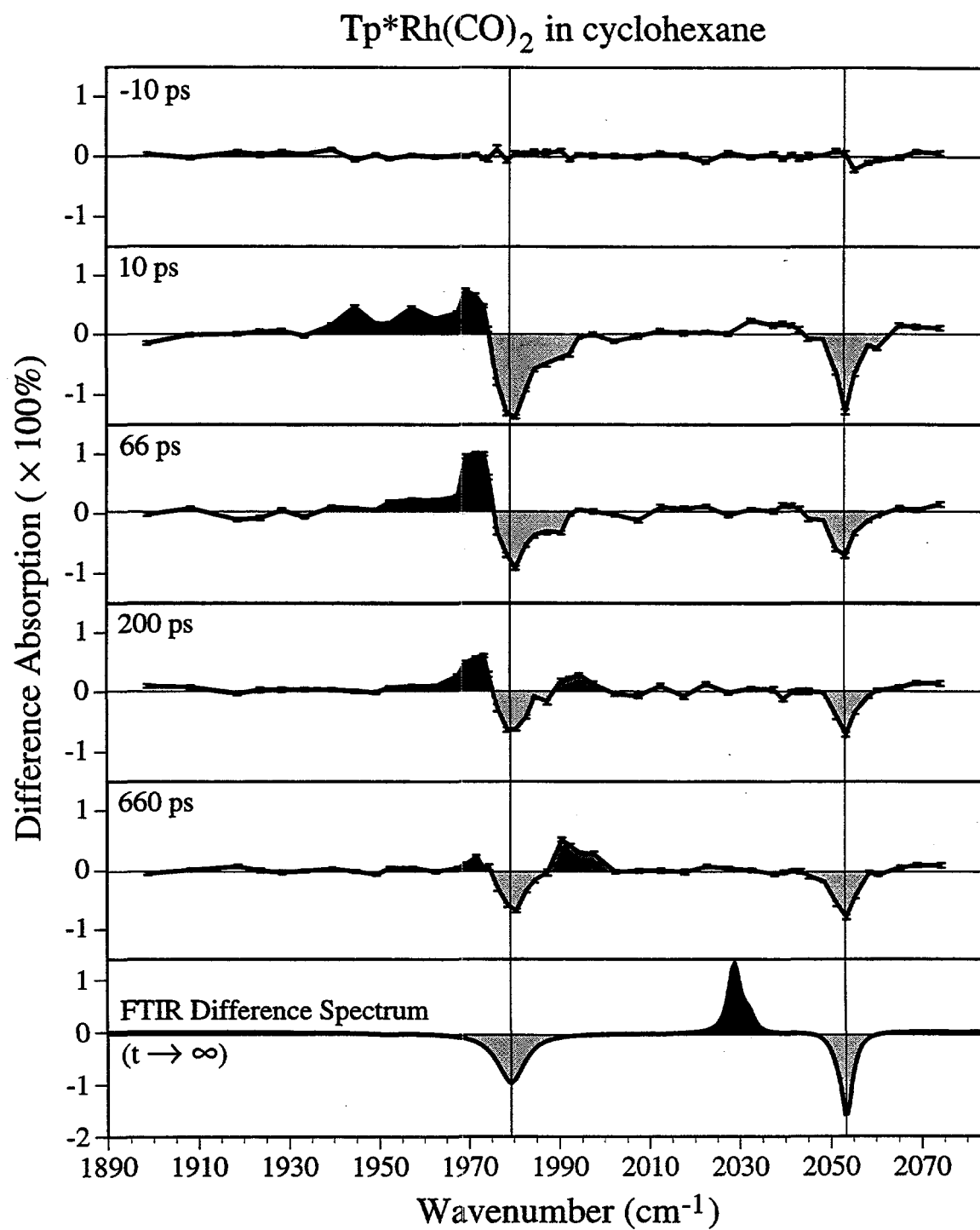
Figure 4.20: Femtosecond spectra of \text{Tp}^*\text{Rh}(\text{CO})_2 in cyclohexane.
