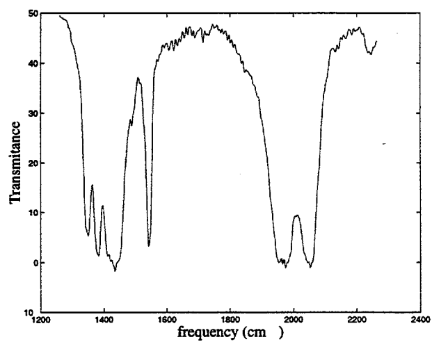
(a) \text{Tp}^*\text{Rh}(\text{CO})_2
