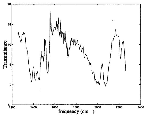
(b) \text{Bp}^*\text{Rh}(\text{CO})_2
