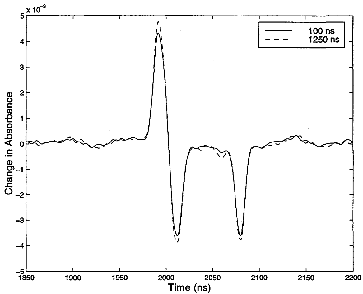
Figure 4.18: Transient nanosecond spectra of Bp*Rh(CO)(H)(phenyl) complex in benzene
