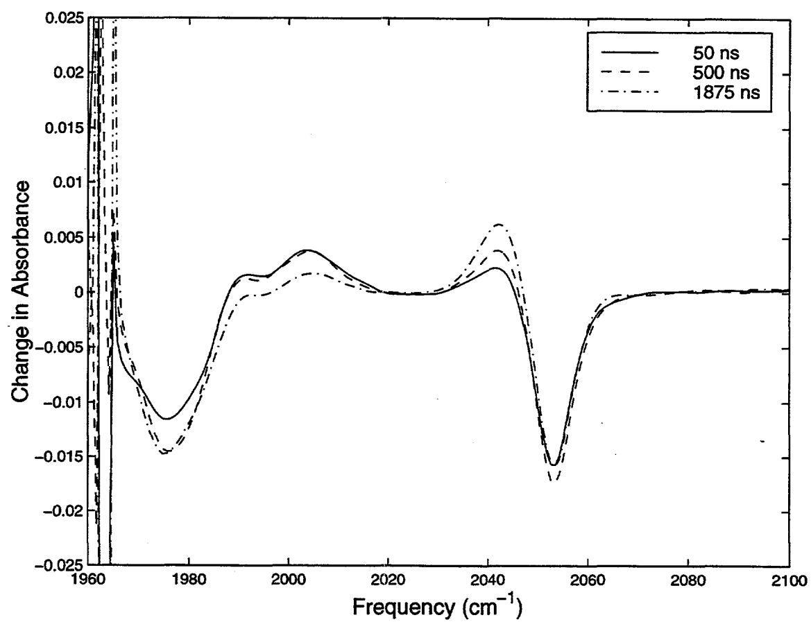
Figure 4.24: Nanosecond Spectra for C-H activation by Tp * Rh(CO) 2 in toluene
