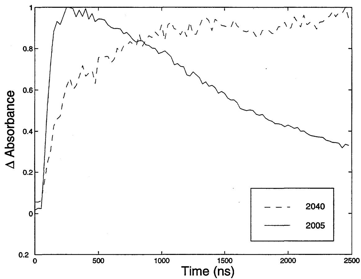
Figure 4.23: Kinetics of \text{Tp}^*\text{Rh}(\text{CO})_2 in \text{d}_6 -benzene
