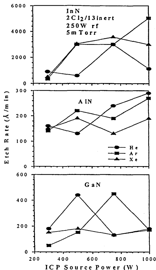
Figure 4. Effect of ICP source power on etch rates of InN (top), AlN (center) and GaN (bottom) with 2Cl 2 /13He, 2Cl 2 /13Ar and 2Cl 2 /13Xe plasma chemistries (250W rf chuck power, 5mTorr).
