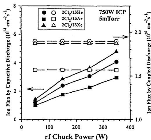
Figure 3. Effect of rf chuck power on the ion fluxes generated by capacitive discharge and inductively coupled discharge with 2\text{Cl}_2/13\text{He} , 2\text{Cl}_2/13\text{Ar} and 2\text{Cl}_2/13\text{Xe} plasma chemistries (750W source power, 5mTorr).
