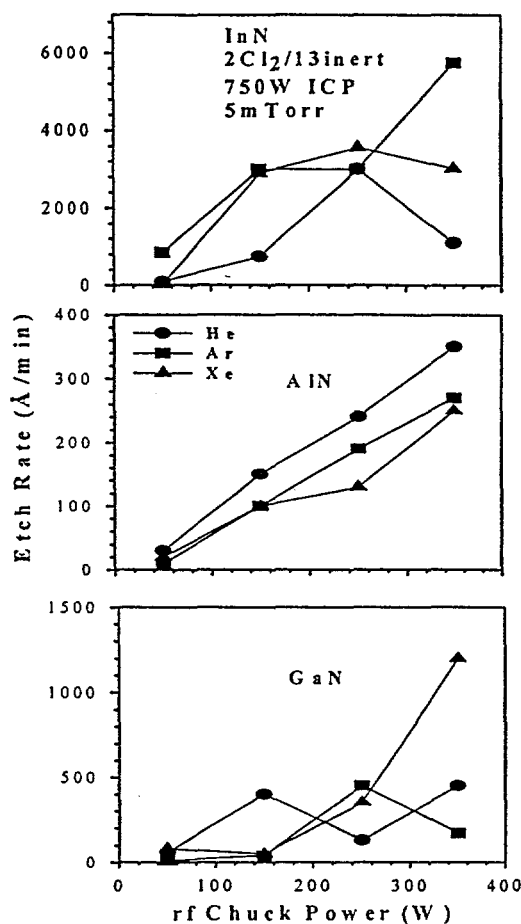
Figure 2. Effect of rf chuck power on etch rates of InN (top), AlN (center) and GaN (bottom) with 2Cl 2 /13He, 2Cl 2 /13Ar and 2Cl 2 /13Xe plasma chemistries (750W source power, 5mTorr).
