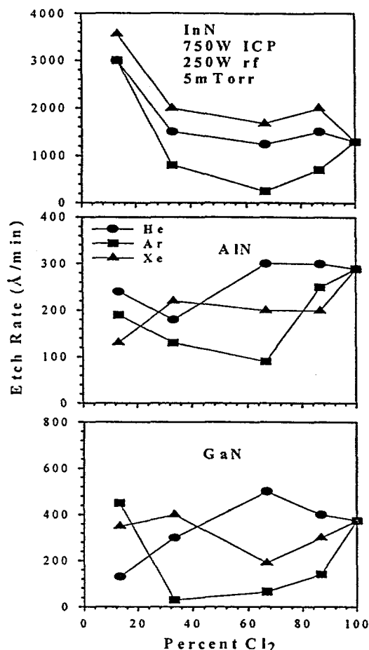
Figure 1. Effect of chlorine concentration on etch rates of InN (top), AlN (center) and GaN (bottom) with Cl 2 /He, Cl 2 /Ar and Cl 2 /Xe plasma chemistries (750W source power, 250W rf chuck power, 5mTorr).
