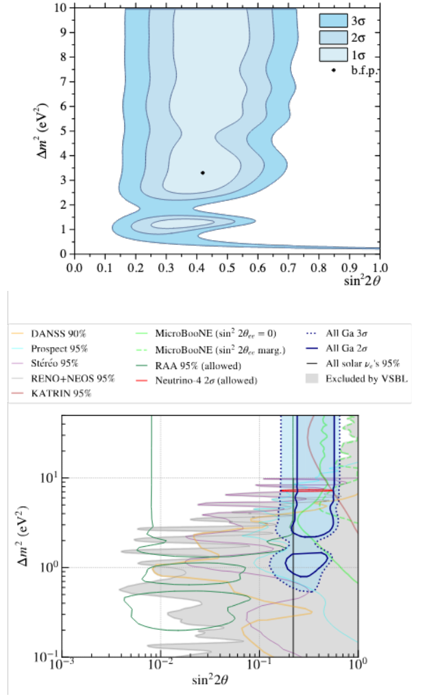
FIG. 3. Top: Exclusion for the results from BEST. The best fit point (b.f.p.) is for m^2 = 3.3 \text{ eV}^2 and \sin^2 2\theta = 0.42 . Bottom: Exclusion contours of all Ga anomaly experiments: two GALLEX, two SAGE and two BEST results. The blue solid line and the blue dotted line shows the 2\sigma and 3\sigma confidence level respectively. The figure also presents the exclusion contours from Prospect [38], DANSS [39], Stéréo [40], KATRIN [41], the combined analysis of RENO and NEOS data [42], reactor anti-neutrino anomalies (RAA) [43] allowed region, interpretations of the MicroBooNE result for the oscillation hypothesis with fixed mixing angle ( \sin^2 2\theta ) and profiled over the angle [44], and the model-independent 95% upper bound on \sin^2 2\theta from all solar neutrino experiments [45]. The 2\sigma allowed region of Neutrino-4 [46] is also presented and the grey shading represents the merged exclusion of the very short baseline (VSBL) null results.
