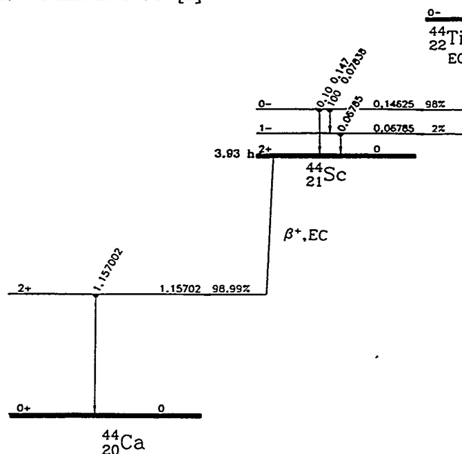
Figure 1. Relevant portions of the decay schemes of ^{44}\text{Ti} and ^{44}\text{Sc} [2]. All energies are in MeV.
