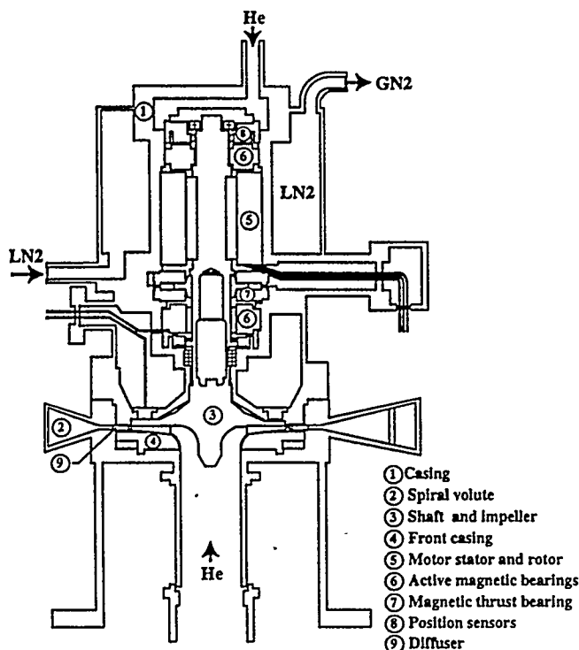
Figure 4. Cold Compressor
