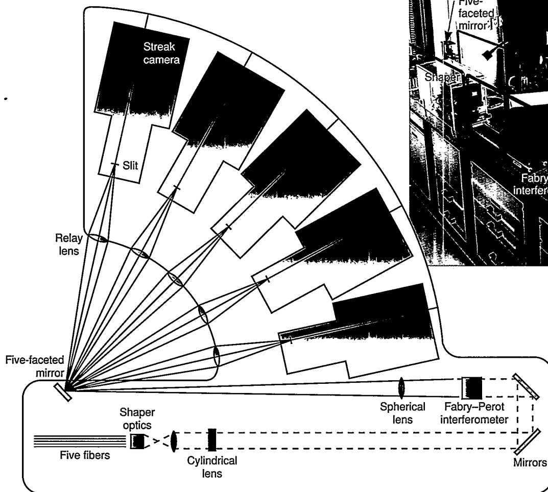
Figure 1. Photo of five-beam system (with a second five-beam array in the background) and a schematic of the system.
