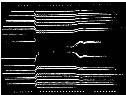
Figure 6. (a) An example of a streak camera record from an earlier version of our dual-cavity Fabry-Perot interferometer. (b) An example of data analysis using three different estimates of the "jump" in the dot pattern when rapid acceleration occurs. Without the second set of fringes, the scientists would not know which is correct. The overlap of the center two curves shows it to be the correctly estimated velocity.
