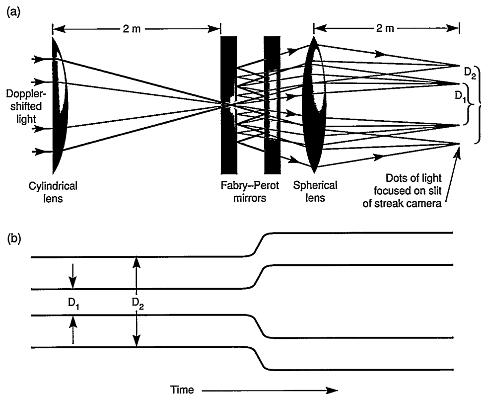
Figure 2. (a) A top view of the Fabry-Perot velocimeter system from the cylindrical lens to the slit in the streak camera. The interference pattern of bright dots— D_1 and D_2 —is recorded on the streak camera. (b) A hypothetical streak camera record shows what happens to D_1 and D_2 when acceleration occurs. Velocities are determined using a formula based on measurements of the separation between the dots.
