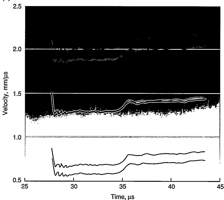
Figure 6. (a) An example of a streak camera record from an earlier version of our dual-cavity Fabry-Perot interferometer. (b) An example of data analysis using three different estimates of the "jump" in the dot pattern when rapid acceleration occurs. Without the second set of fringes, the scientists would not know which is correct. The overlap of the center two curves shows it to be the correctly estimated velocity.
