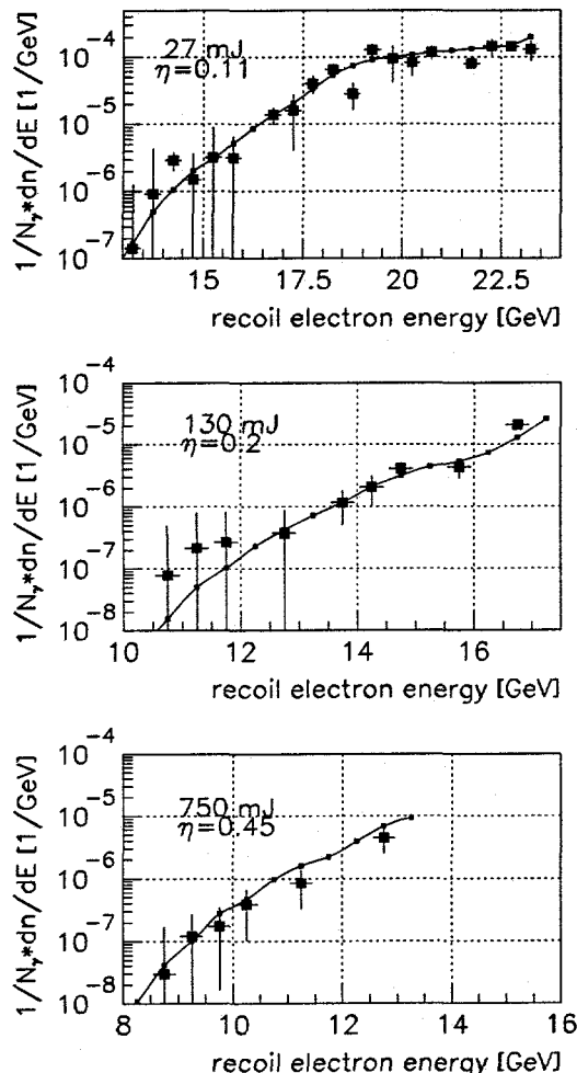
FIG. 10. Energy spectra of scattered electrons as observed in the ECAL calorimeter for 3 of 12 laser intensities. The data are normalized to the total Compton-scattered photon rate measured in the CCM1 detector. The curves are from a simulation of the experiment.
