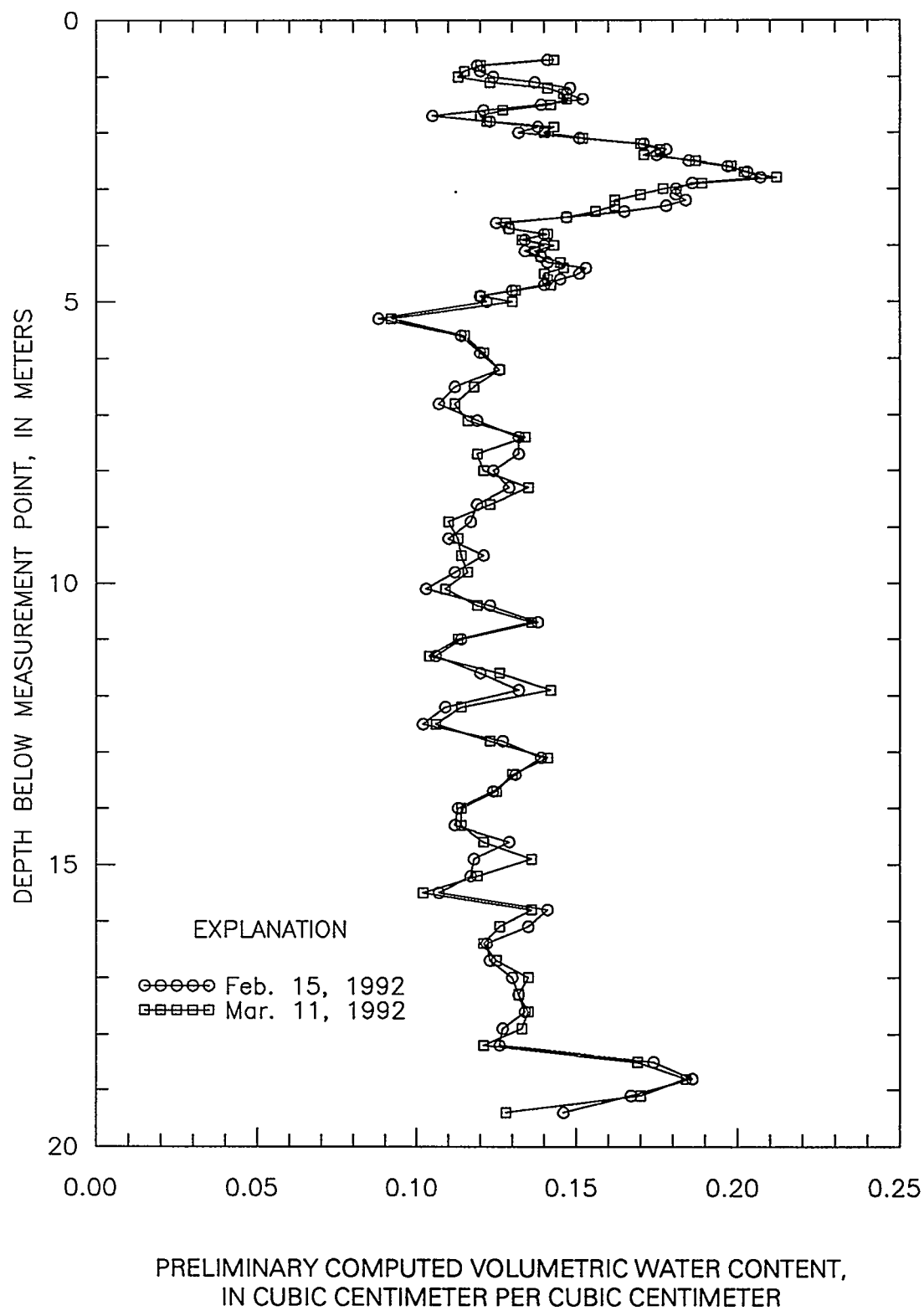
Figure 13. Preliminary computed volumetric water-content profiles for UE-29 UZN #92 for Feb. 15, 1992 and Mar. 11, 1992.
