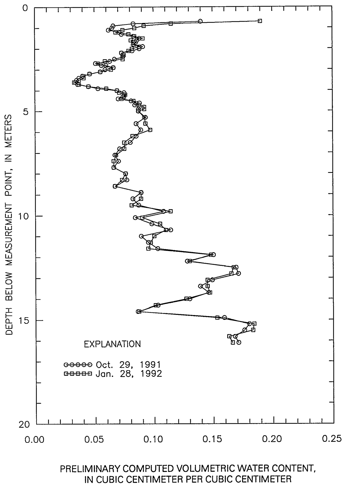
Figure 6. Preliminary computed volumetric water-content profiles for UE-29 UZN #91 for Oct. 29, 1991 and Jan. 28, 1992.
