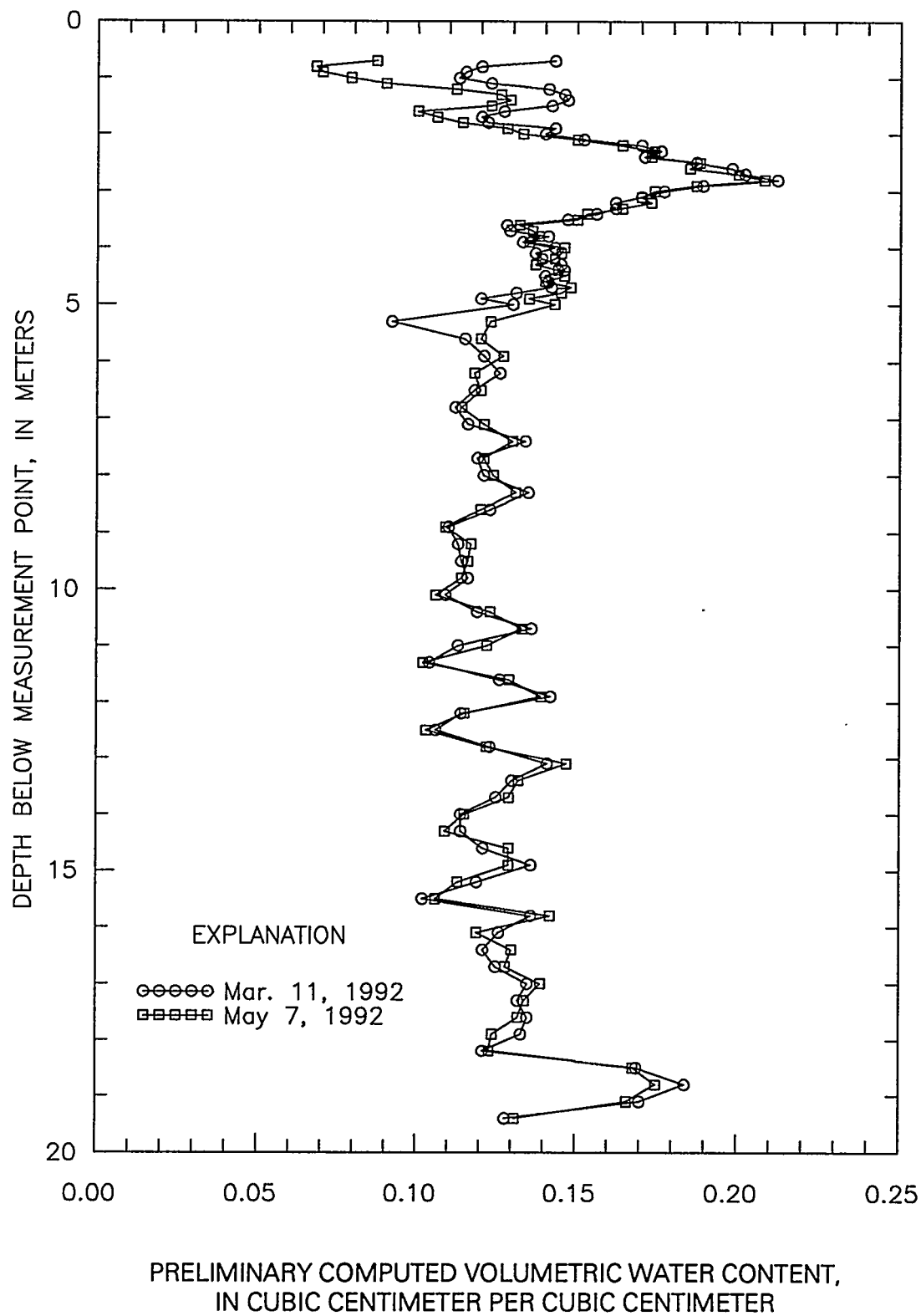
Figure 14. Preliminary computed volumetric water-content profiles for UE-29 UZN #92 for Mar. 11, 1992 and May 7, 1992.
