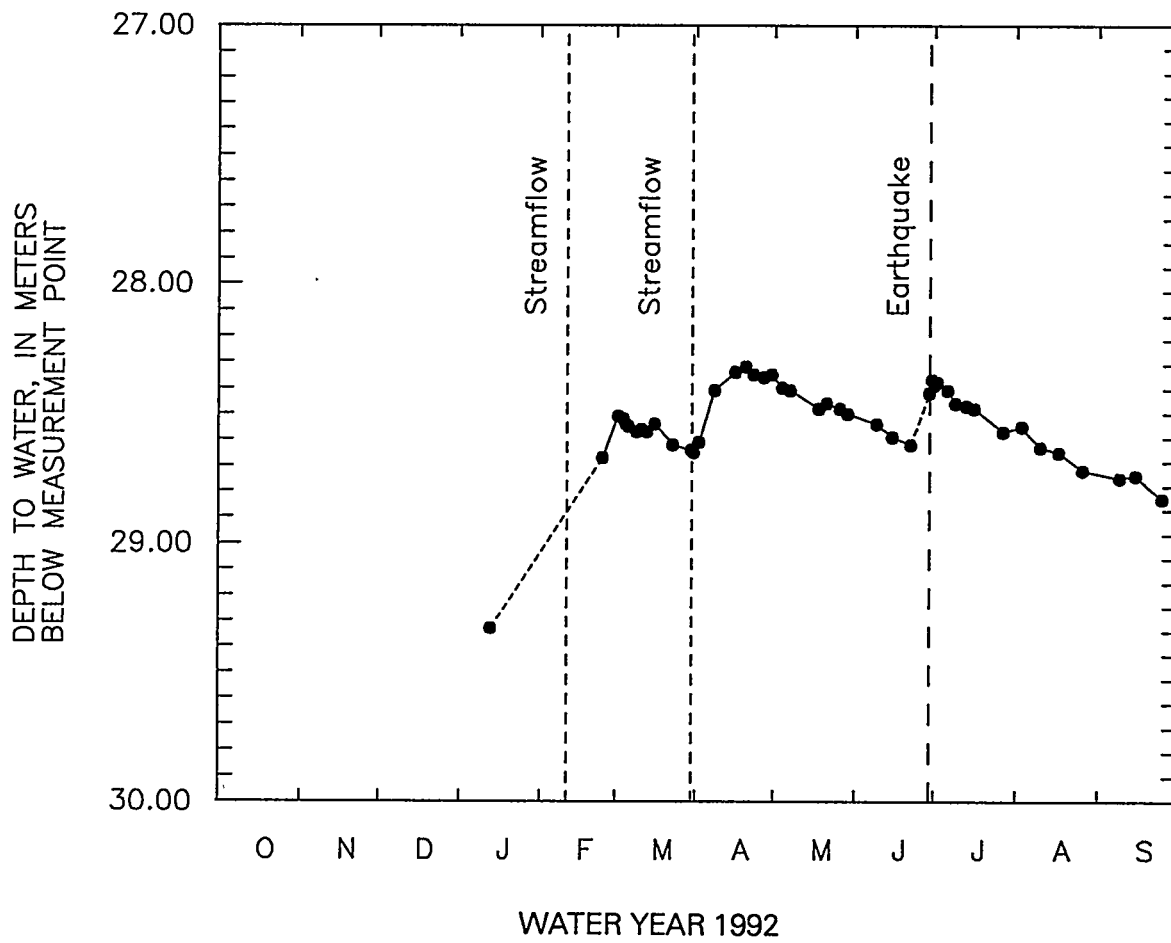
Figure 17. Depth-to-water measurements in UE-29 a#2.
