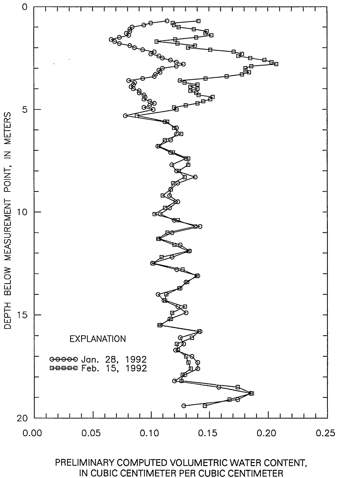
Figure 12. Preliminary computed volumetric water-content profiles for UE-29 UZN #92 for Jan. 28, 1992 and Feb. 15, 1992.
