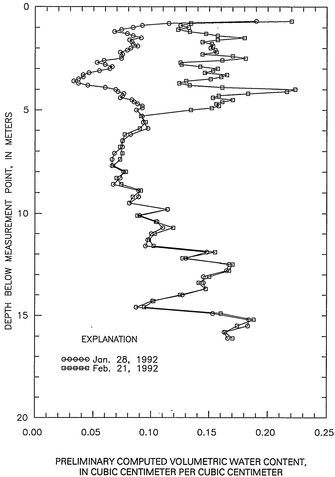
Figure 7. Preliminary computed volumetric water-content profiles for UE-29 UZN #91 for Jan. 28, 1992 and Feb. 21, 1992.
