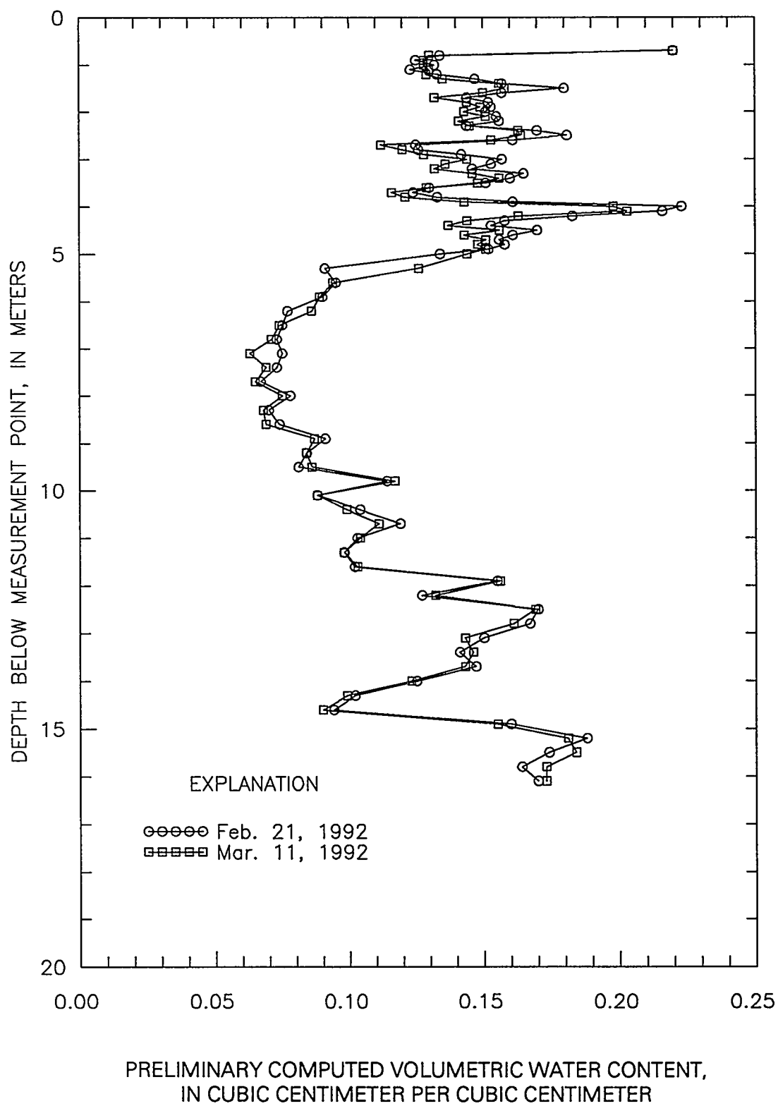
Figure 8. Preliminary computed volumetric water-content profiles for UE-29 UZN #91 for Feb. 21, 1992 and Mar. 11, 1992.
