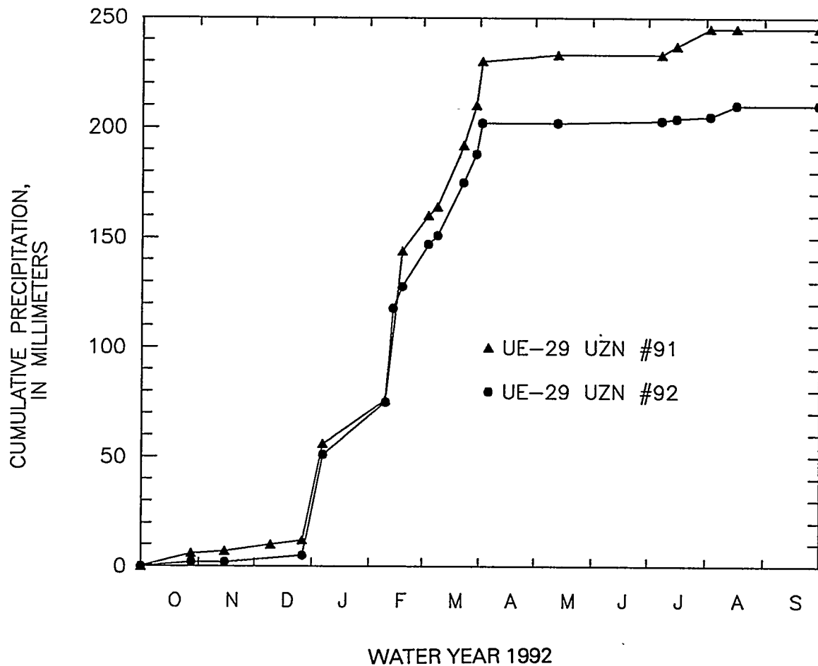
Figure 2. Cumulative precipitation at UE-29 UZN #91 and UE-29 UZN #92.
