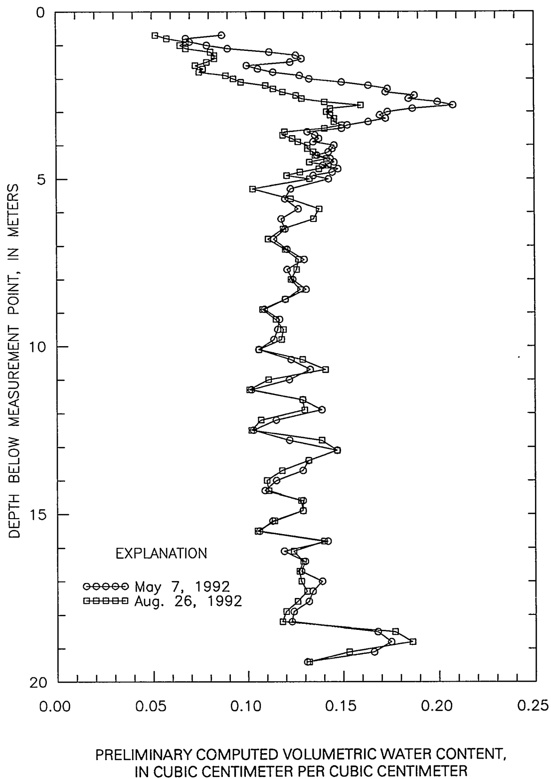
Figure 15. Preliminary computed volumetric water-content profiles for UE-29 UZN #92 for May 7, 1992 and Aug. 26, 1992.
