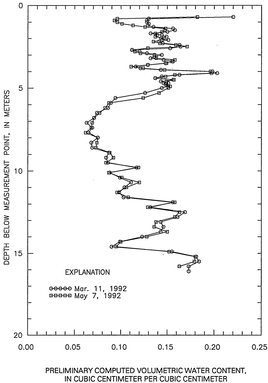
Figure 9. Preliminary computed volumetric water-content profiles for UE-29 UZN #91 for Mar. 11, 1992 and May 7, 1992.
