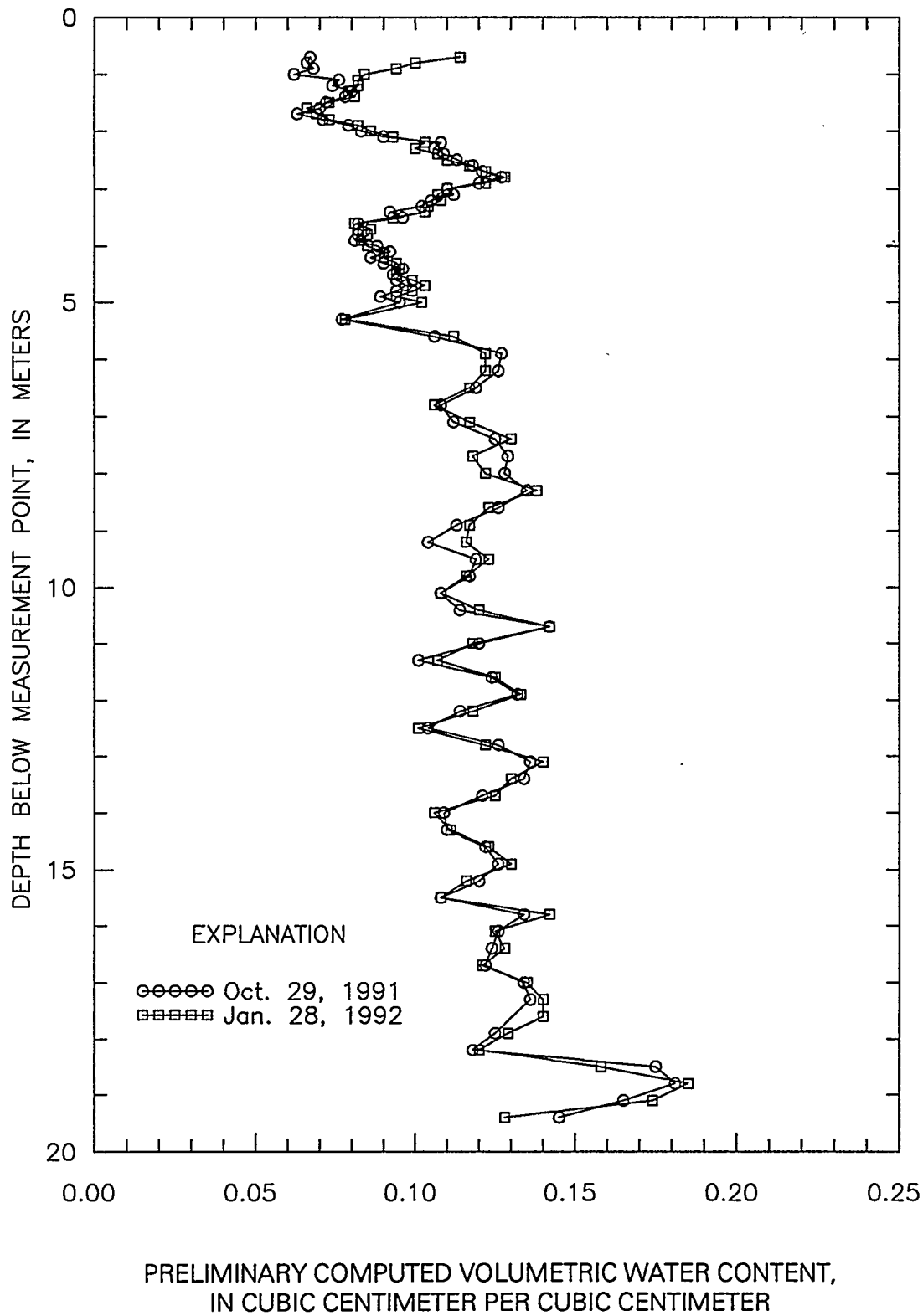
Figure 11. Preliminary computed volumetric water-content profiles for UE-29 UZN #92 for Oct. 29, 1991 and Jan. 28, 1992.
