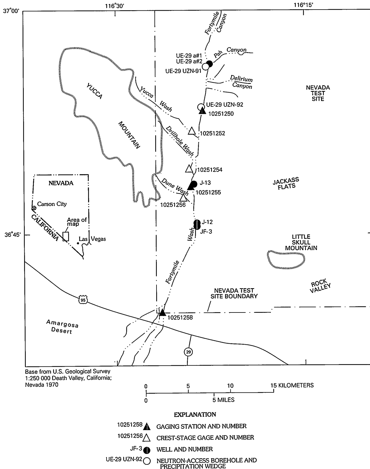
Figure 1. Location of gaging stations, crest-stage gages, neutron-access boreholes, and wells.
