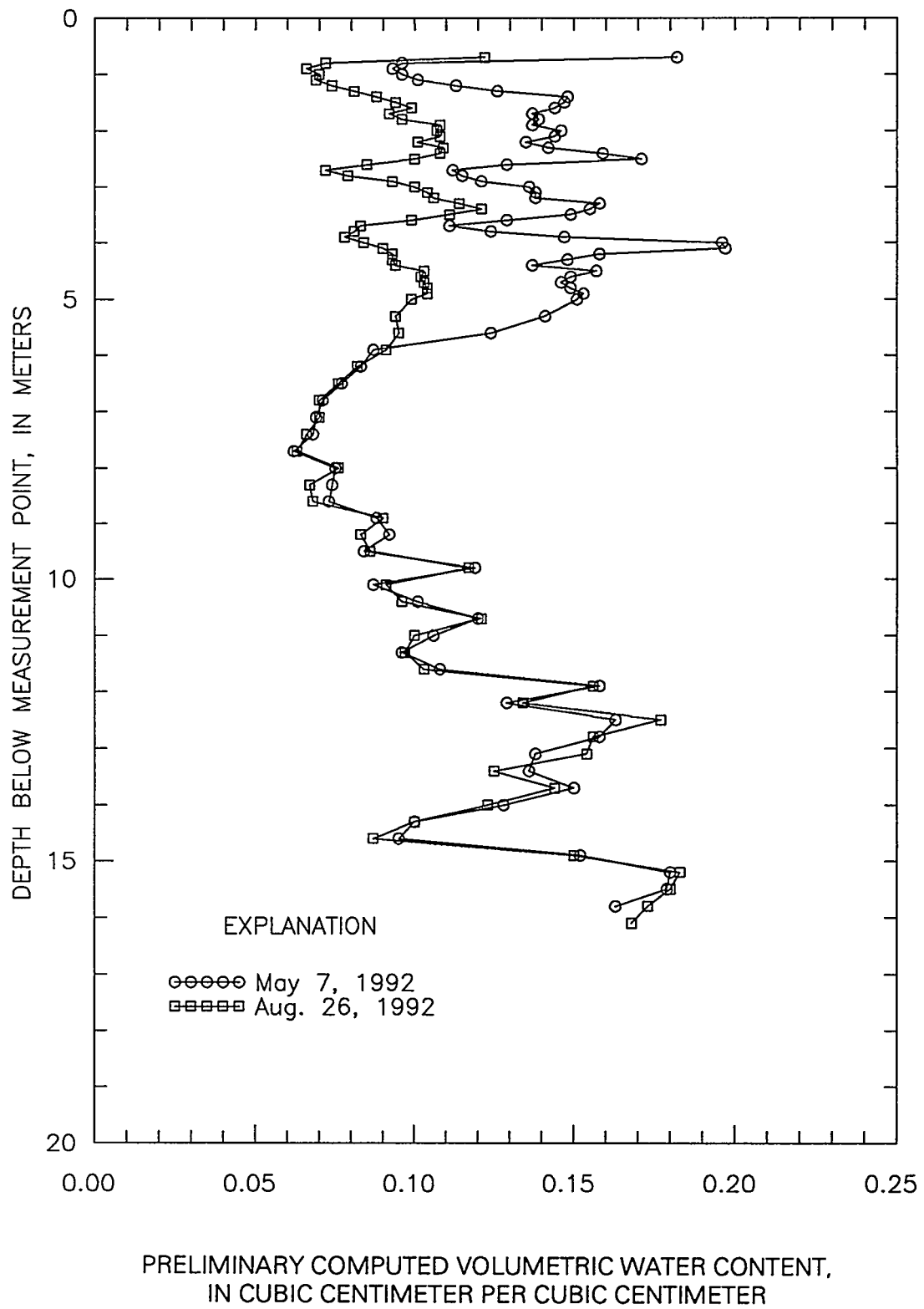
Figure 10. Preliminary computed volumetric water-content profiles for UE-29 UZN #91 for May 7, 1992 and Aug. 26, 1992.
