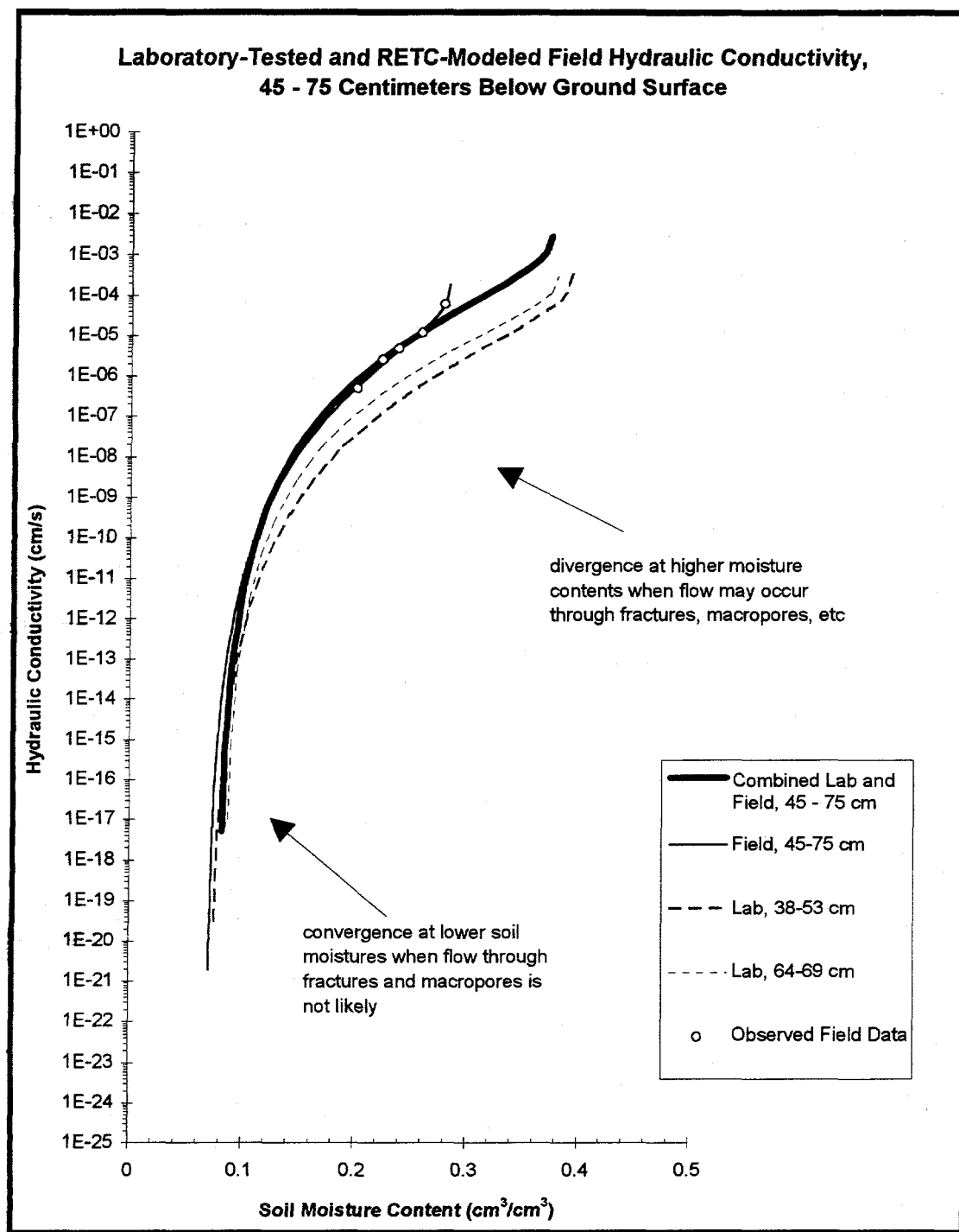
Figure 4. RETC-predicted hydraulic conductivity-moisture content relationships based on field, laboratory, and combined field and laboratory data. Lower hydraulic conductivity values from laboratory testing are observed at higher moisture contents. The divergence at higher moisture contents and the convergence at lower moisture contents suggests that preferential flow through soil structure (macropores and fractures) may occur if moisture contents approach saturation.
