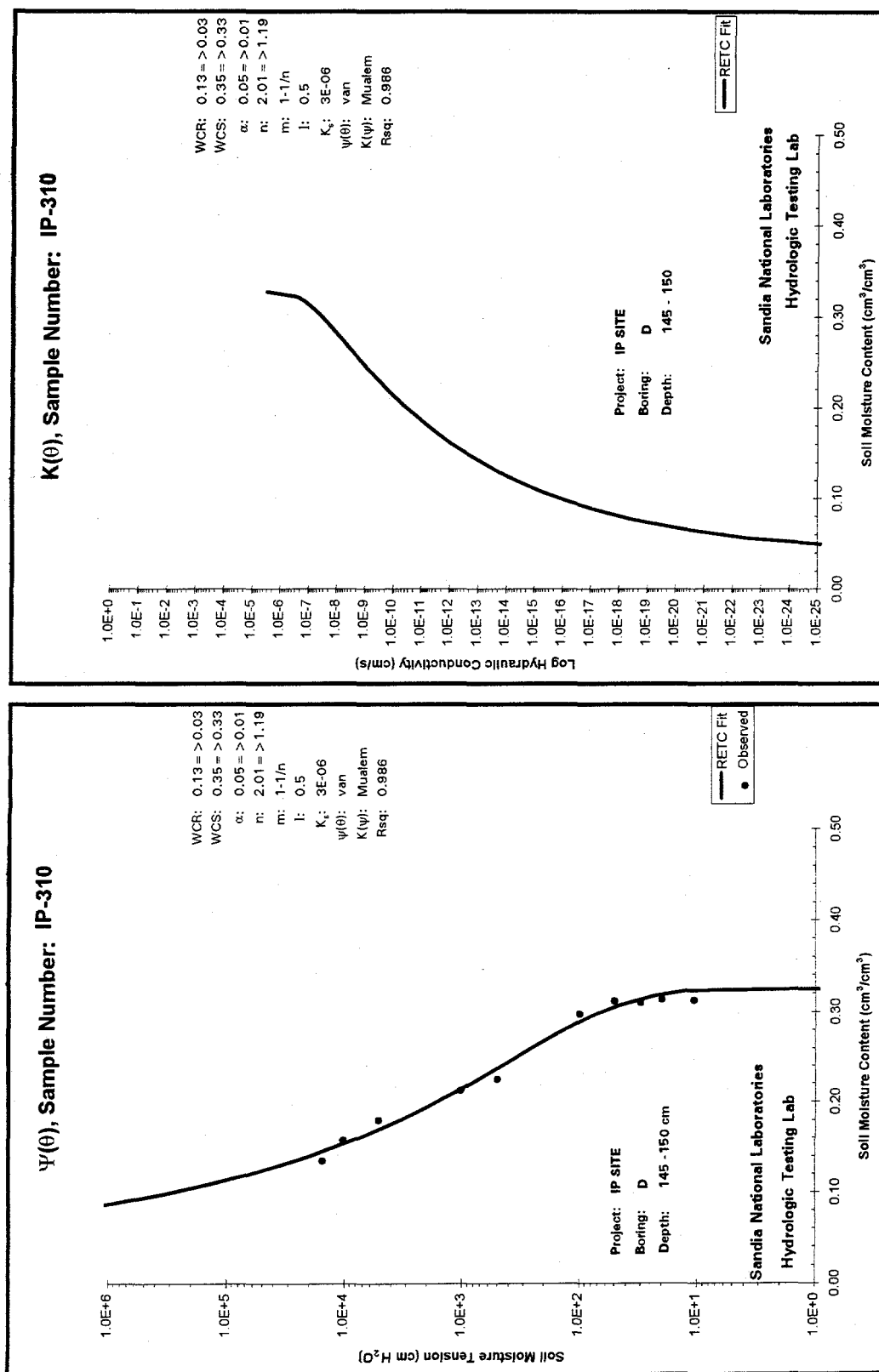
Figure A-11. RETC simulations of \psi(\theta) and K(\theta) relationships for the laboratory-tested sample from 145 - 150 cm bgs.
