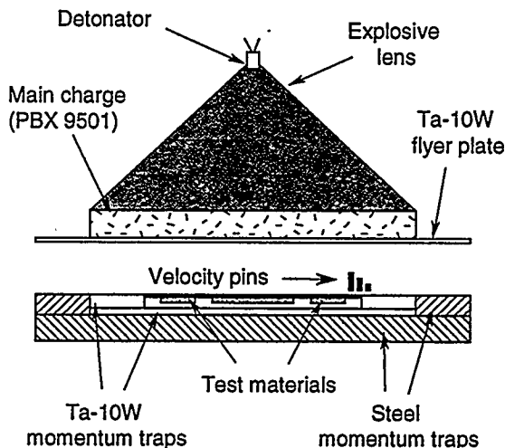
Figure 1: Schematic of the shock assembly.
