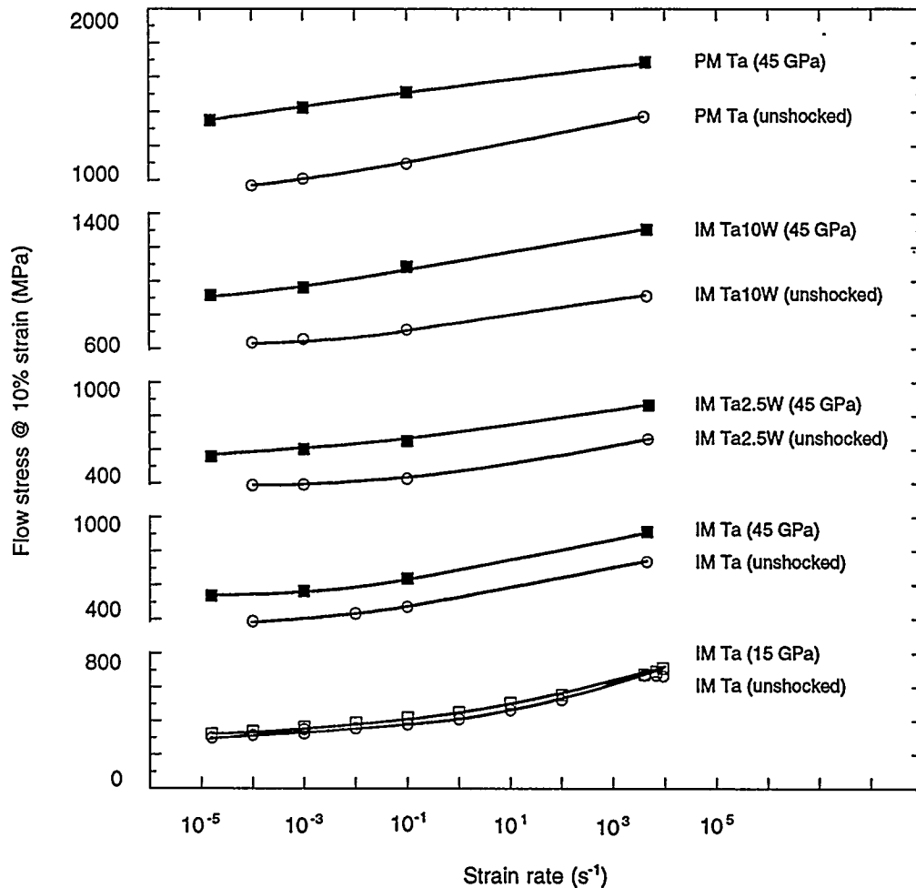
Figure 5: Plot of the strain rate sensitivities of the shocked and unshocked materials.
