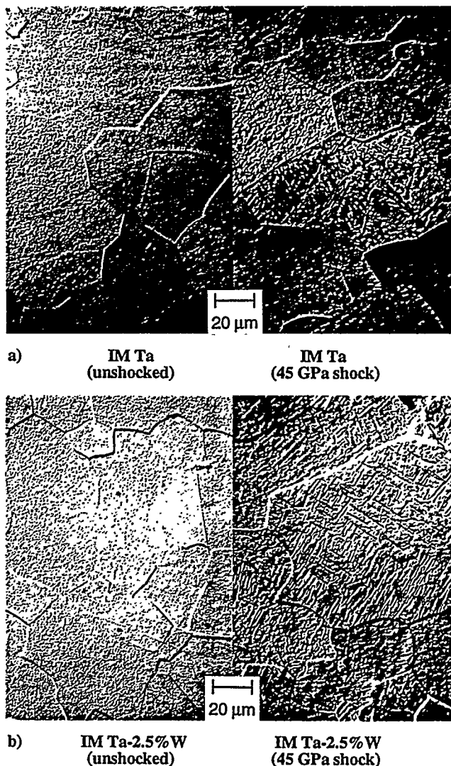
Figure 2: Micrographs of the test materials in the annealed and post-shock conditions.
