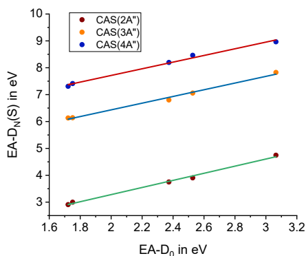
Fig. 9 (a) Correlation plot between EA-D_N(S) and EA-D_0 at the EOM-EA-CCSD level. Linear regression gives: y = 1.0106x + 4.7116 with R^2 = 0.9848 . (b) Correlation plots between EA of the three resonances 2^2A'' , 3^2A'' , 4^2A'' vs 1^2A'' ( EA-D_0 ) at the CASSCF level. Linear regression gives: 2^2A'' : y = 1.3245x + 0.6306 with R^2 = 0.9948 ; 3^2A'' : y = 1.2473x + 3.9387 with R^2 = 0.9915 ; 4^2A'' : y = 1.2401x + 5.2333 with R^2 = 0.991 . All values are obtained from the orbital stabilization method.
