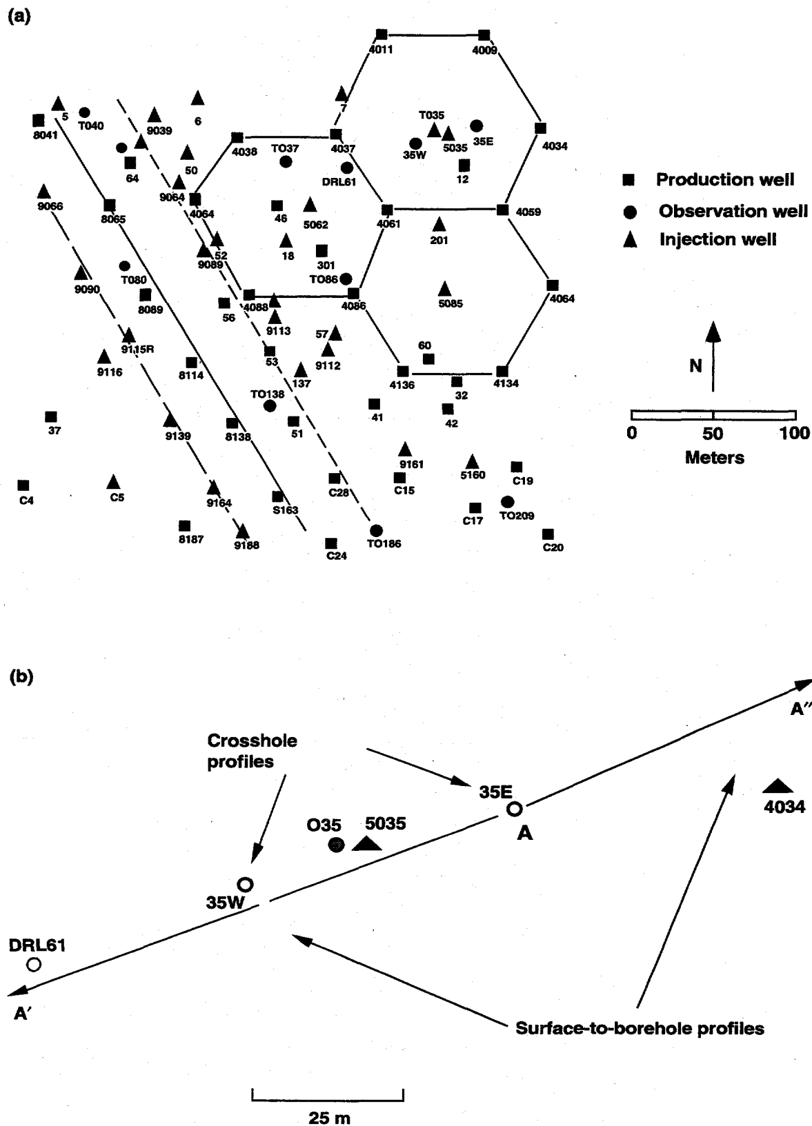
Figure 3. Site map for the EM project at the Lost Hills 3T steamflood.
