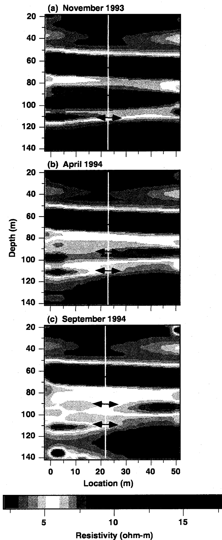
Figure 8. Resistivity images derived from crosshole EM data (a) before steam-flooding, (b) 6 months after flooding, and (c) 10 months after flooding.
