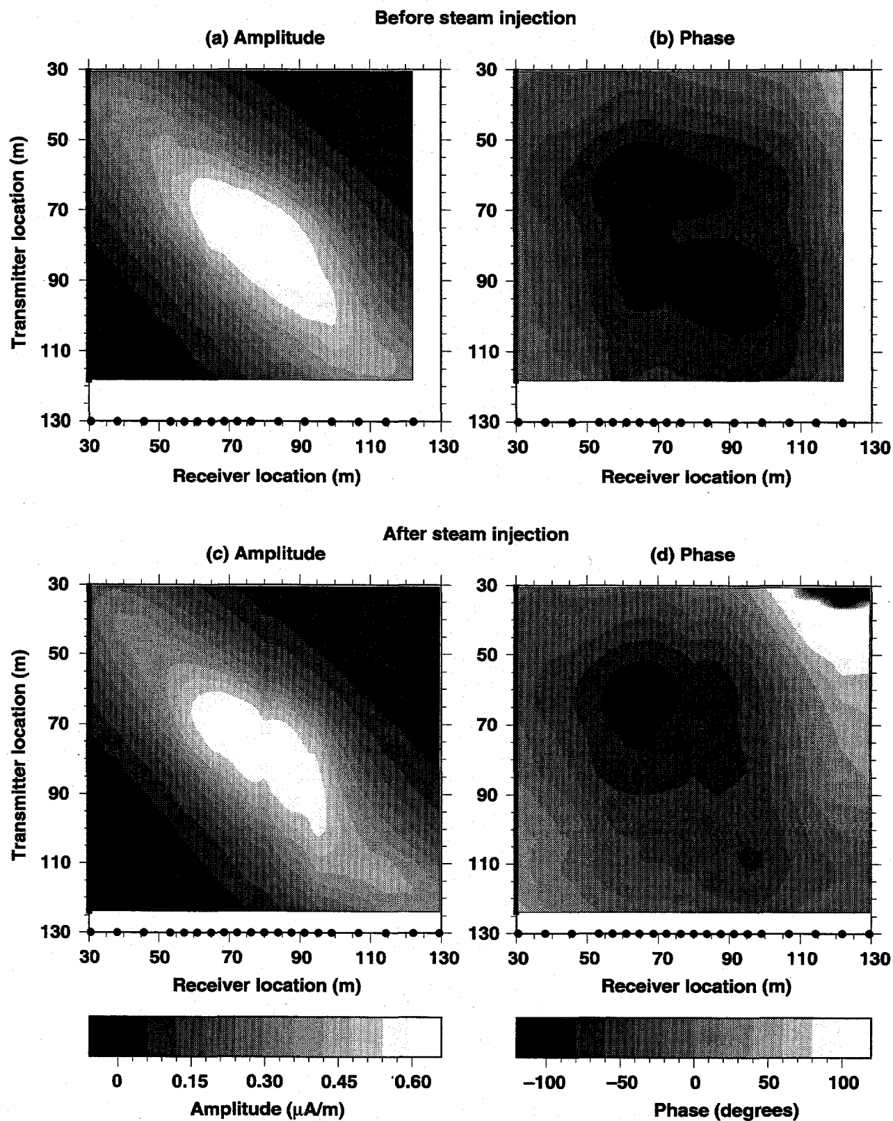
Figure 7. Combined 5-kHz crosshole data set before and six months after steam injection.
