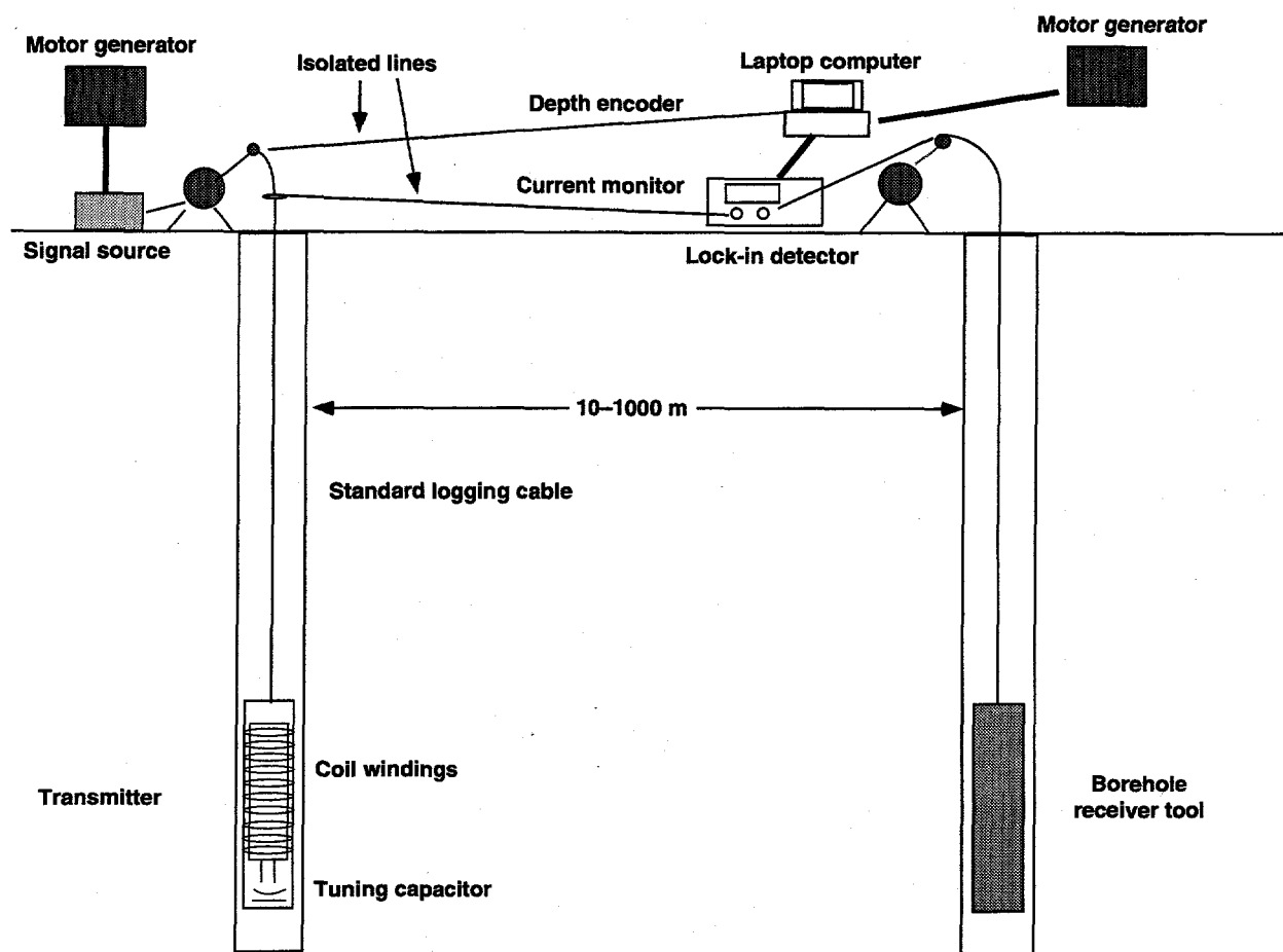
Figure 4. Schematic diagram for the LLNL/LBNL EM system.
