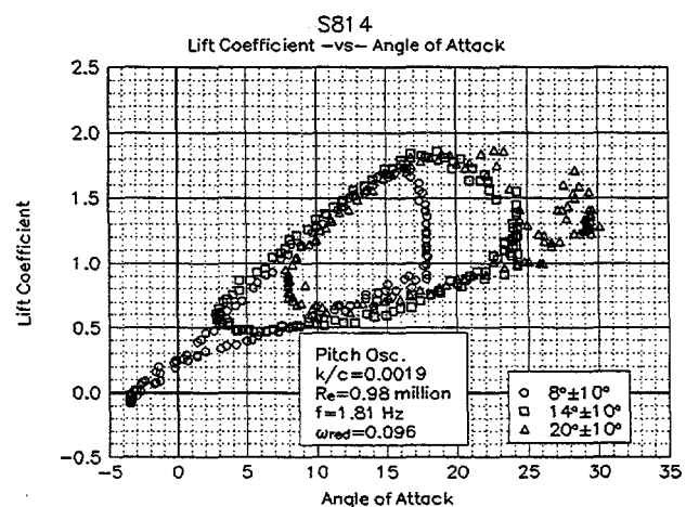
Figure 33. LEGR, C_l vs \alpha , \omega_{red}=0.096 , \pm 10^\circ
