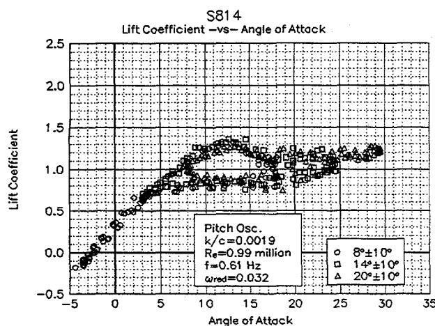
Figure 32. LEGR, C_l vs \alpha , \omega_{red}=0.032 , \pm 10^\circ
