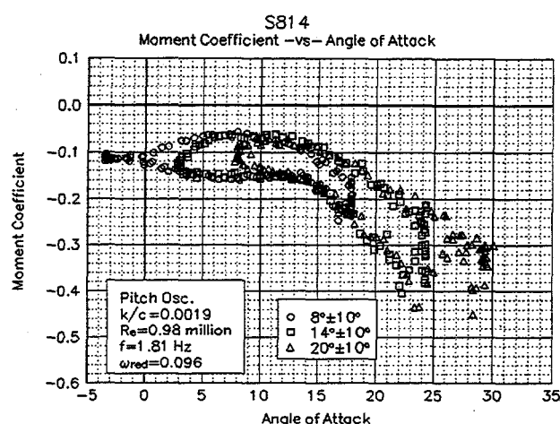
Figure 35. LEGR, C_m vs \alpha , \omega_{red} = 0.096 , \pm 10^\circ
