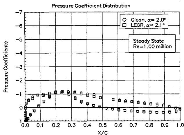
Figure 18. Pressure distribution, \alpha = 2.0^\circ
