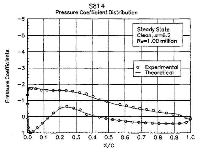
Figure 11. Comparison with theory, C_p vs x/c , \alpha=6.2^\circ
