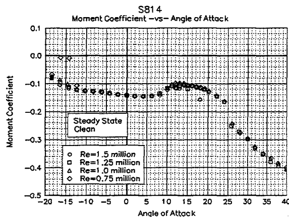
Figure 14. C_m vs \alpha , clean
