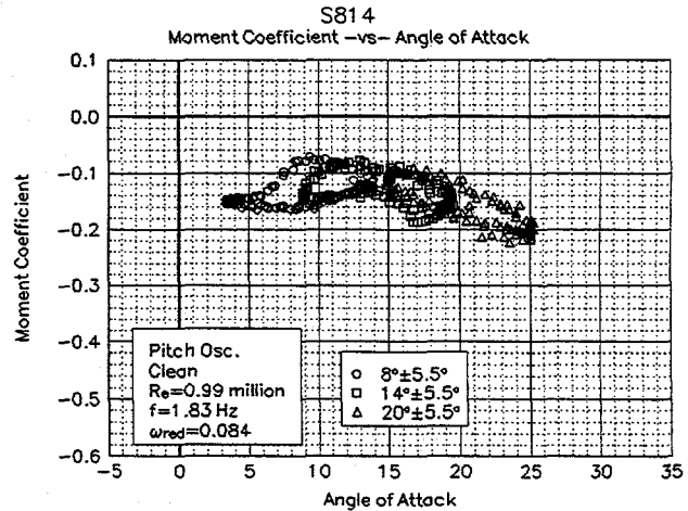
Figure 23. Clean, C_m vs \alpha , \omega_{red}=0.084 , \pm 5.5^\circ
