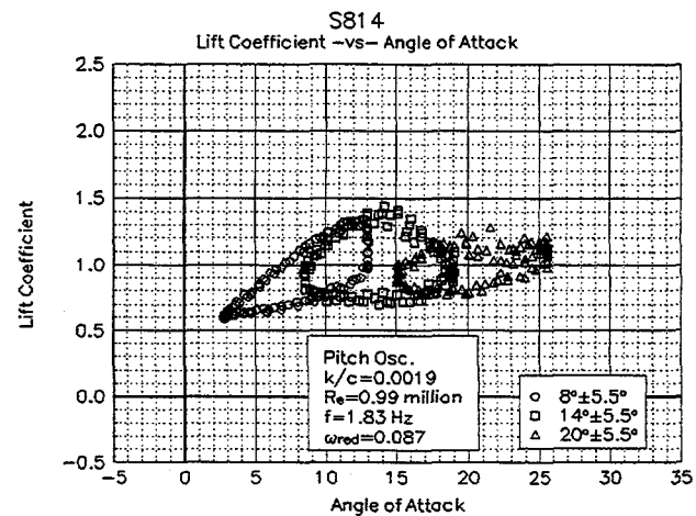
Figure 25. LEGR, C_l vs \alpha , \omega_{red}=0.087 , \pm 5.5^\circ
