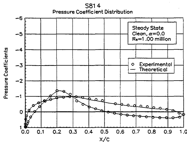
Figure 10. Comparison with theory, C_p vs x/c , \alpha=0.0^\circ
