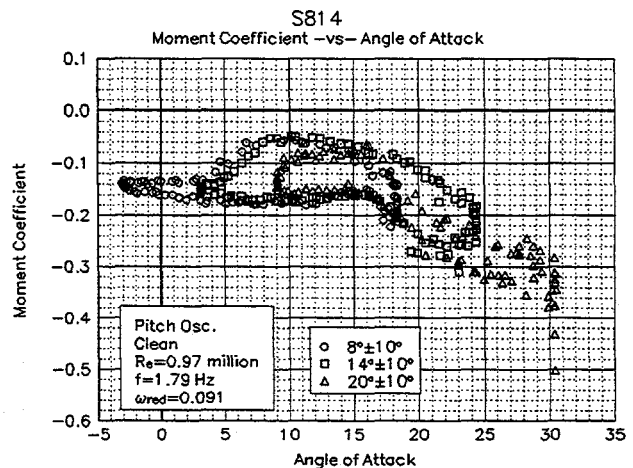
Figure 31. Clean, C_m vs \alpha , \omega_{red}=0.091 , \pm 10^\circ
