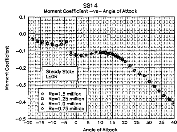
Figure 15. C_m vs \alpha , LEGR, k/c=0.0019
