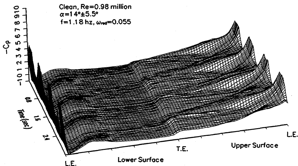
Figure 36. Unsteady pressure distribution, clean, \omega_{red}=0.055 , 14 \pm 5.5^\circ
