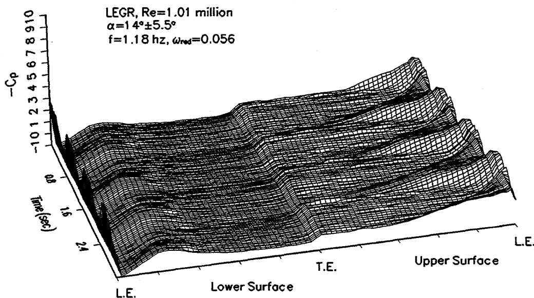
Figure 37. Unsteady pressure distribution, LEGR, \omega_{red}=0.056 , 14 \pm 5.5^\circ
