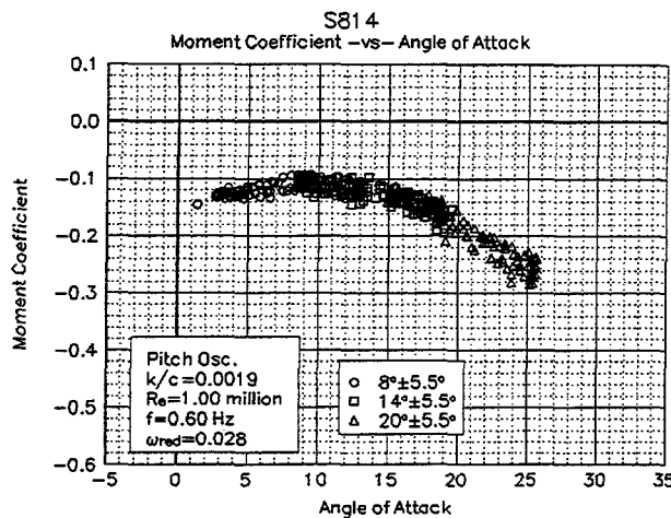
Figure 26. LEGR, C_m vs \alpha , \omega_{red}=0.028 , \pm 5.5^\circ
