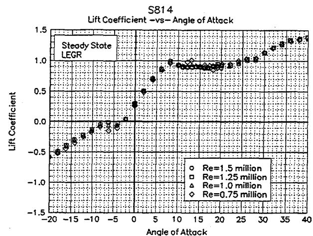
Figure 13. C_l vs \alpha , LEGR, k/c=0.0019
