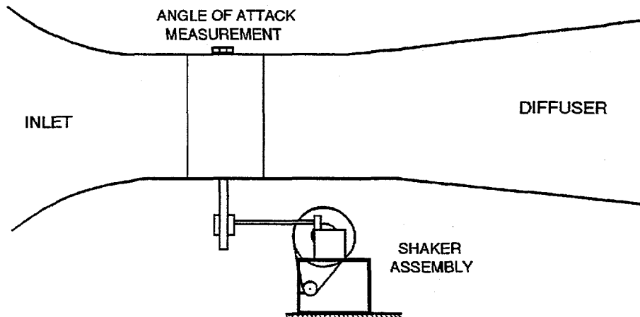
Figure 2. 3×5 Subsonic wind tunnel, side view
