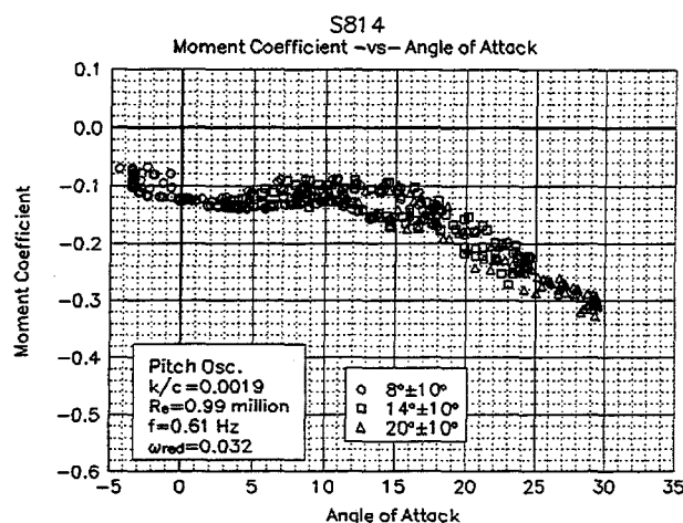
Figure 34. LEGR, C_m vs \alpha , \omega_{red} = 0.032 , \pm 10^\circ
