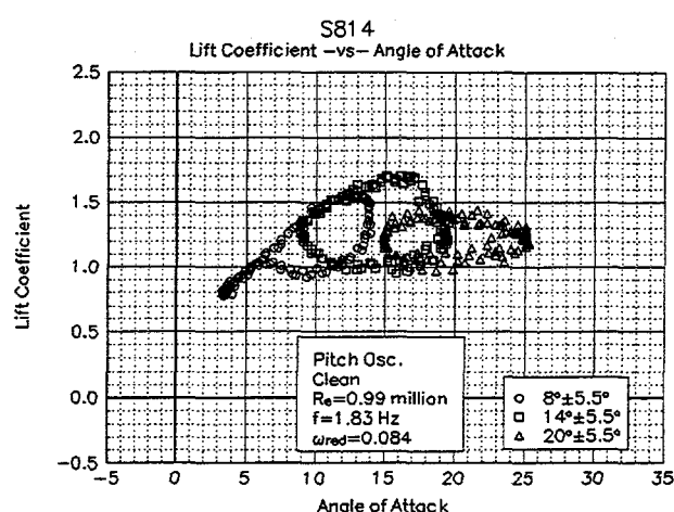
Figure 21. Clean, C_l vs \alpha , \omega_{red}=0.084 , \pm 5.5^\circ
